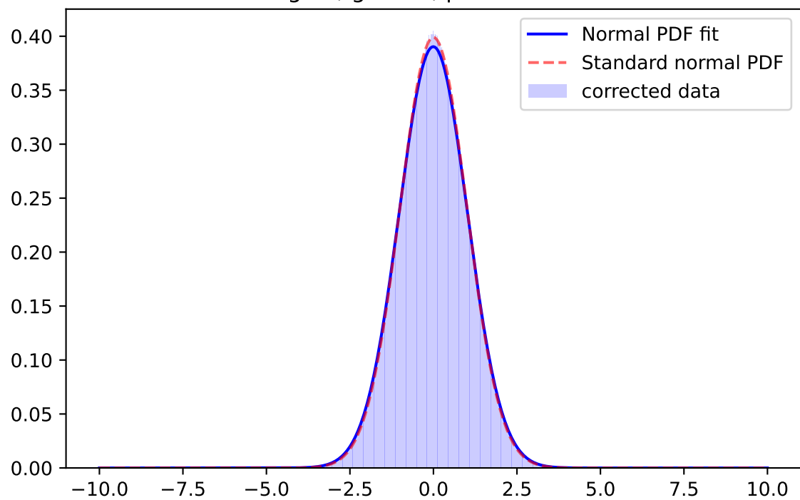
Whiten Signal, i-band, \mu=-0.0002 \sigma=1.0265
