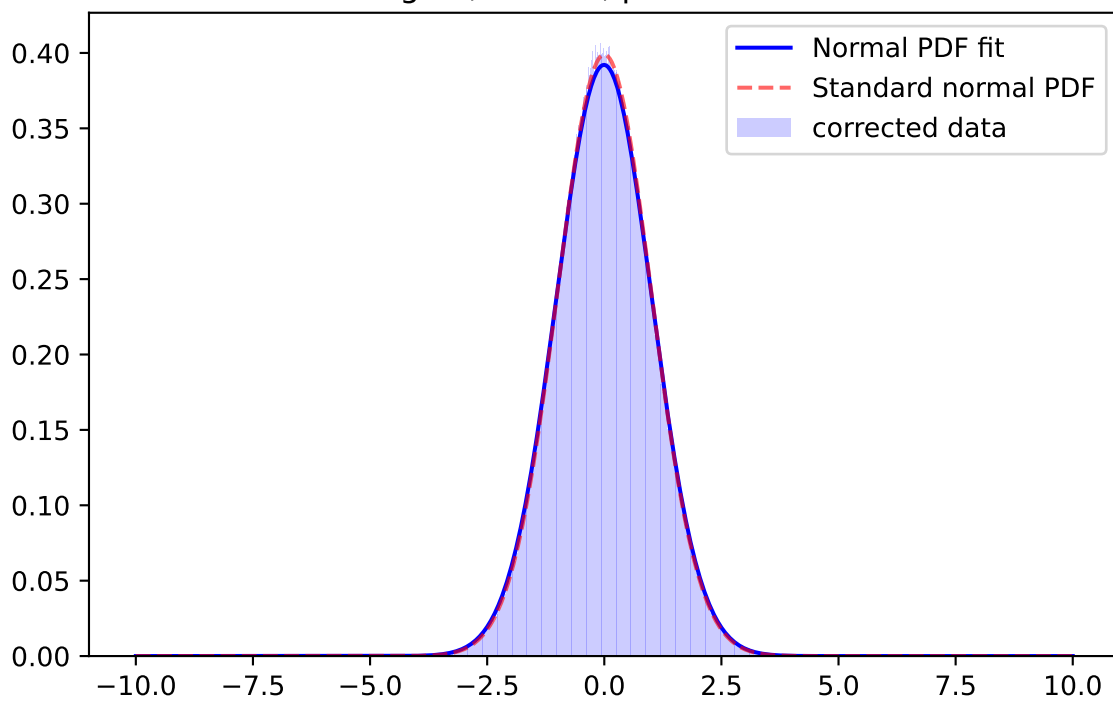
Whiten Signal, r-band, \mu=-0.0026 \sigma=1.0243
