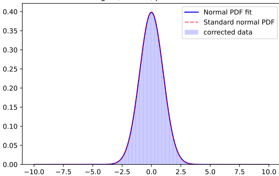
Whiten Signal, z-band, \mu=-0.0065 \sigma=1.0021
