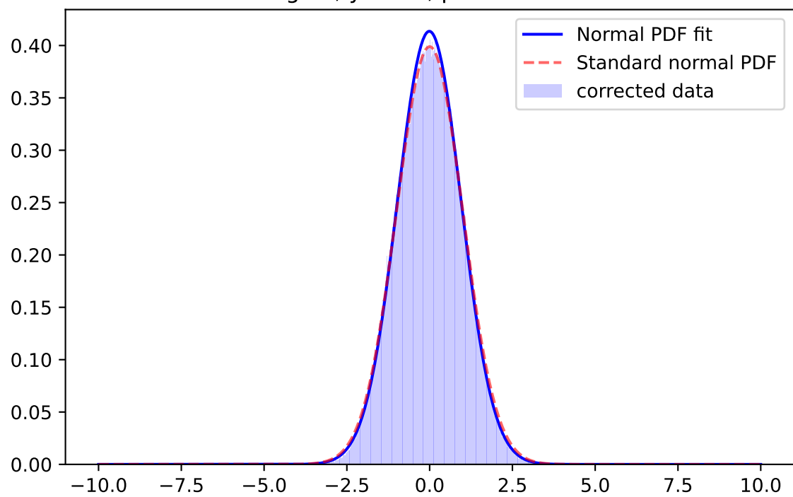
Whiten Signal, y-band, \mu=-0.0097 \sigma=0.9645
