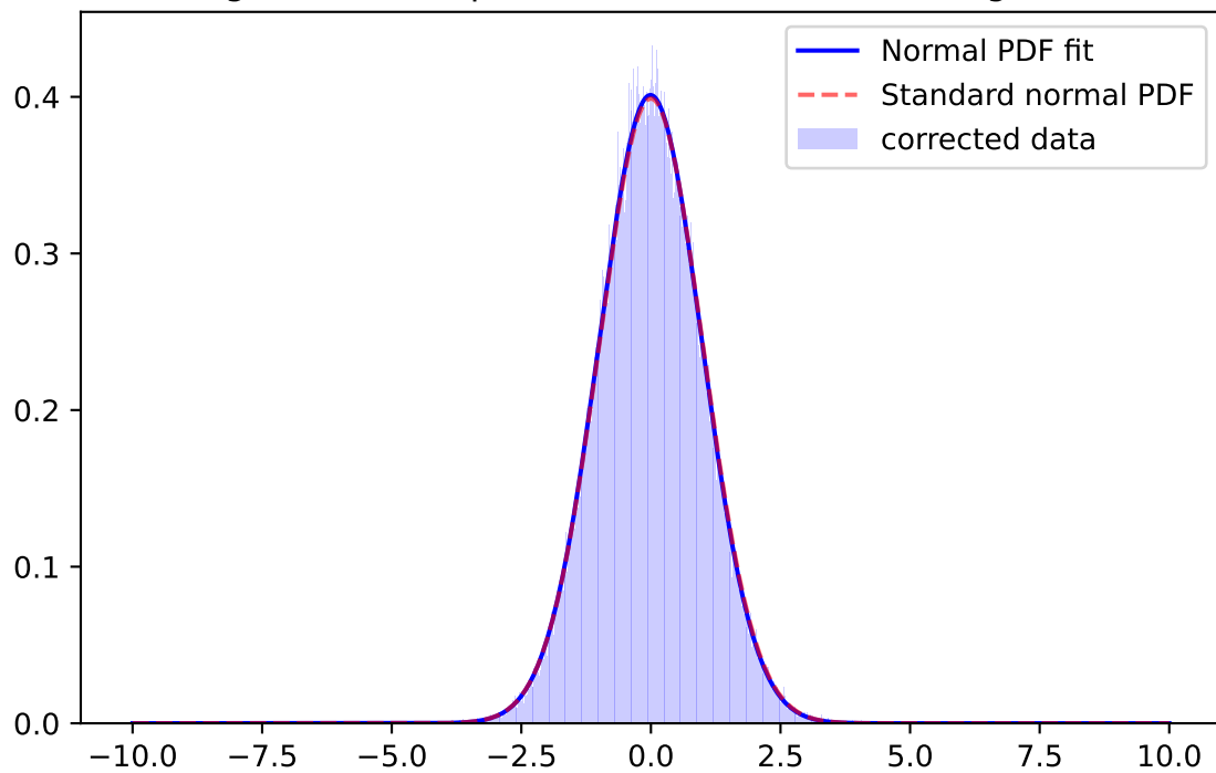
Whiten Signal, r-band, \mu=-0.0056 \sigma=1.0146 ; for mag=[25.0; 25.5]
