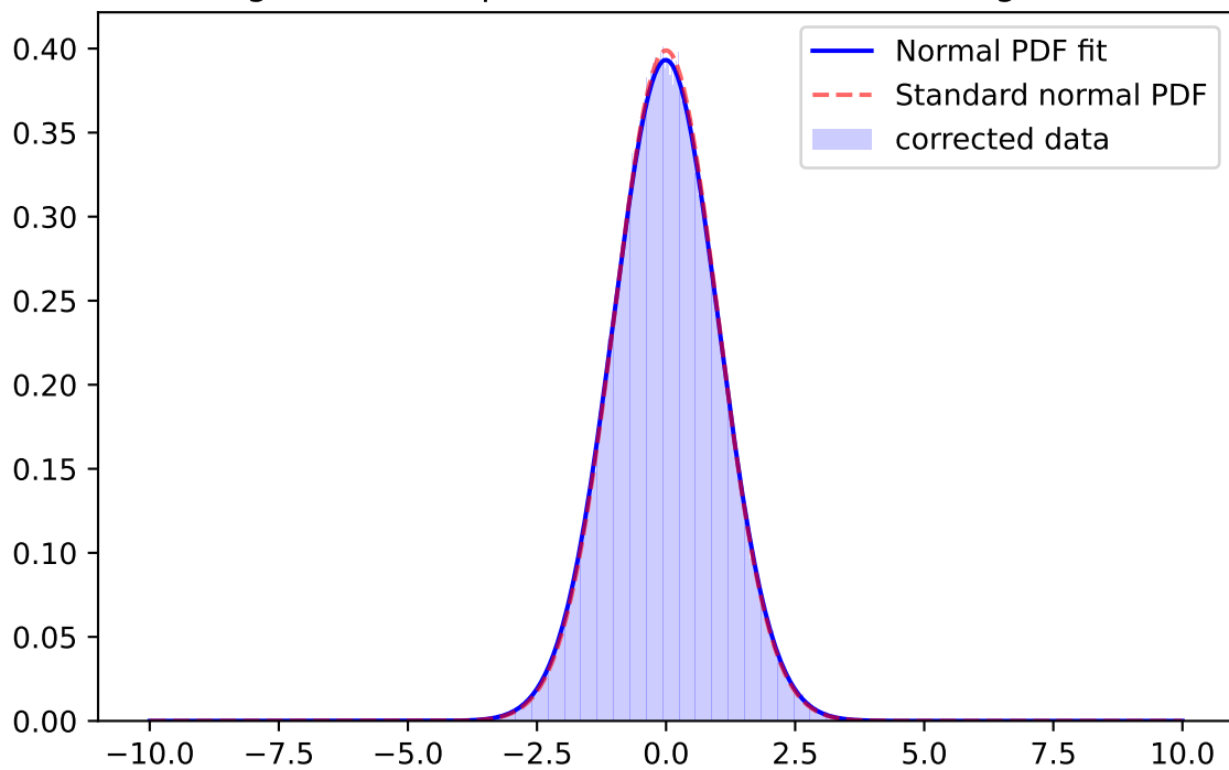
Whiten Signal, z-band, \mu=-0.0167 \sigma=0.9943 ; for mag=[25.0; 25.5]
