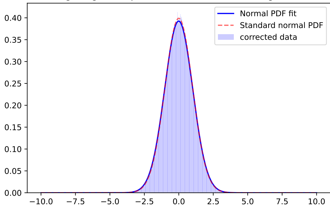
Whiten Signal, i-band, \mu=-0.0049 \sigma=1.0196 ; for mag=[25.0; 25.5]
