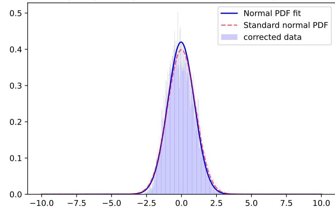
Whiten Signal, y-band, \mu=-0.0318 \sigma=0.9500 ; for mag=[25.0; 25.5]
