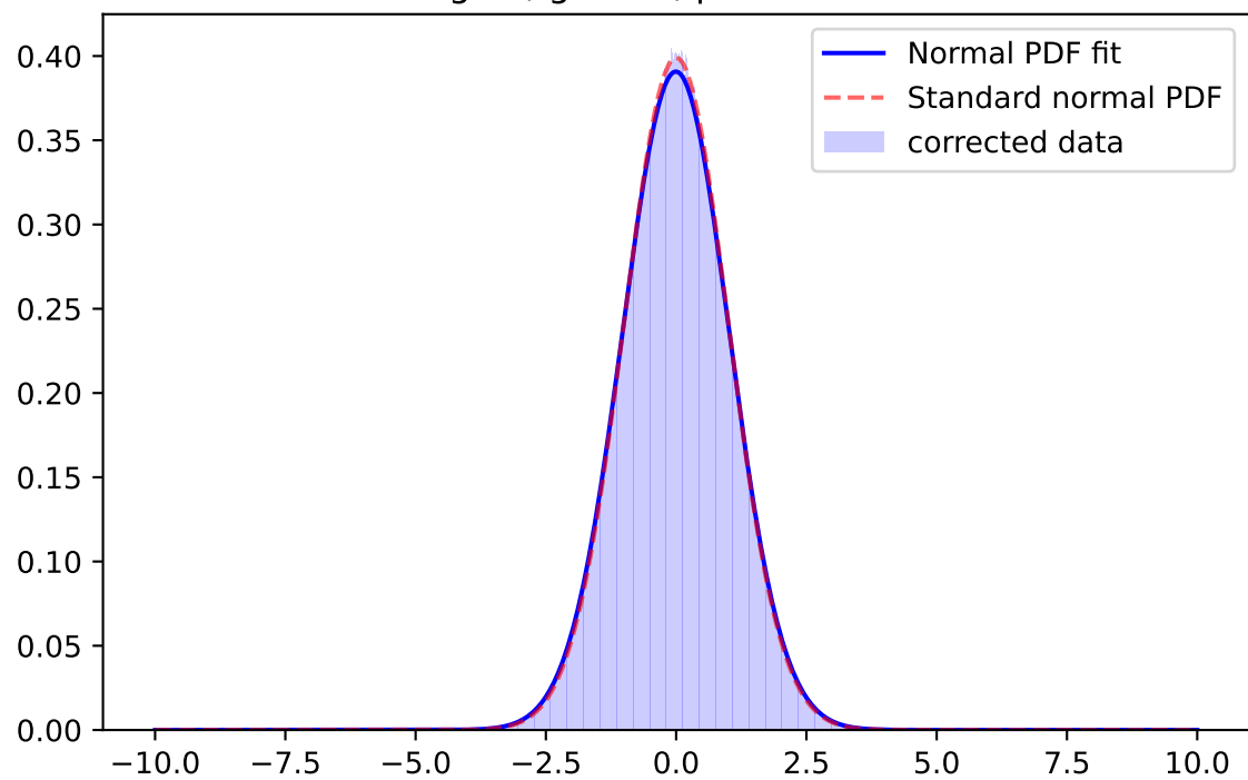
Whiten Signal, i-band, \mu=-0.0014 \sigma=1.0248
