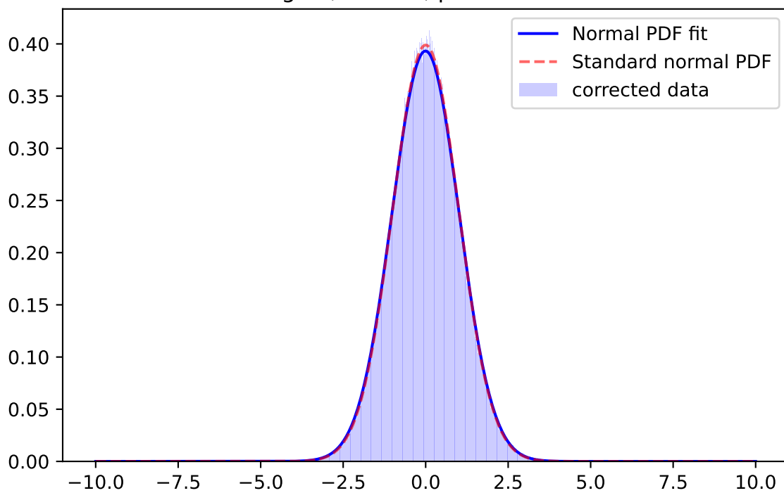
Whiten Signal, r-band, \mu=-0.0011 \sigma=1.0251
