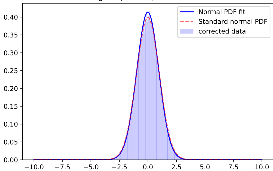
Whiten Signal, y-band, \mu=-0.0091 \sigma=0.9634
