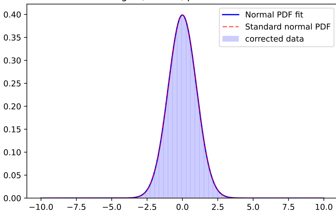
Whiten Signal, z-band, \mu=-0.0055 \sigma=1.0007
