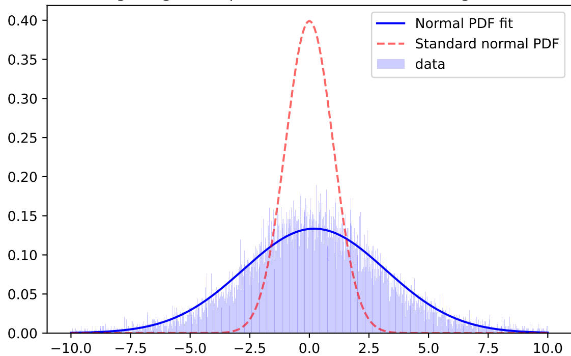
Whiten Signal, i-band, \mu=0.0616 \sigma=2.6499 ; for mag=[18.0; 18.5]
