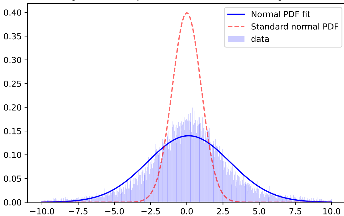
Whiten Signal, z-band, \mu=0.0062 \sigma=1.7609 ; for mag=[18.0; 18.5]
