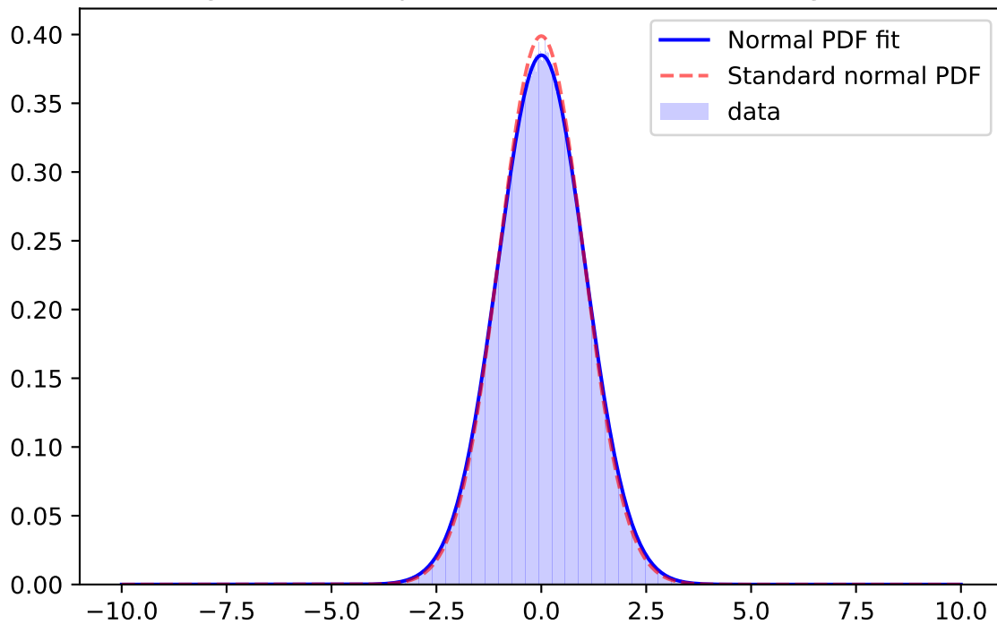
Whiten Signal, z-band, \mu=0.0045 \sigma=1.0362 ; for mag=[25.0; 25.5]
