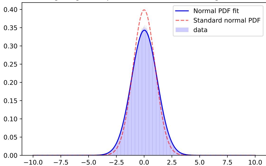
Whiten Signal, i-band, \mu=0.0028 \sigma=1.0483 ; for mag=[25.0; 25.5]
