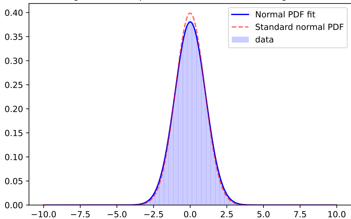
Whiten Signal, y-band, \mu=-0.0012 \sigma=1.0453 ; for mag=[25.0; 25.5]
