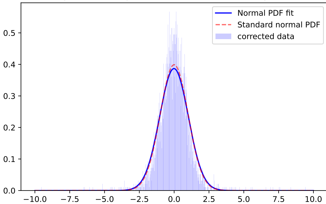
Whiten Signal, z-band, \mu=-0.0118 \sigma=1.0315 ; for mag=[18.0; 18.5]
