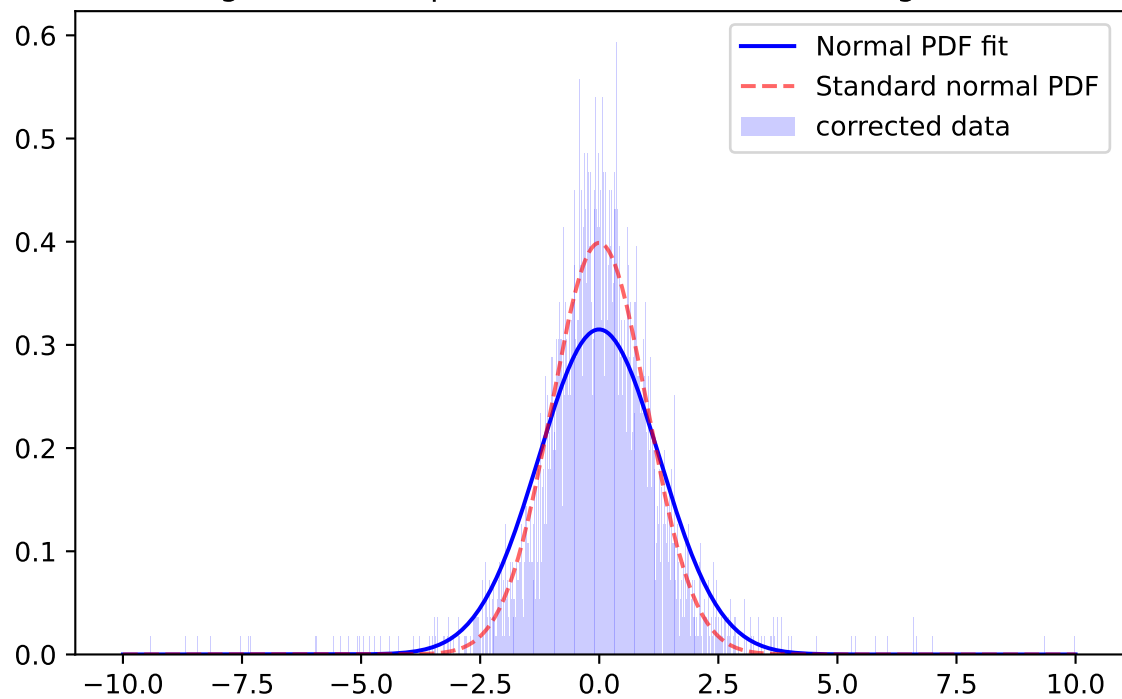
Whiten Signal, y-band, \mu=0.0831 \sigma=1.2365 ; for mag=[18.0; 18.5]
