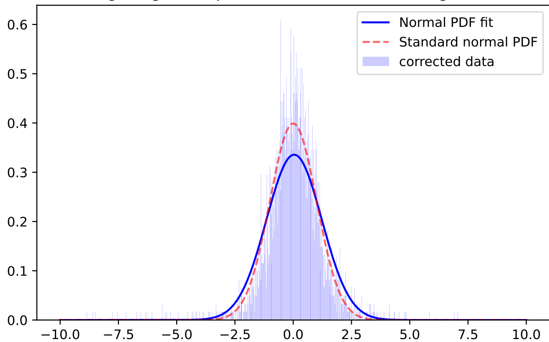
Whiten Signal, i-band, \mu=-0.0040 \sigma=1.2665 ; for mag=[18.0; 18.5]
