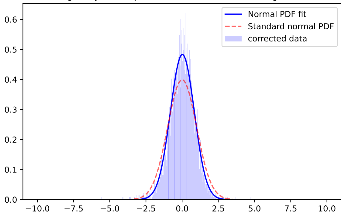
Whiten Signal, y-band, \mu=0.0154 \sigma=0.8254 ; for mag=[21.0; 21.5]
