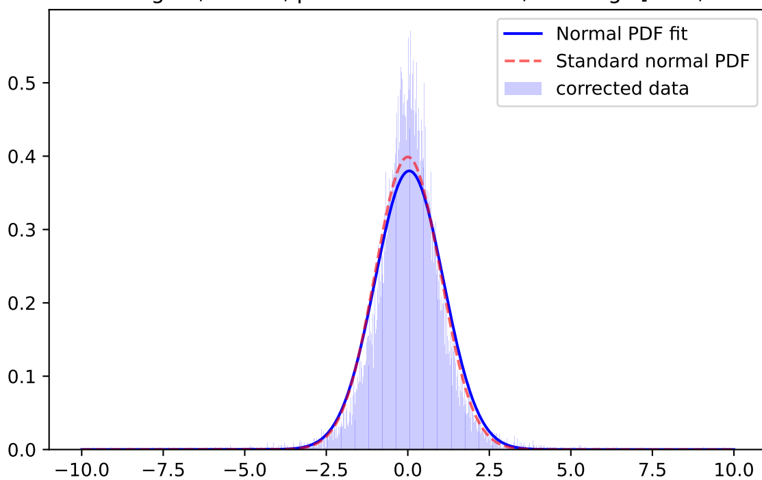
Whiten Signal, z-band, \mu=0.0462 \sigma=0.8994 ; for mag=[21.0; 21.5]
