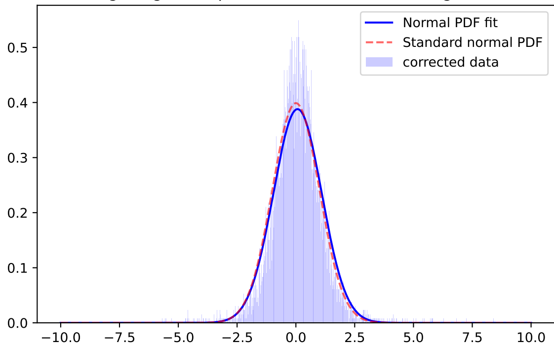
Whiten Signal, i-band, \mu=0.0254 \sigma=1.0099 ; for mag=[21.0; 21.5]
