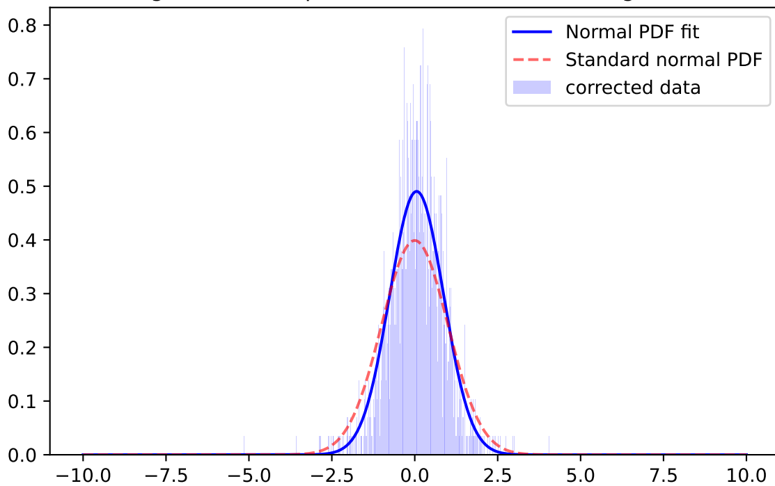
Whiten Signal, r-band, \mu=0.0441 \sigma=1.0500 ; for mag=[21.0; 21.5]
