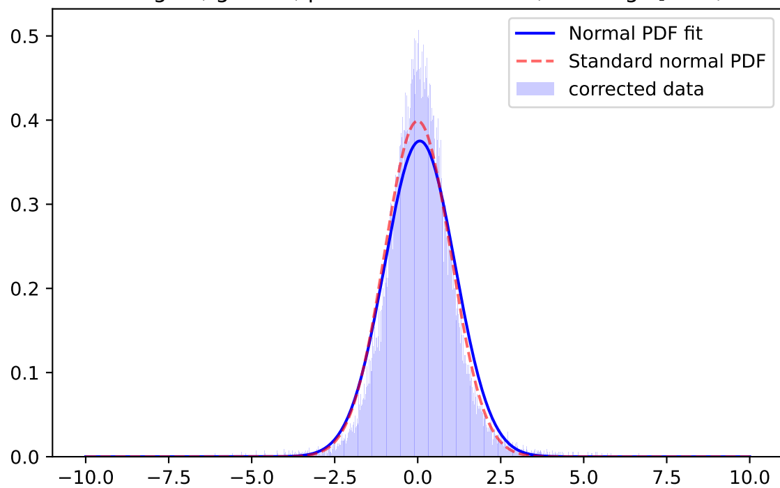
Whiten Signal, i-band, \mu=0.0362 \sigma=1.0167 ; for mag=[21.0; 21.5]
