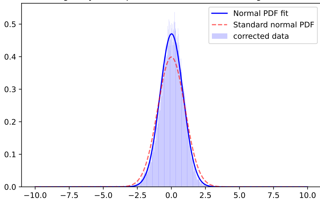
Whiten Signal, y-band, \mu=0.0152 \sigma=0.8485 ; for mag=[21.0; 21.5]
