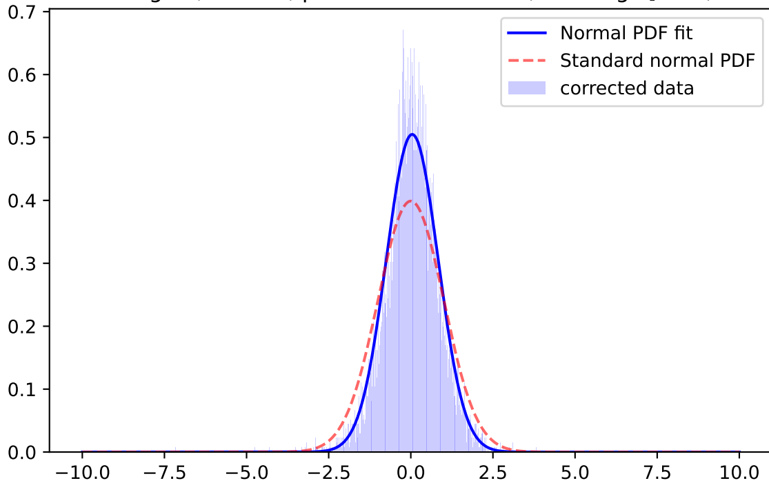
Whiten Signal, r-band, \mu=0.0563 \sigma=1.0894 ; for mag=[21.0; 21.5]
