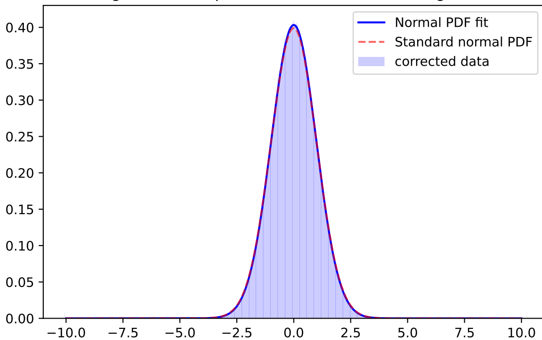
Whiten Signal, z-band, \mu=-0.0262 \sigma=0.9851 ; for mag=[25.0; 25.5]
