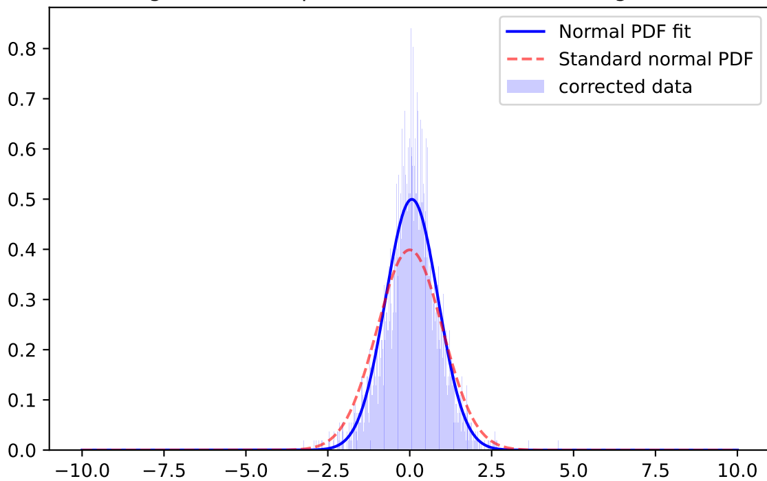
Whiten Signal, r-band, \mu=0.0552 \sigma=1.0684 ; for mag=[21.0; 21.5]
