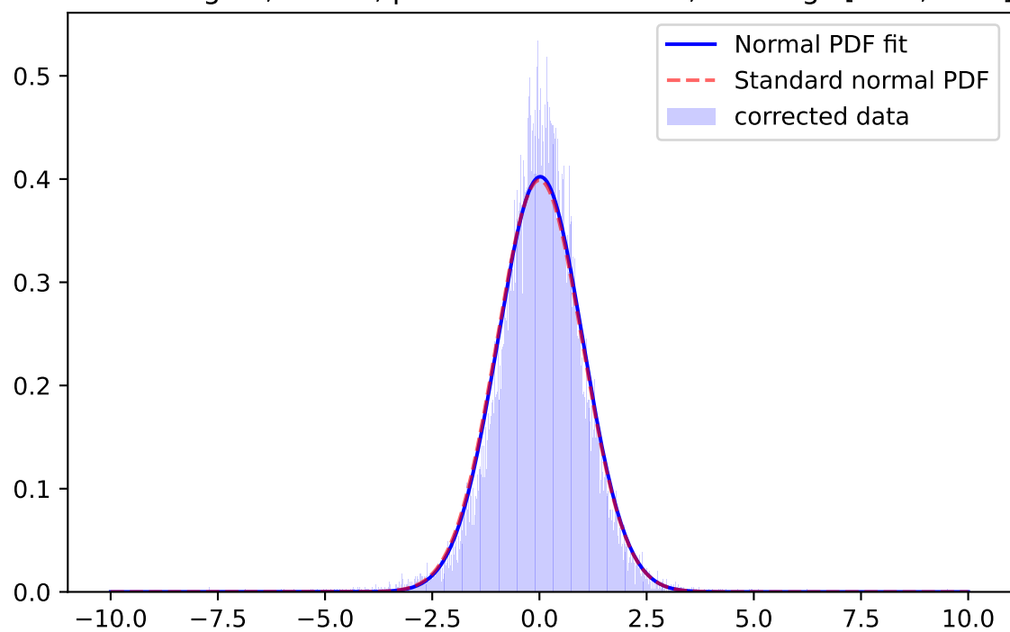
Whiten Signal, y-band, \mu=-0.0005 \sigma=0.8569 ; for mag=[21.0; 21.5]
