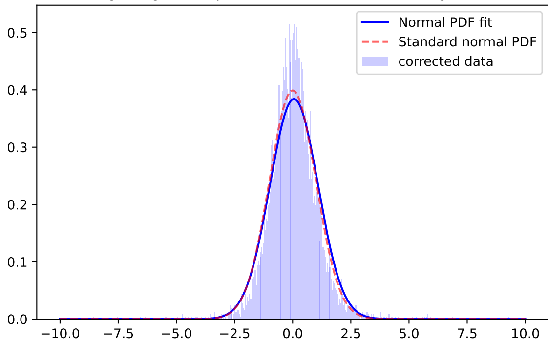
Whiten Signal, i-band, \mu=0.0212 \sigma=0.9917 ; for mag=[21.0; 21.5]
