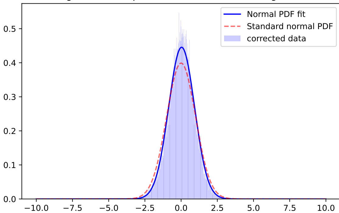
Whiten Signal, z-band, \mu=0.0349 \sigma=0.8955 ; for mag=[21.0; 21.5]
