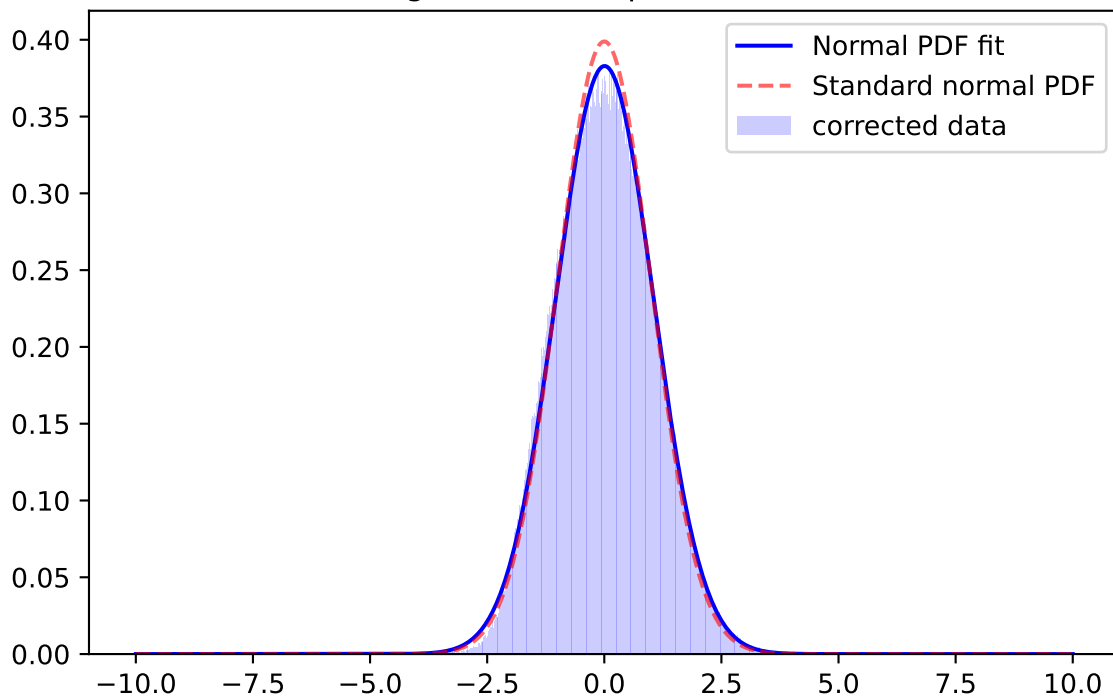
Whiten Signal, r-band, \mu=0.0228 \sigma=1.0189
