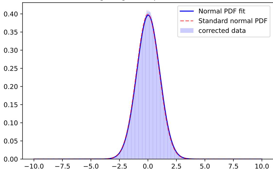
Whiten Signal, i-band, \mu=-0.0001 \sigma=1.0010
