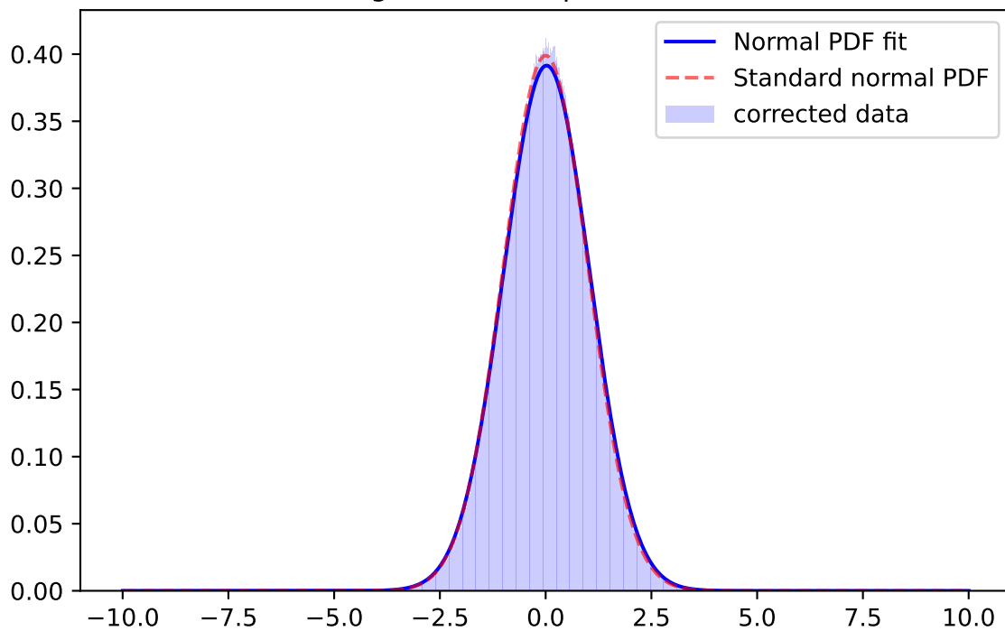
Whiten Signal, z-band, \mu=0.0074 \sigma=1.0021
