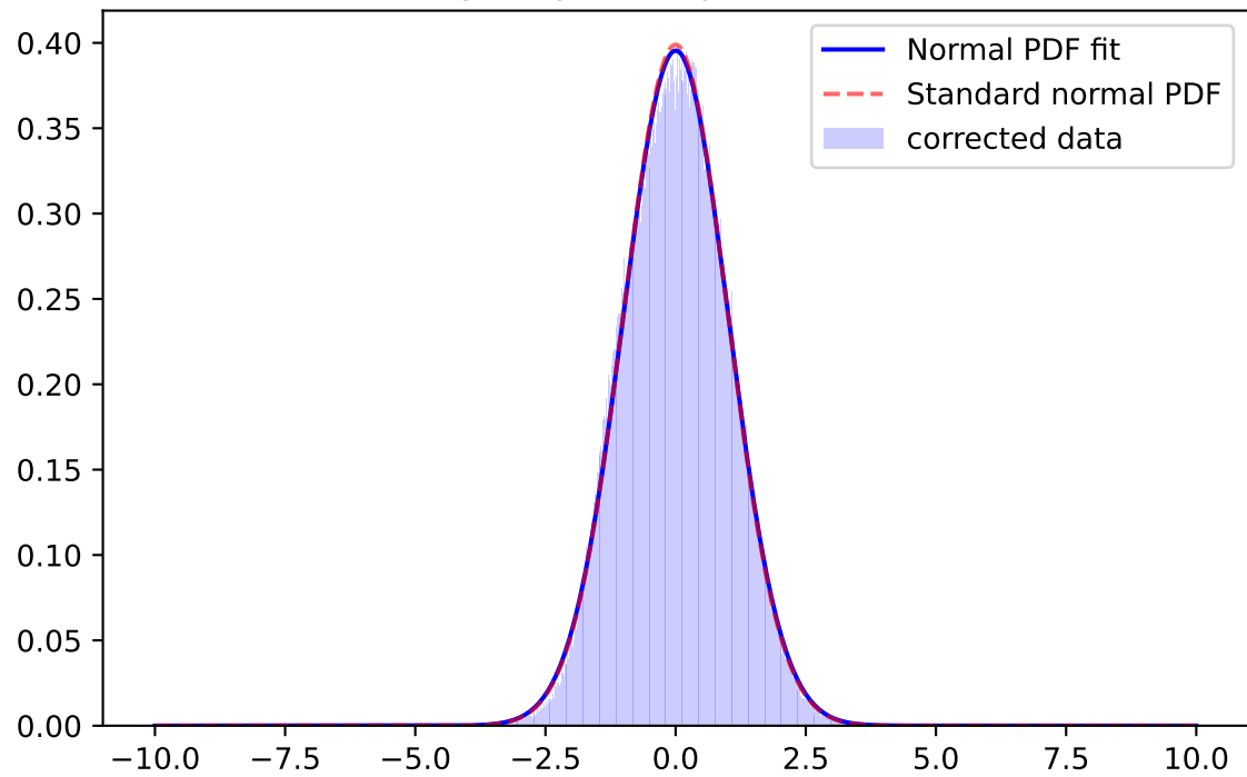
Whiten Signal, y-band, \mu=0.0030 \sigma=1.0087
