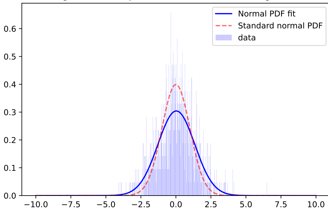
Whiten Signal, r-band, \mu=-0.0250 \sigma=1.6561 ; for mag=[21.0; 21.5]
