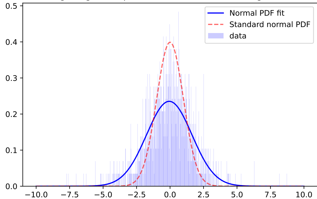
Whiten Signal, i-band, \mu=-0.2586 \sigma=1.8577 ; for mag=[21.0; 21.5]
