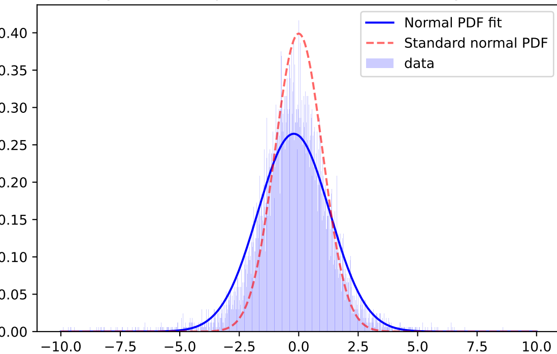
Whiten Signal, z-band, \mu=-0.2057 \sigma=1.5065 ; for mag=[21.0; 21.5]
