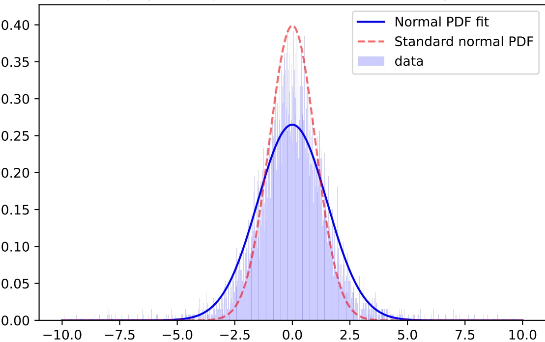
Whiten Signal, y-band, \mu=-0.0009 \sigma=1.5062 ; for mag=[21.0; 21.5]
