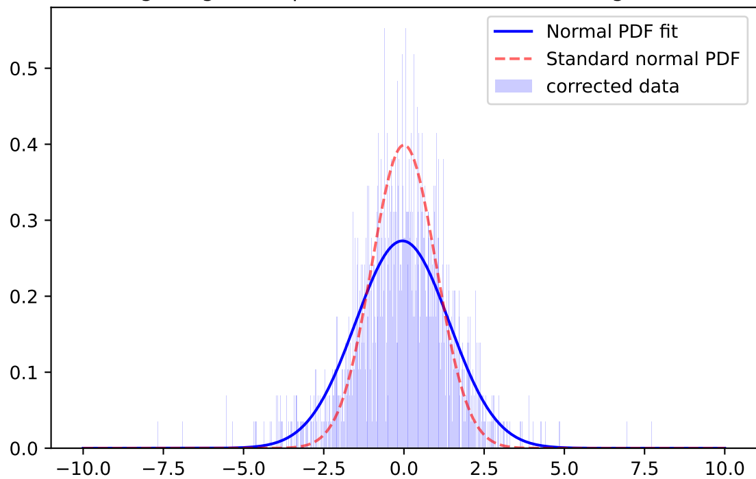
Whiten Signal, i-band, \mu=-0.2435 \sigma=1.7993 ; for mag=[21.0; 21.5]
