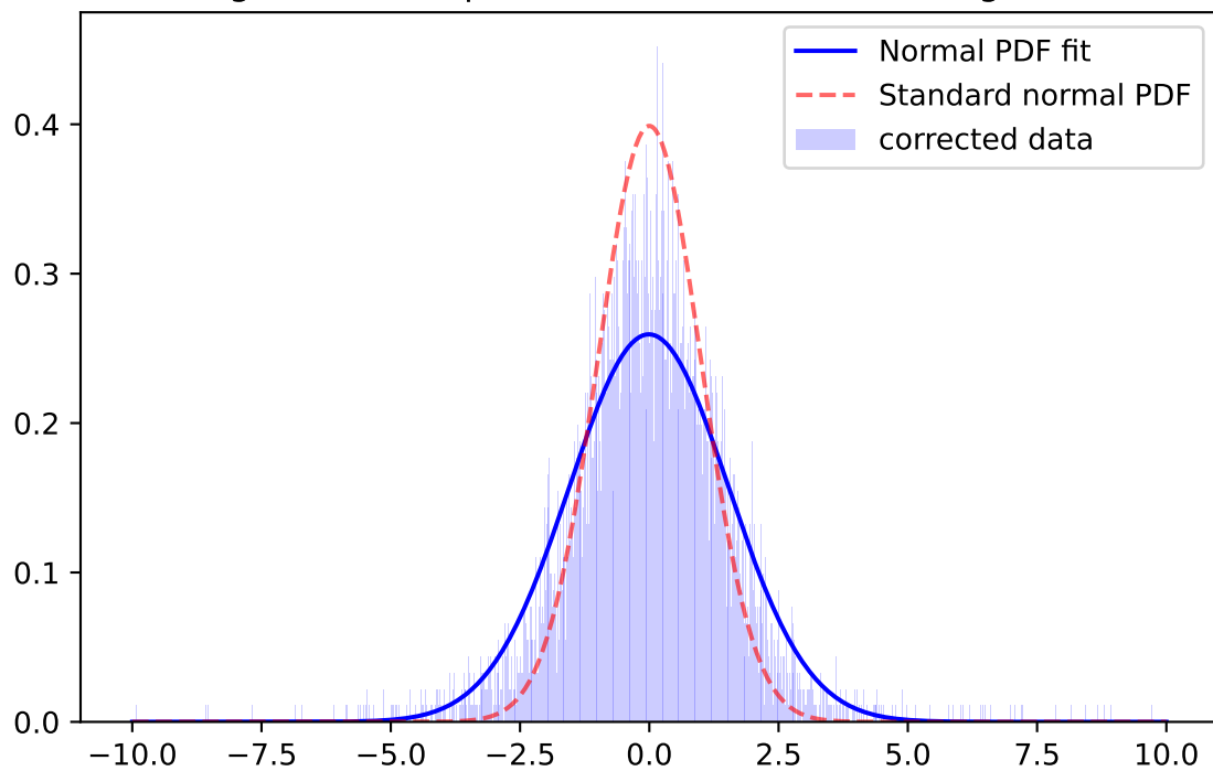
Whiten Signal, z-band, \mu=-0.1987 \sigma=1.4880 ; for mag=[21.0; 21.5]
