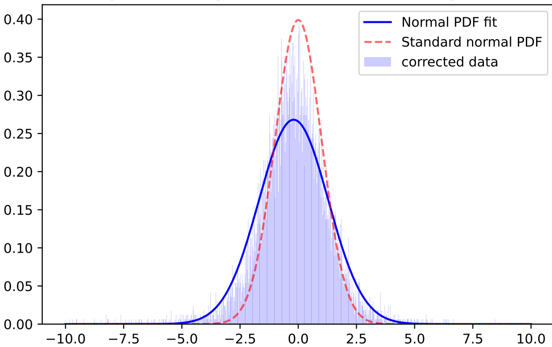
Whiten Signal, z-band, \mu=-0.1987 \sigma=1.4880 ; for mag=[21.0; 21.5]
