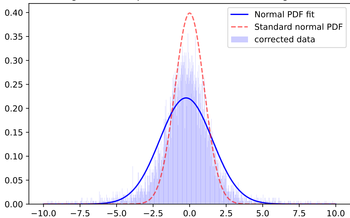
Whiten Signal, y-band, \mu=0.0004 \sigma=1.5012 ; for mag=[21.0; 21.5]
