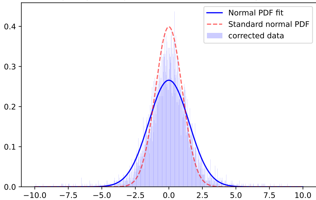
Whiten Signal, y-band, \mu=0.0004 \sigma=1.5012 ; for mag=[21.0; 21.5]
