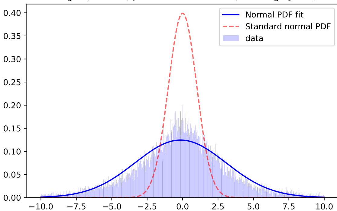
Whiten Signal, z-band, \mu=-0.1448 \sigma=3.2034 ; for mag=[18.0; 18.5]
