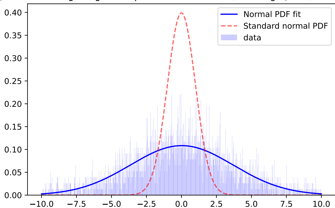
Whiten Signal, i-band, \mu=0.1537 \sigma=3.7379 ; for mag=[18.0; 18.5]
