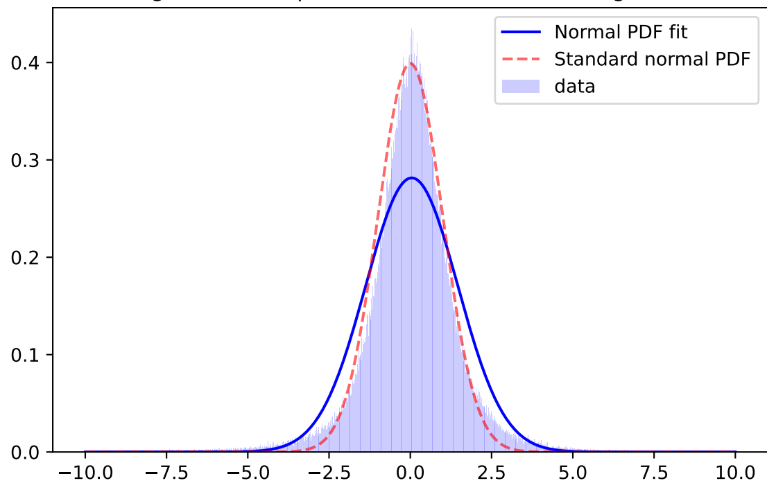
Whiten Signal, y-band, \mu=-0.0122 \sigma=1.2222 ; for mag=[21.0; 21.5]
