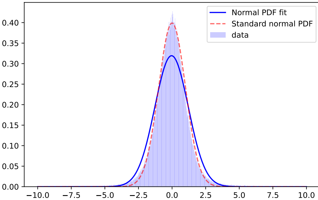
Whiten Signal, z-band, \mu=-0.0367 \sigma=1.2493 ; for mag=[21.0; 21.5]
