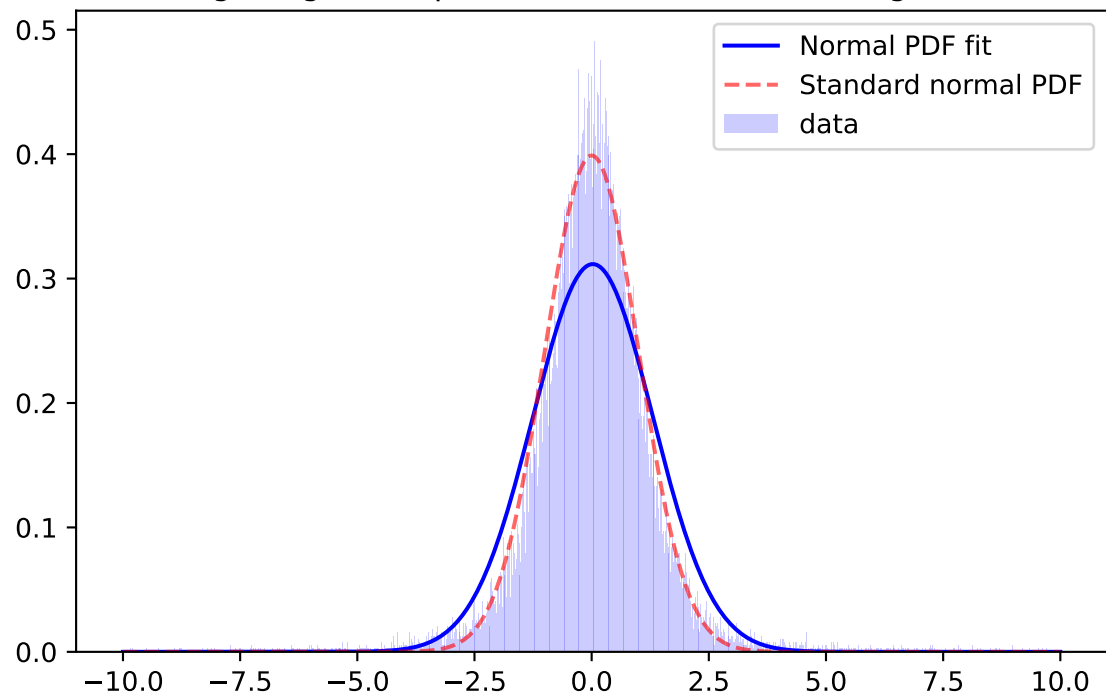
Whiten Signal, i-band, \mu=0.0439 \sigma=1.4171 ; for mag=[21.0; 21.5]
