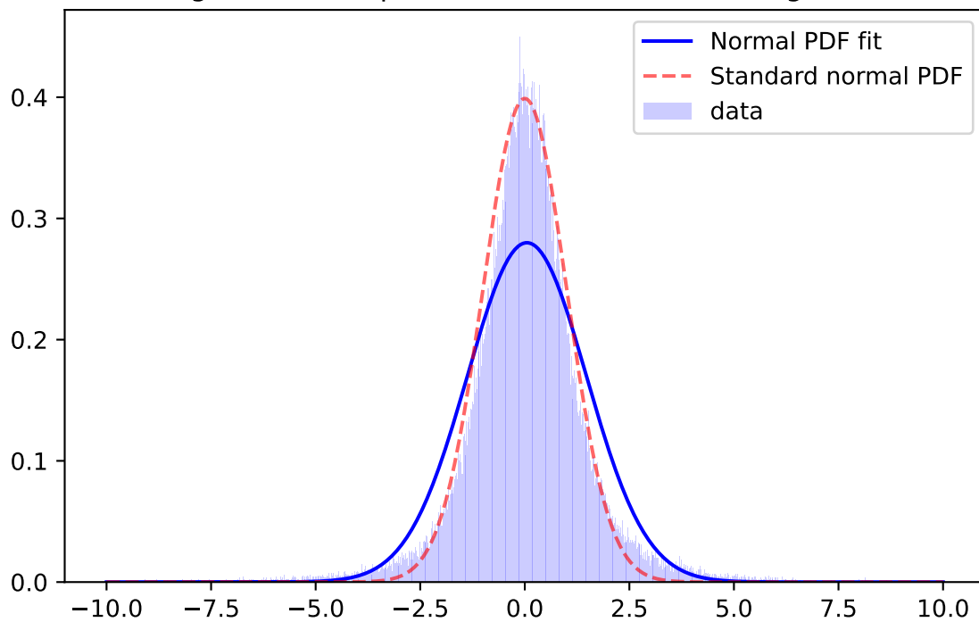
Whiten Signal, z-band, \mu=-0.0367 \sigma=1.2493 ; for mag=[21.0; 21.5]
