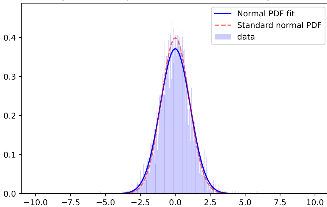
Whiten Signal, r-band, \mu=0.0497 \sigma=1.4249 ; for mag=[21.0; 21.5]
