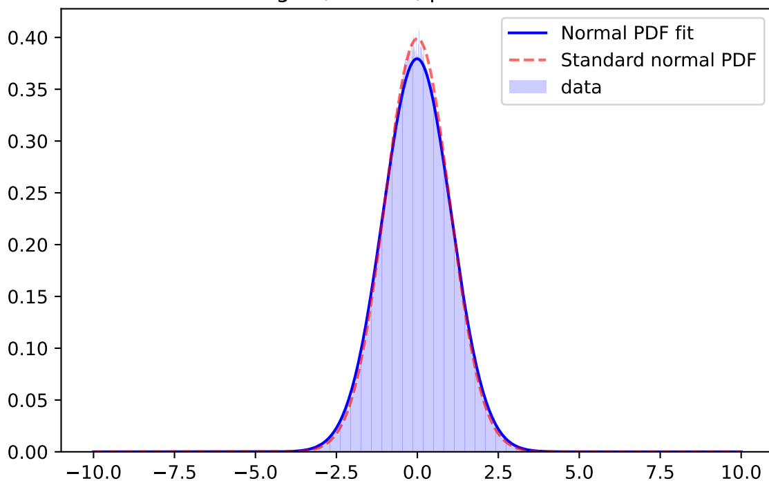
Whiten Signal, r-band, \mu=0.0041 \sigma=1.1246
