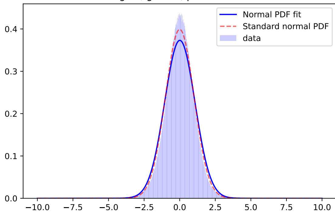
Whiten Signal, i-band, \mu=-0.0007 \sigma=1.1088
