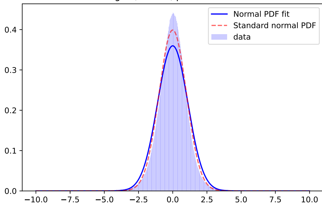
Whiten Signal, y-band, \mu=-0.0135 \sigma=1.1552
