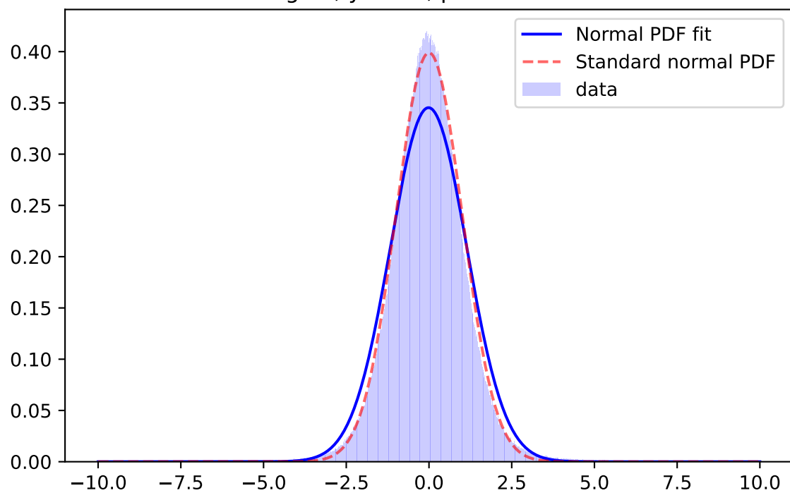
Whiten Signal, y-band, \mu=-0.0135 \sigma=1.1552
