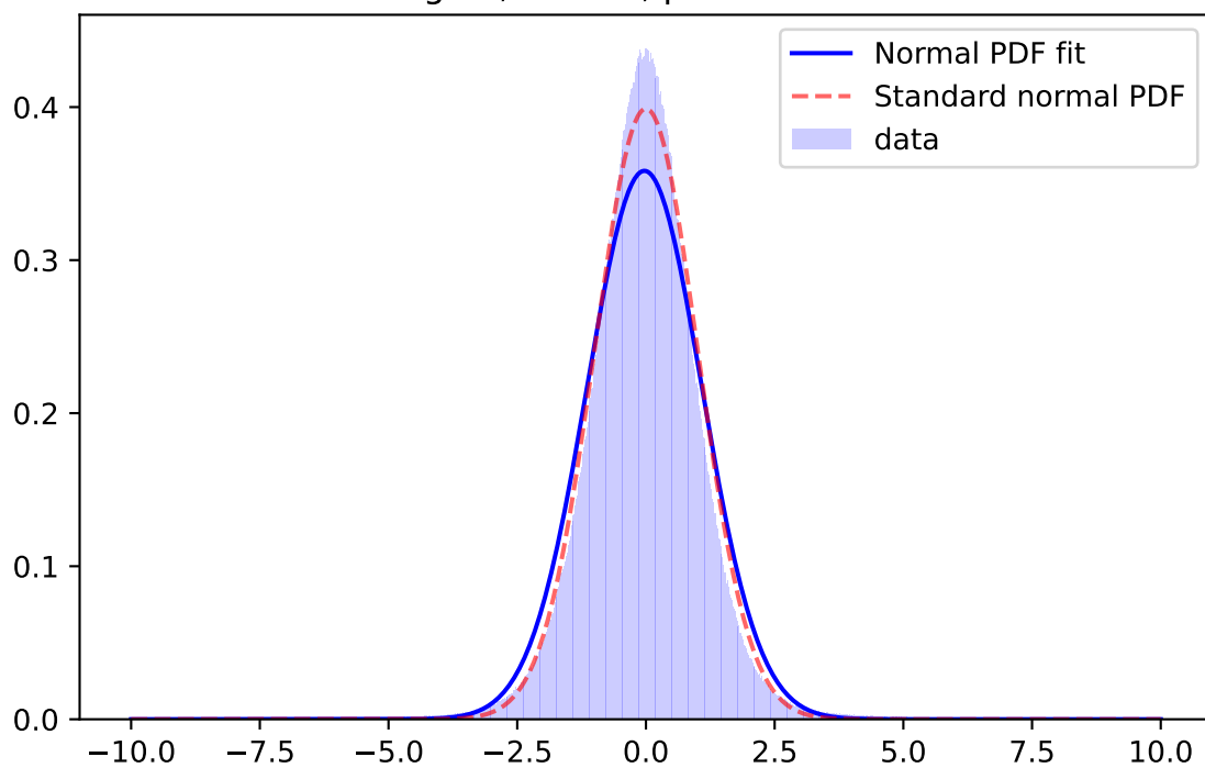
Whiten Signal, z-band, \mu=-0.0300 \sigma=1.1132
