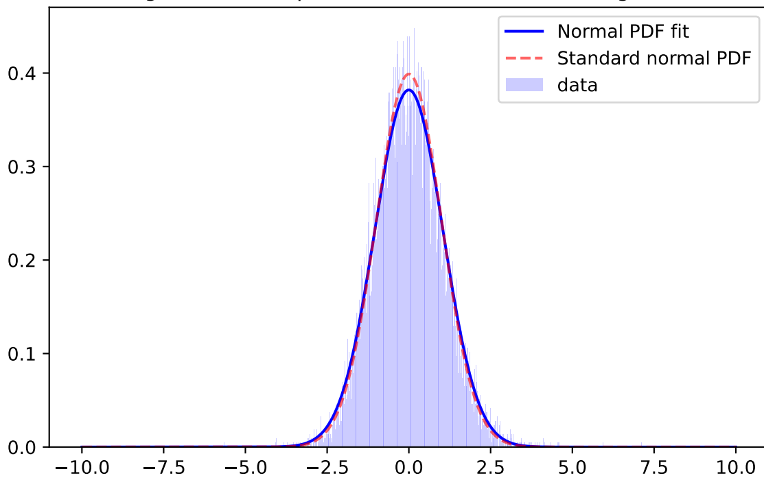
Whiten Signal, r-band, \mu=-0.0116 \sigma=0.9912 ; for mag=[25.0; 25.5]
