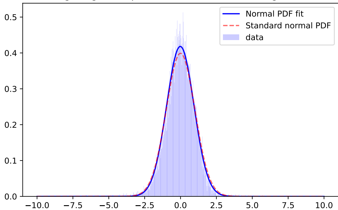
Whiten Signal, i-band, \mu=-0.0272 \sigma=0.9609 ; for mag=[25.0; 25.5]
