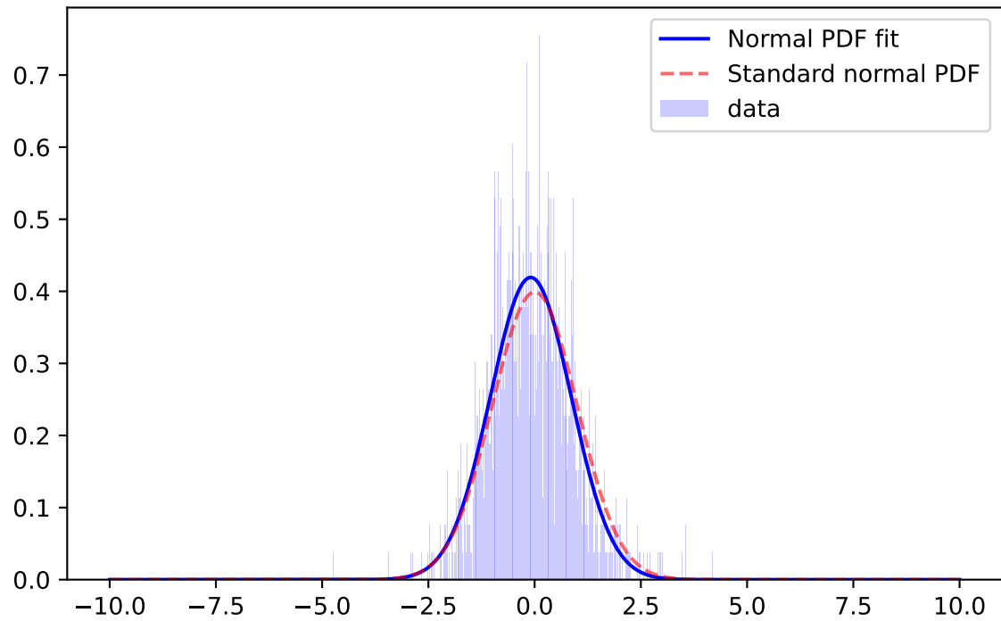
Whiten Signal, y-band, \mu=-0.0922 \sigma=0.9515 ; for mag=[25.0; 25.5]
