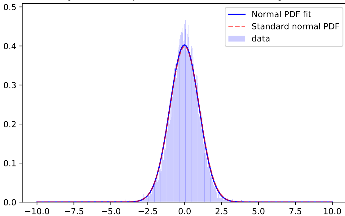
Whiten Signal, z-band, \mu=-0.0495 \sigma=0.9369 ; for mag=[25.0; 25.5]
