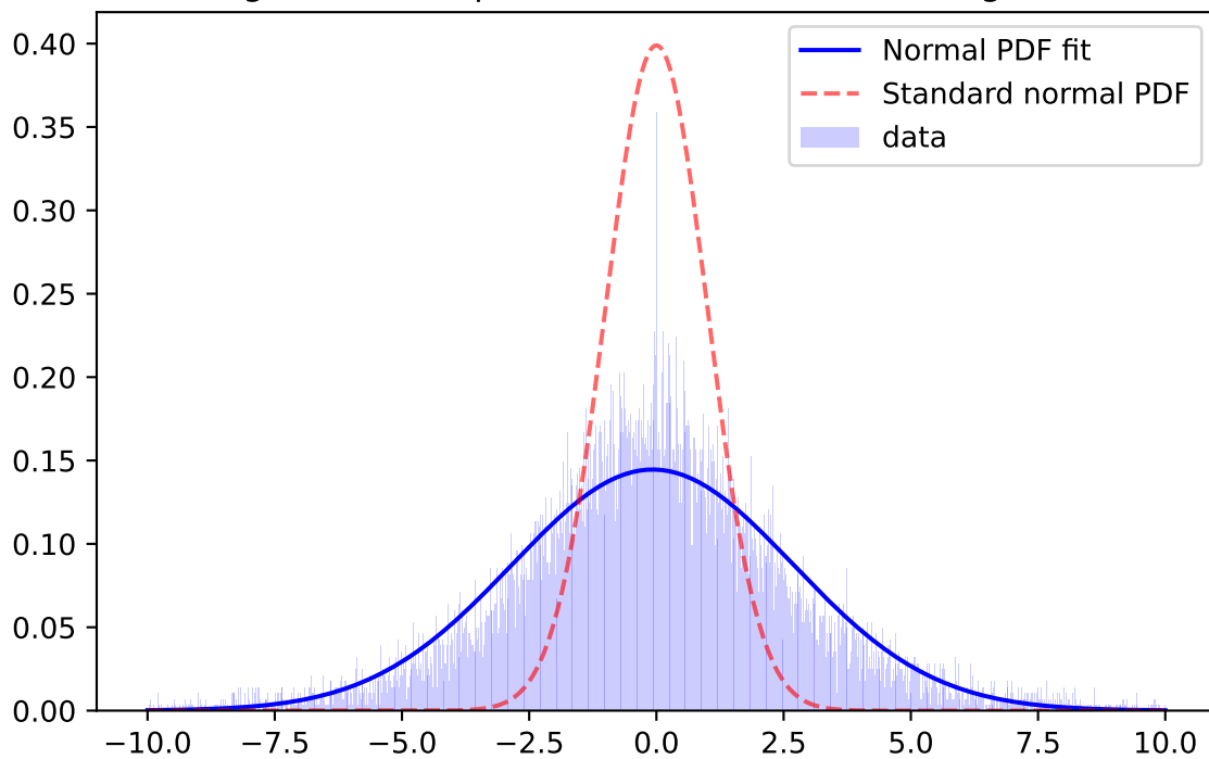
Whiten Signal, z-band, \mu=-0.1126 \sigma=1.9198 ; for mag=[18.0; 18.5]
