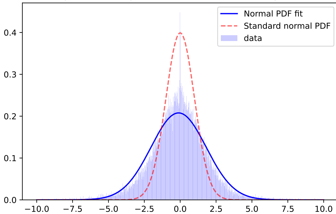
Whiten Signal, z-band, \mu=-0.1126 \sigma=1.9198 ; for mag=[18.0; 18.5]
