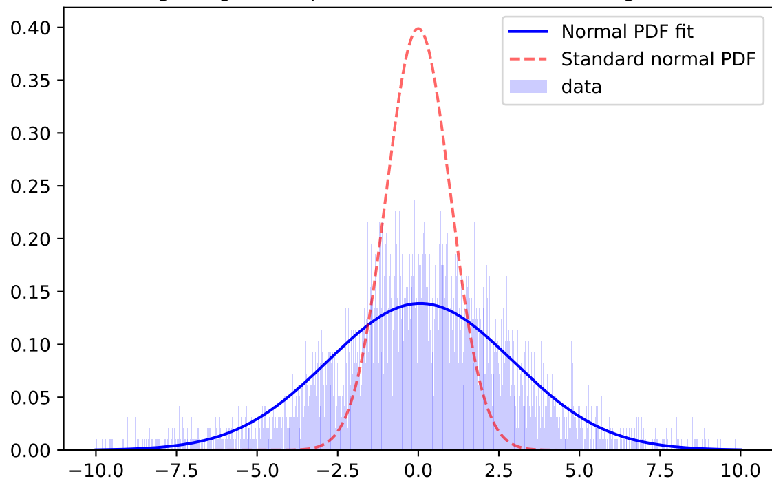
Whiten Signal, i-band, \mu=-0.2061 \sigma=2.8167 ; for mag=[18.0; 18.5]
