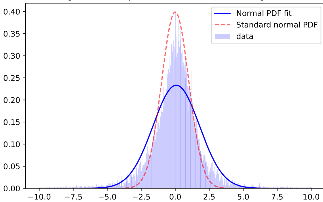
Whiten Signal, z-band, \mu=0.0192 \sigma=1.2551 ; for mag=[18.0; 18.5]
