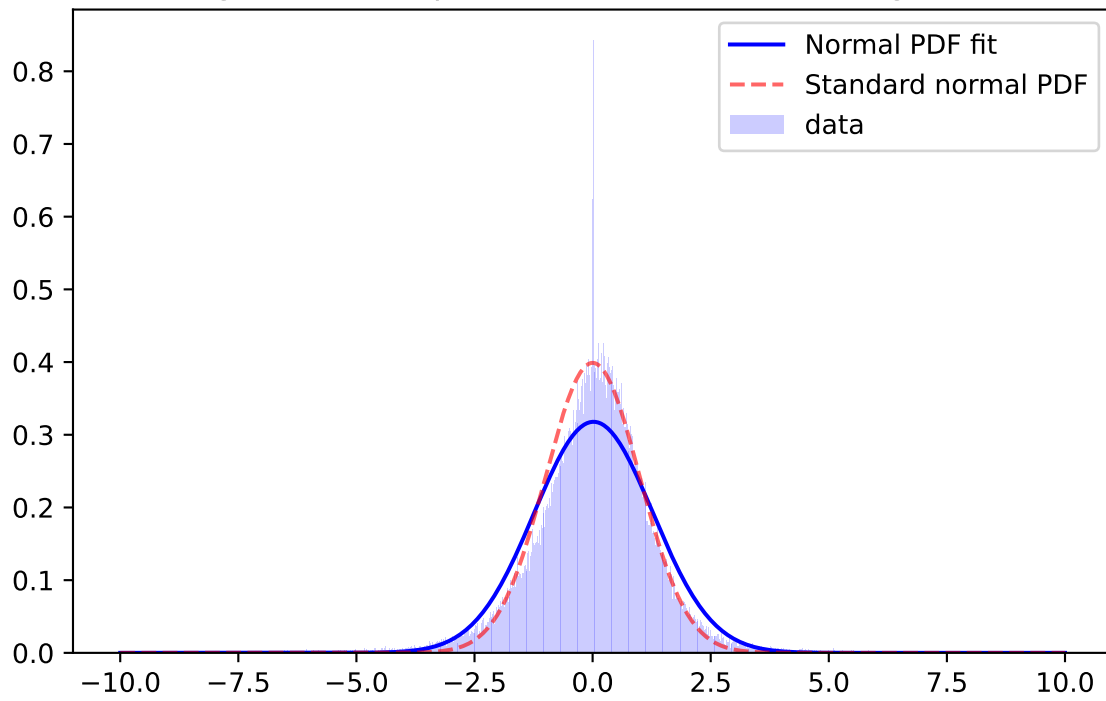
Whiten Signal, z-band, \mu=0.0192 \sigma=1.2551 ; for mag=[18.0; 18.5]
