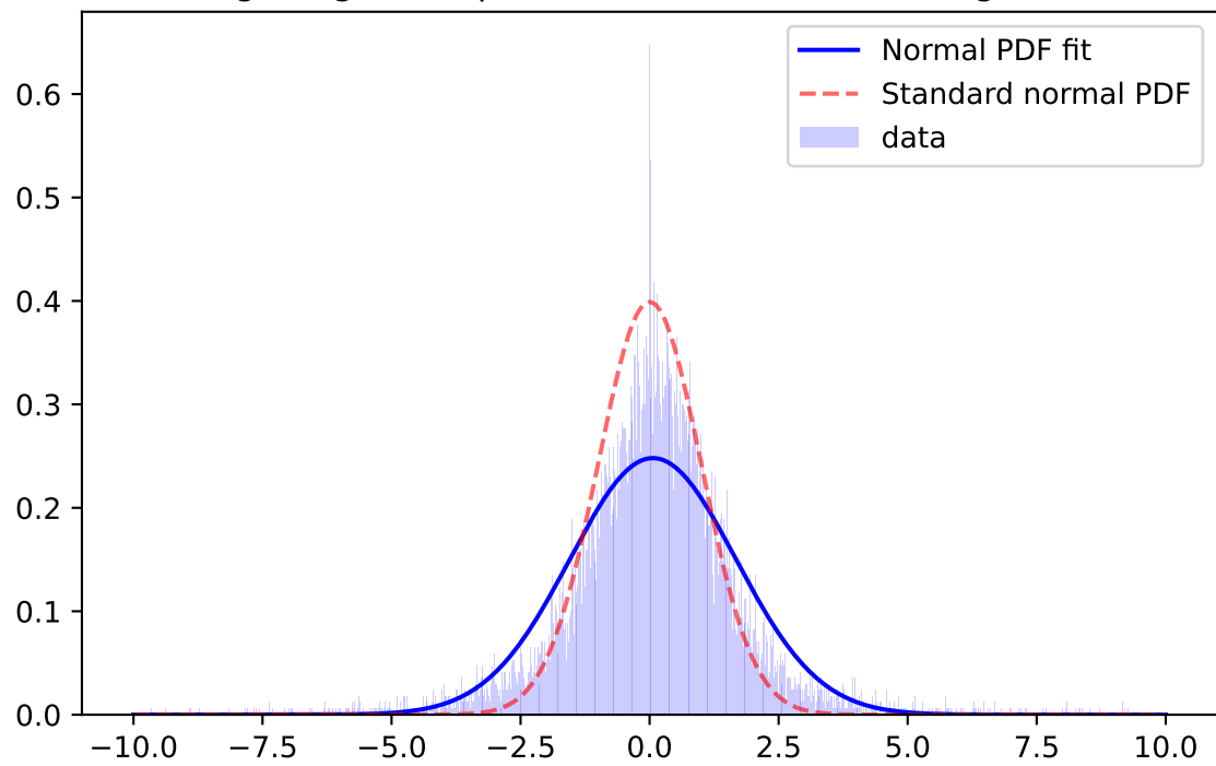
Whiten Signal, i-band, \mu=0.0270 \sigma=1.6916 ; for mag=[18.0; 18.5]
