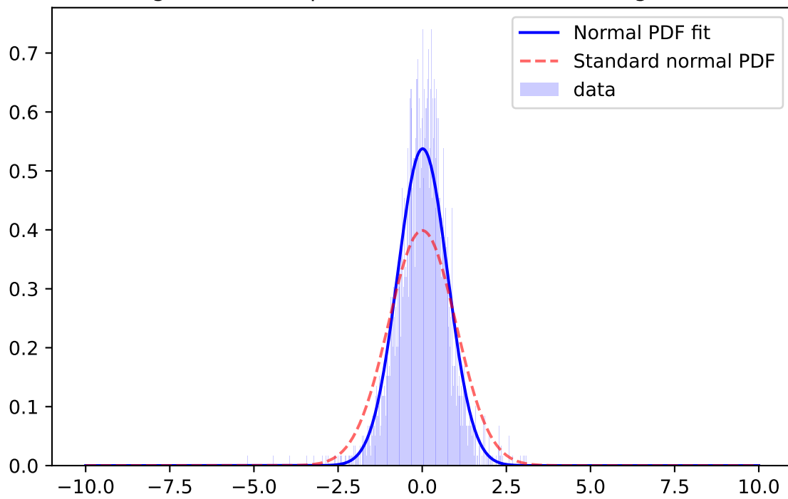
Whiten Signal, r-band, \mu=0.0769 \sigma=1.7102 ; for mag=[18.0; 18.5]
