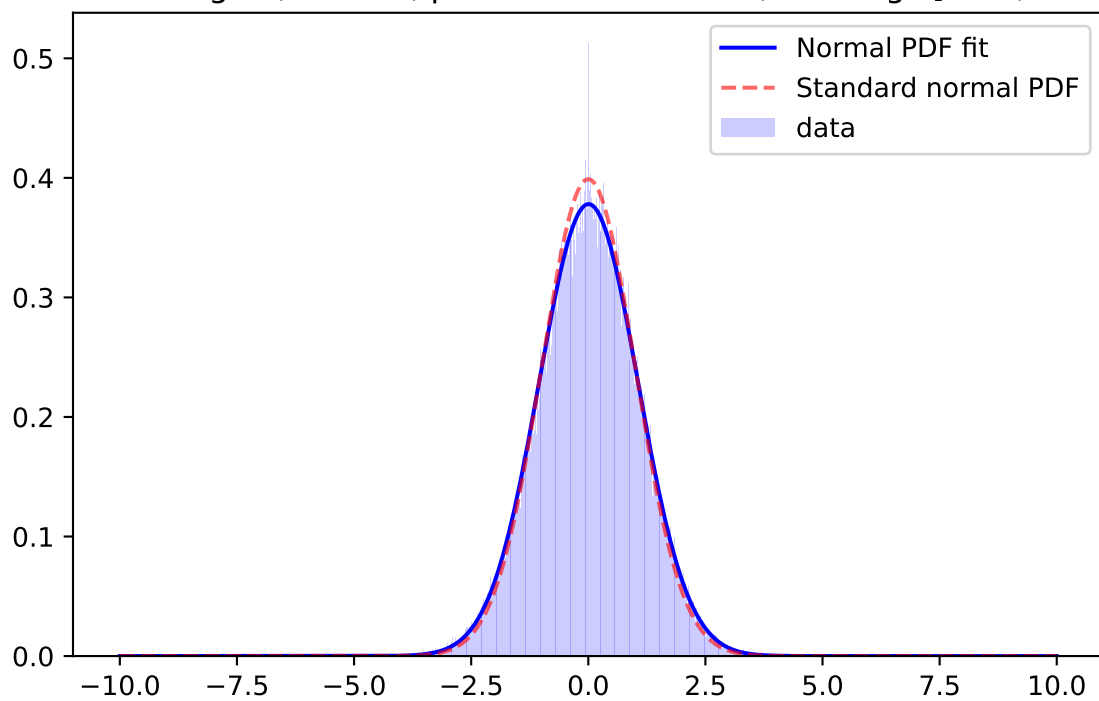
Whiten Signal, r-band, \mu=-0.0013 \sigma=1.0422 ; for mag=[25.0; 25.5]
