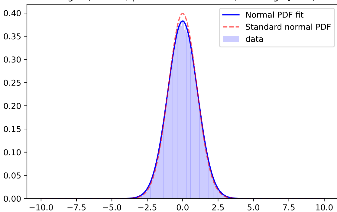
Whiten Signal, z-band, \mu=-0.0116 \sigma=0.9763 ; for mag=[25.0; 25.5]
