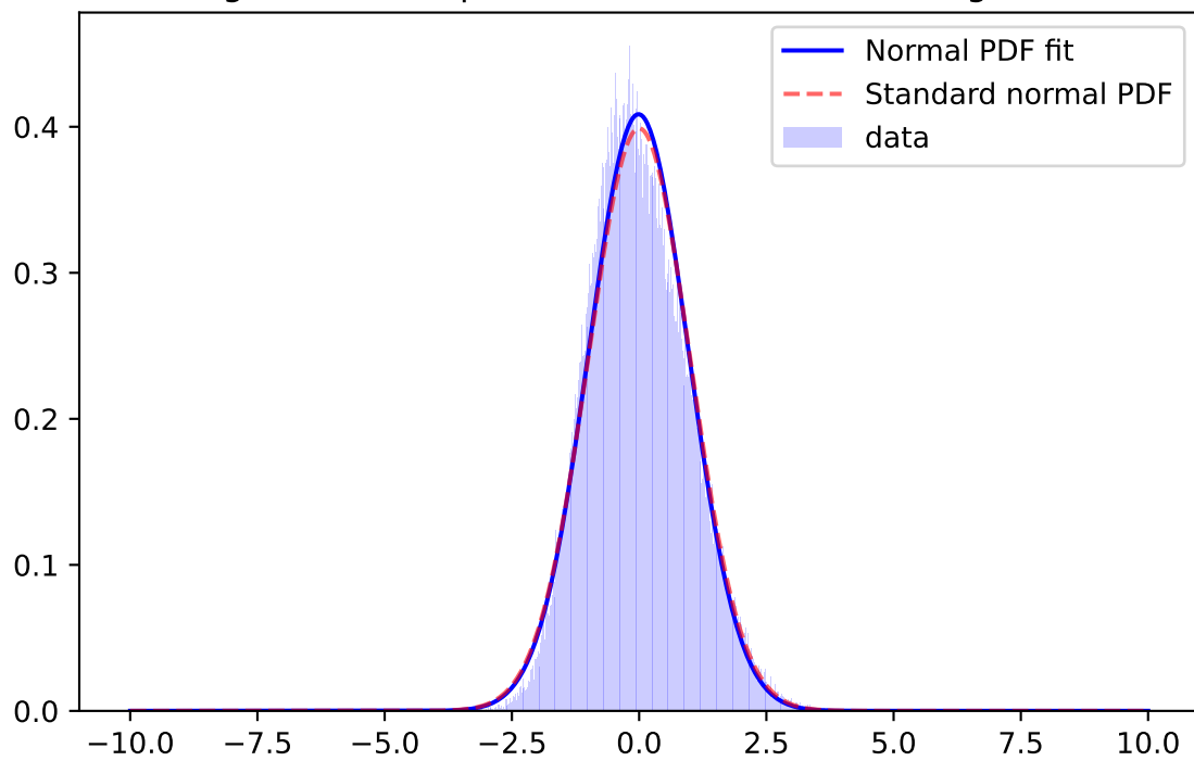
Whiten Signal, z-band, \mu=-0.0116 \sigma=0.9763 ; for mag=[25.0; 25.5]
