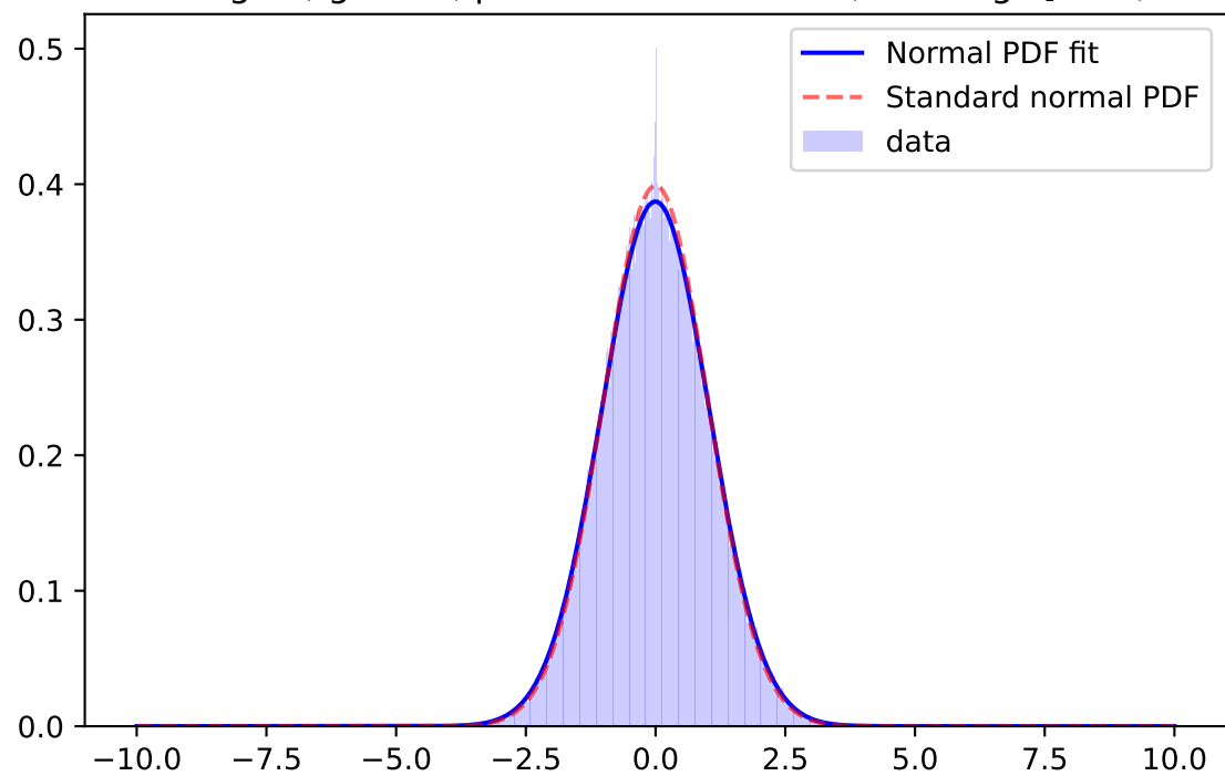
Whiten Signal, i-band, \mu=-0.0023 \sigma=1.0058 ; for mag=[25.0; 25.5]
