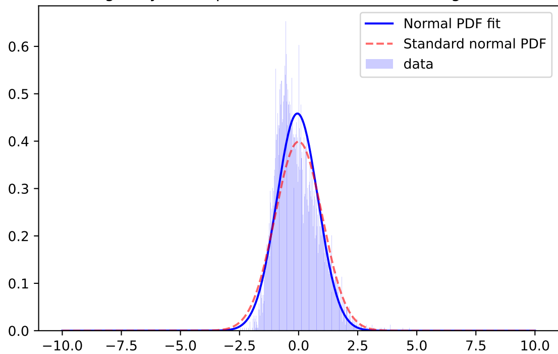
Whiten Signal, y-band, \mu=-0.0520 \sigma=0.8703 ; for mag=[25.0; 25.5]
