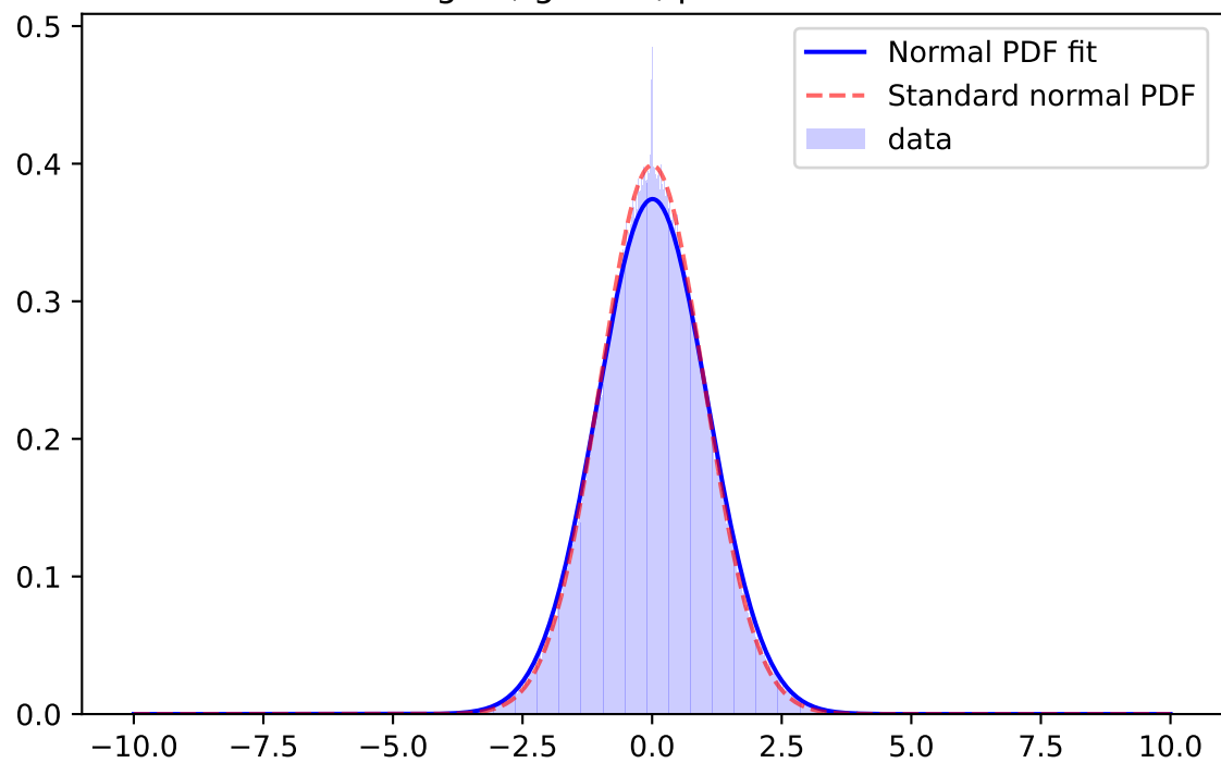
Whiten Signal, i-band, \mu=-0.0012 \sigma=1.0900
