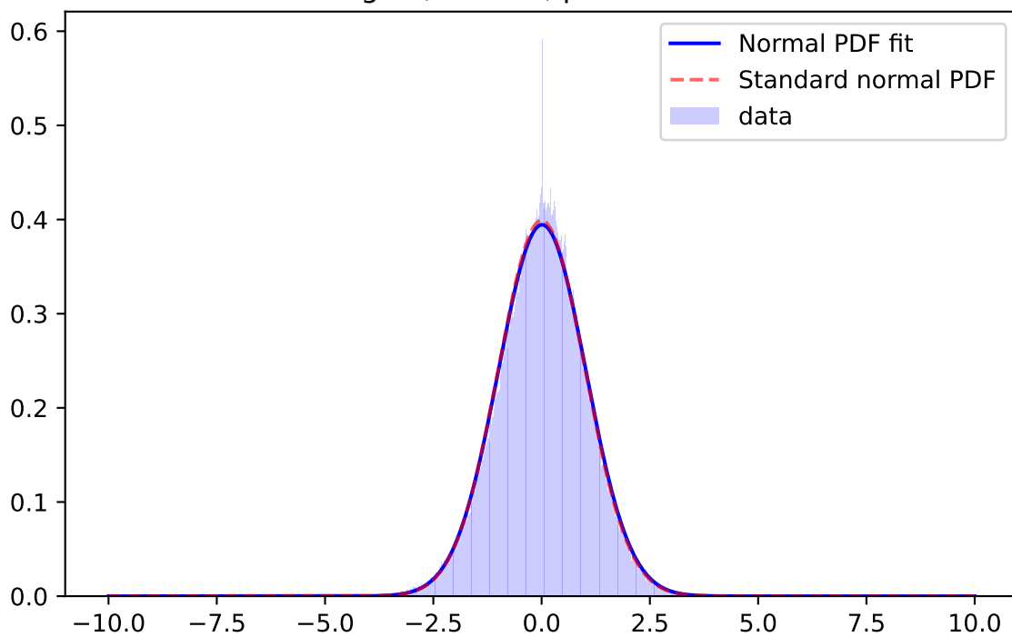
Whiten Signal, r-band, \mu=0.0051 \sigma=1.0877
