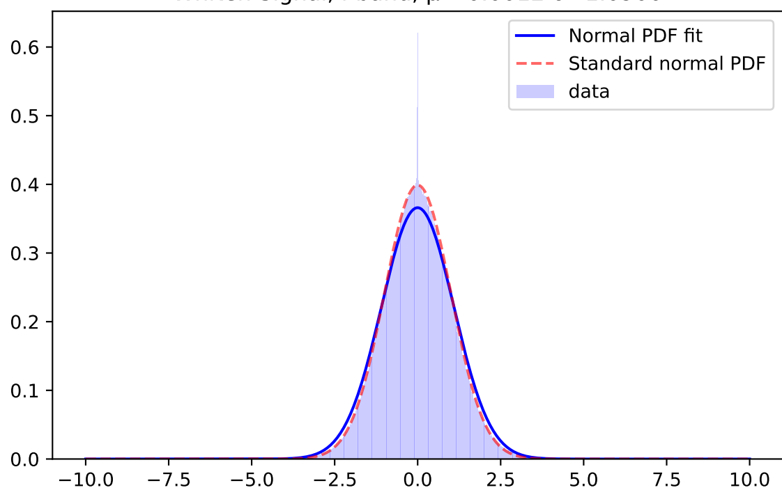
Whiten Signal, y-band, \mu=0.0155 \sigma=1.0355
