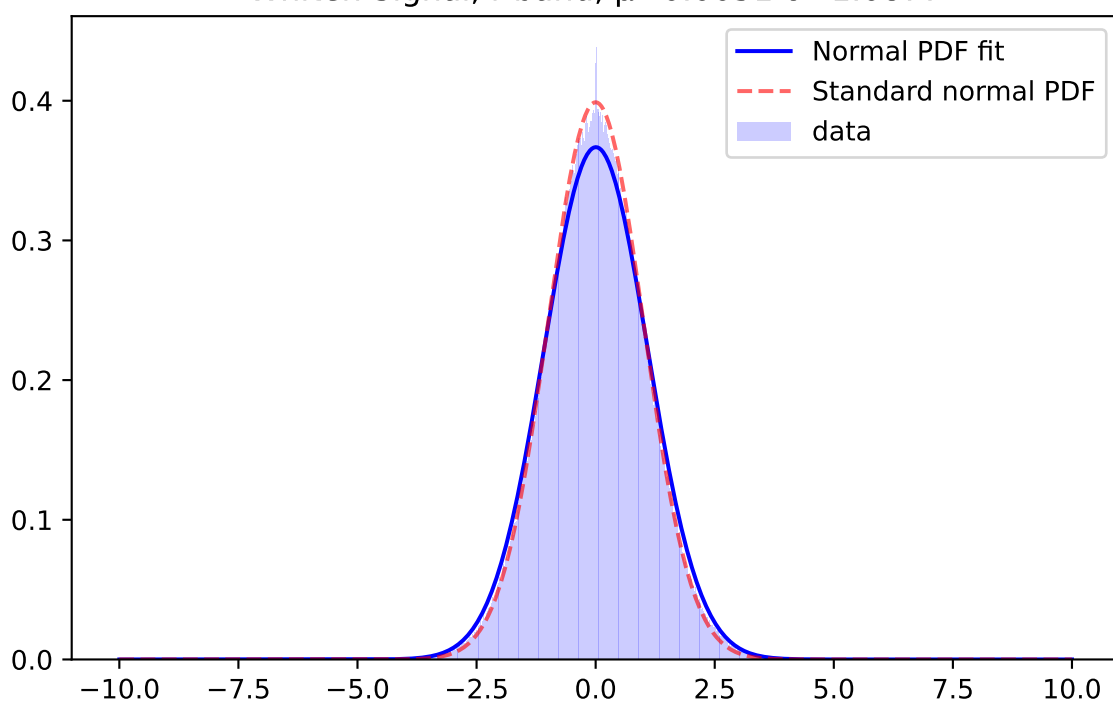
Whiten Signal, z-band, \mu=-0.0016 \sigma=1.0521
