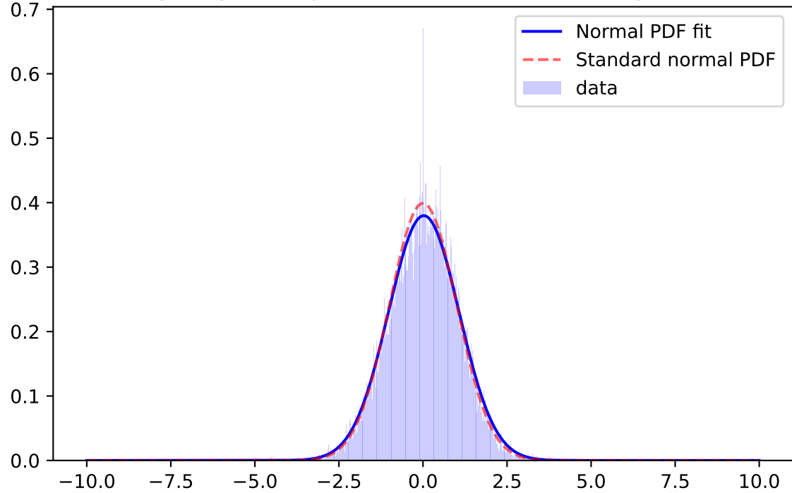
Whiten Signal, y-band, \mu=0.0236 \sigma=1.0503 ; for mag=[21.0; 21.5]
