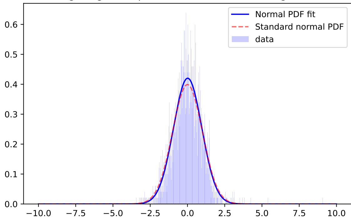
Whiten Signal, i-band, \mu=-0.0030 \sigma=0.9830 ; for mag=[21.0; 21.5]
