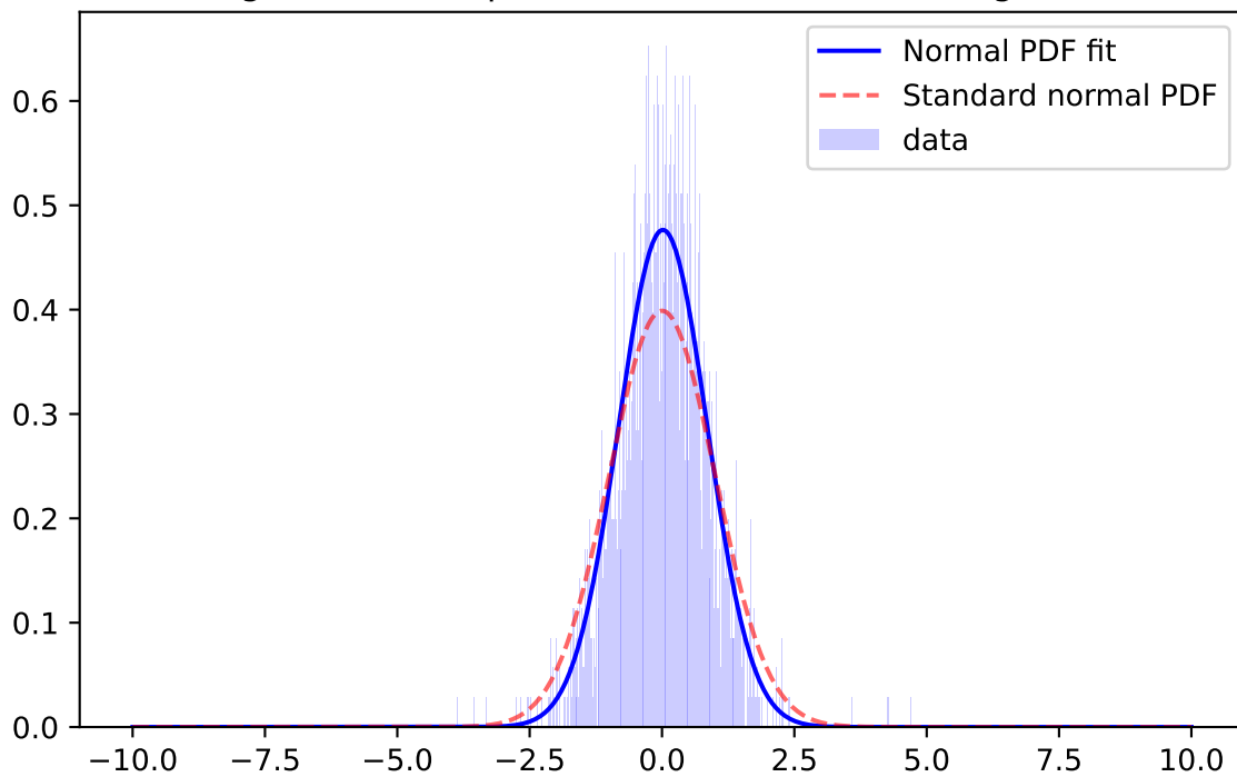
Whiten Signal, r-band, \mu=0.0074 \sigma=0.9963 ; for mag=[21.0; 21.5]
