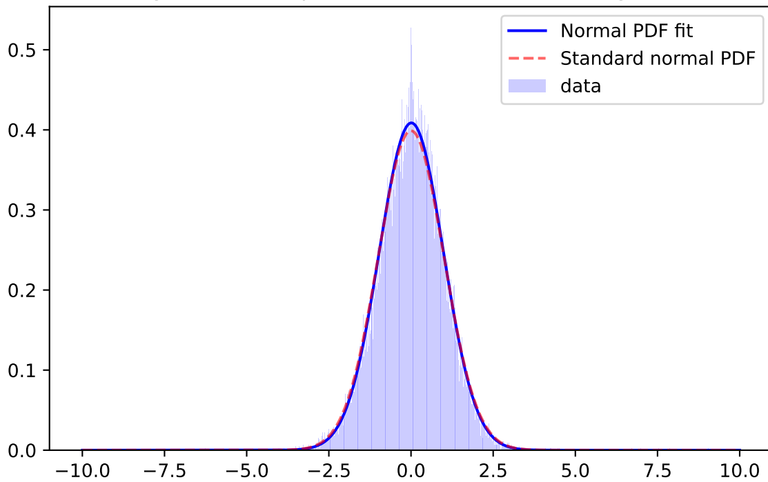
Whiten Signal, z-band, \mu=0.0102 \sigma=0.9761 ; for mag=[21.0; 21.5]
