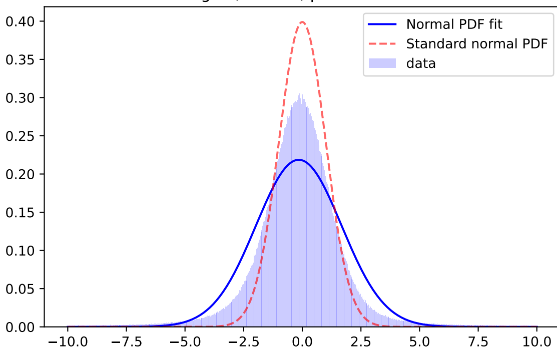
Whiten Signal, z-band, \mu=-0.1509 \sigma=1.8247
