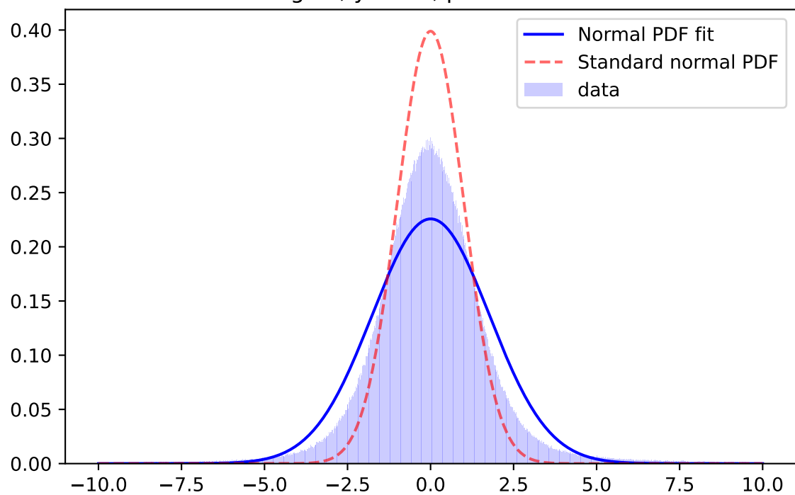
Whiten Signal, y-band, \mu=0.0048 \sigma=1.7671
