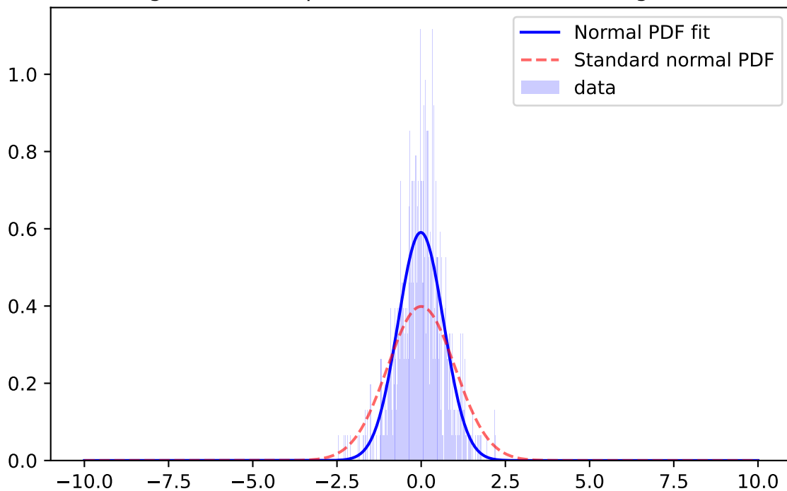
Whiten Signal, r-band, \mu=0.0669 \sigma=1.0819 ; for mag=[18.0; 18.5]
