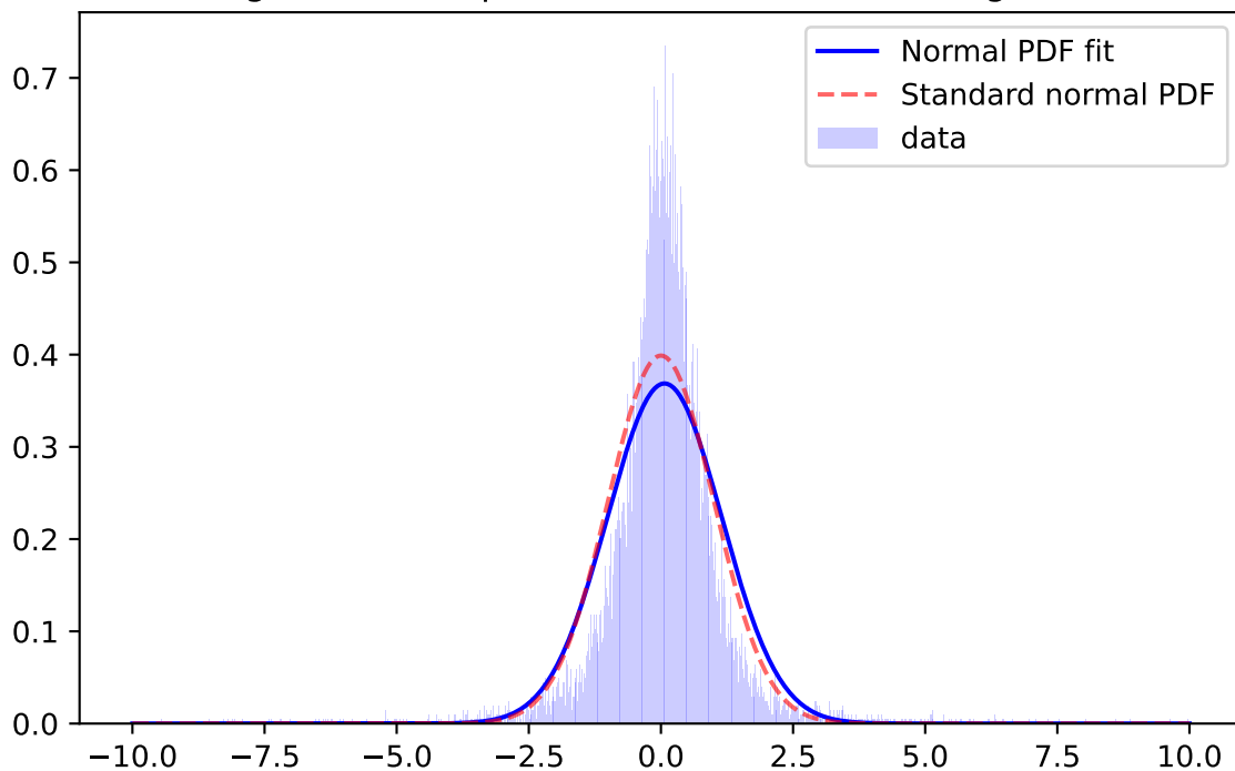
Whiten Signal, z-band, \mu=-0.0508 \sigma=1.0556 ; for mag=[18.0; 18.5]
