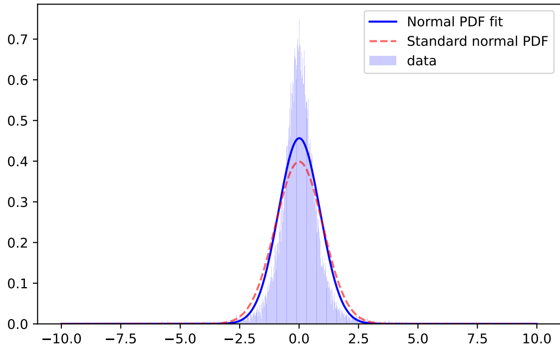
Whiten Signal, y-band, \mu=0.0080 \sigma=0.8738 ; for mag=[18.0; 18.5]
