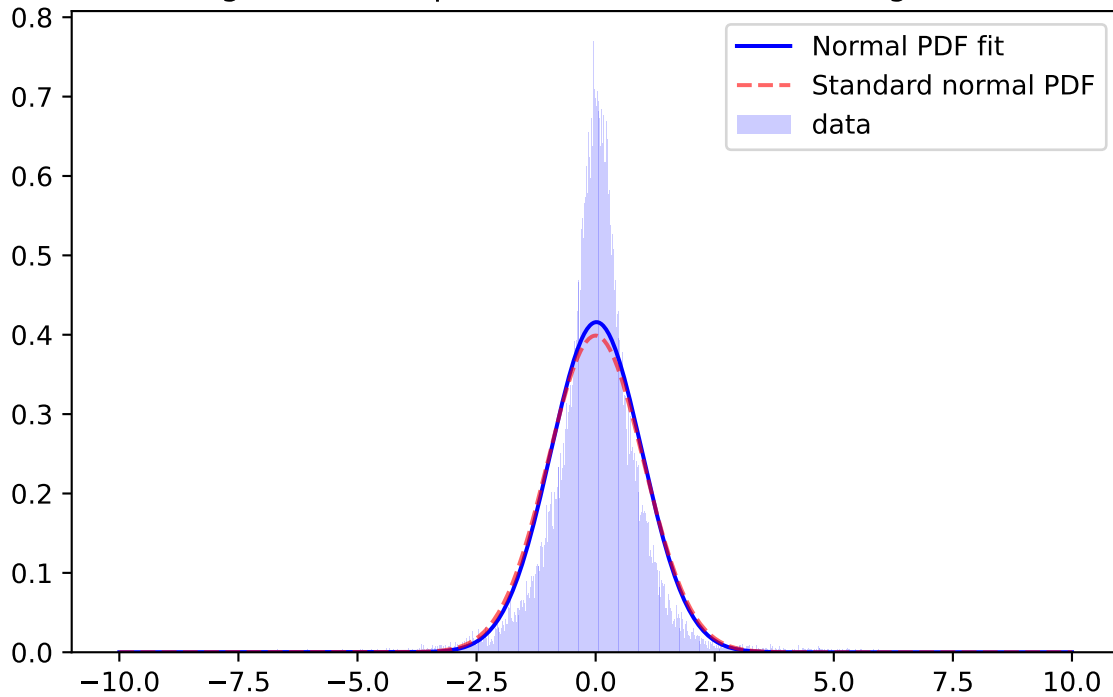
Whiten Signal, z-band, \mu=-0.0981 \sigma=1.0052 ; for mag=[21.0; 21.5]
