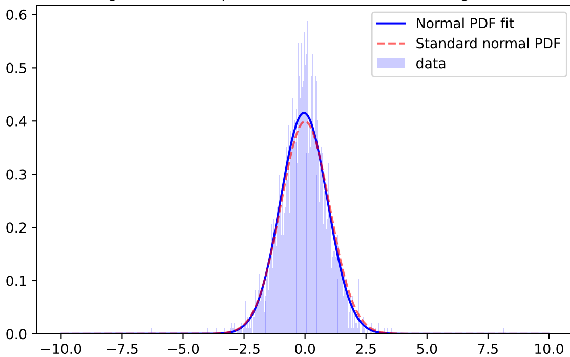
Whiten Signal, r-band, \mu=0.0169 \sigma=0.9592 ; for mag=[21.0; 21.5]
