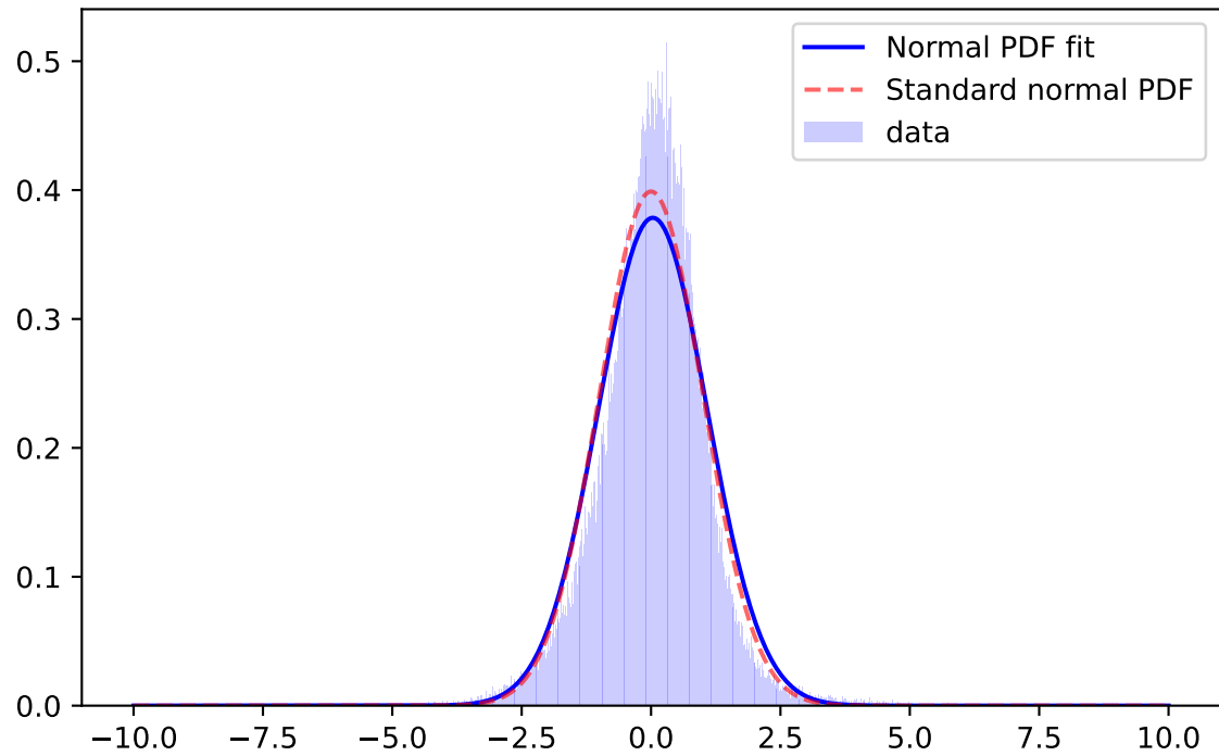
Whiten Signal, y-band, \mu=0.0337 \sigma=1.0539 ; for mag=[21.0; 21.5]
