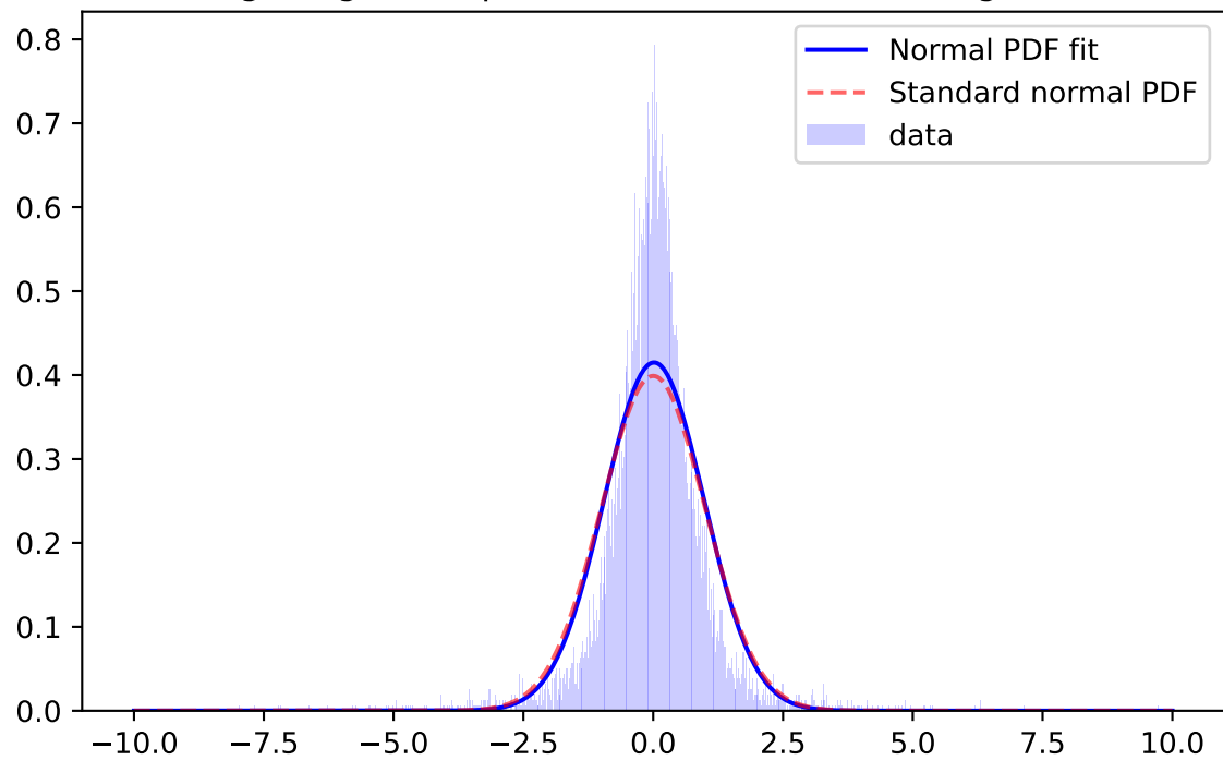
Whiten Signal, i-band, \mu=-0.0371 \sigma=0.9791 ; for mag=[21.0; 21.5]
