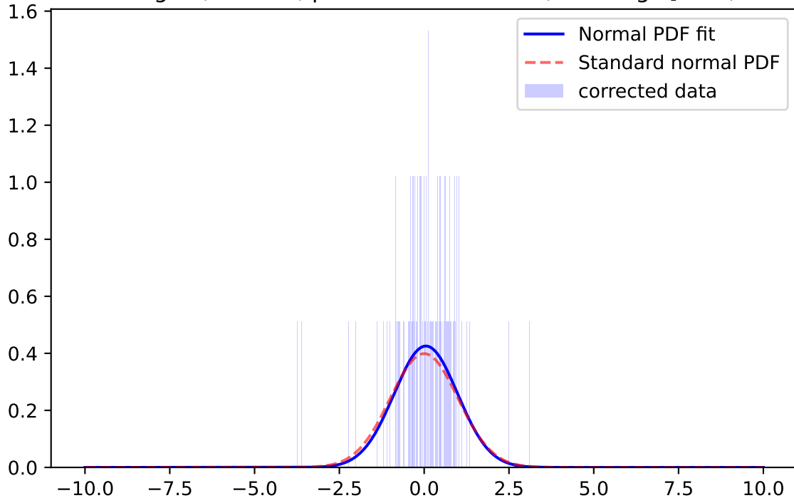
Whiten Signal, r-band, \mu=0.1009 \sigma=1.5409 ; for mag=[18.0; 18.5]
