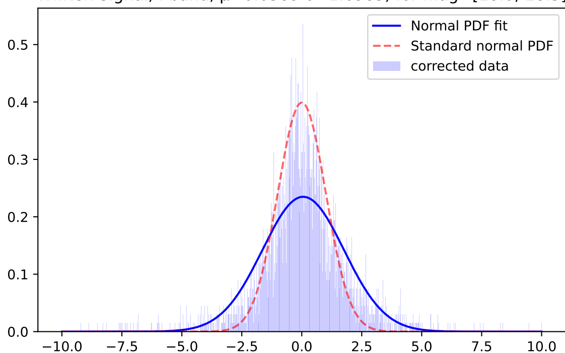
Whiten Signal, y-band, \mu=0.0592 \sigma=1.6023 ; for mag=[18.0; 18.5]
