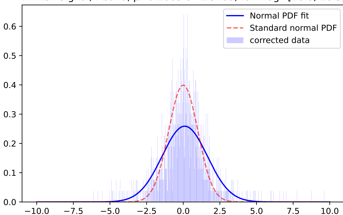
Whiten Signal, z-band, \mu=-0.0596 \sigma=1.7464 ; for mag=[18.0; 18.5]
