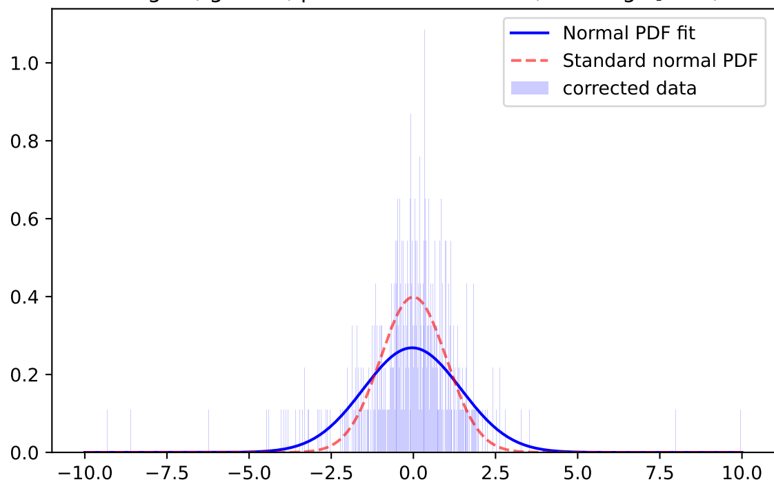
Whiten Signal, i-band, \mu=0.0589 \sigma=1.6985 ; for mag=[18.0; 18.5]
