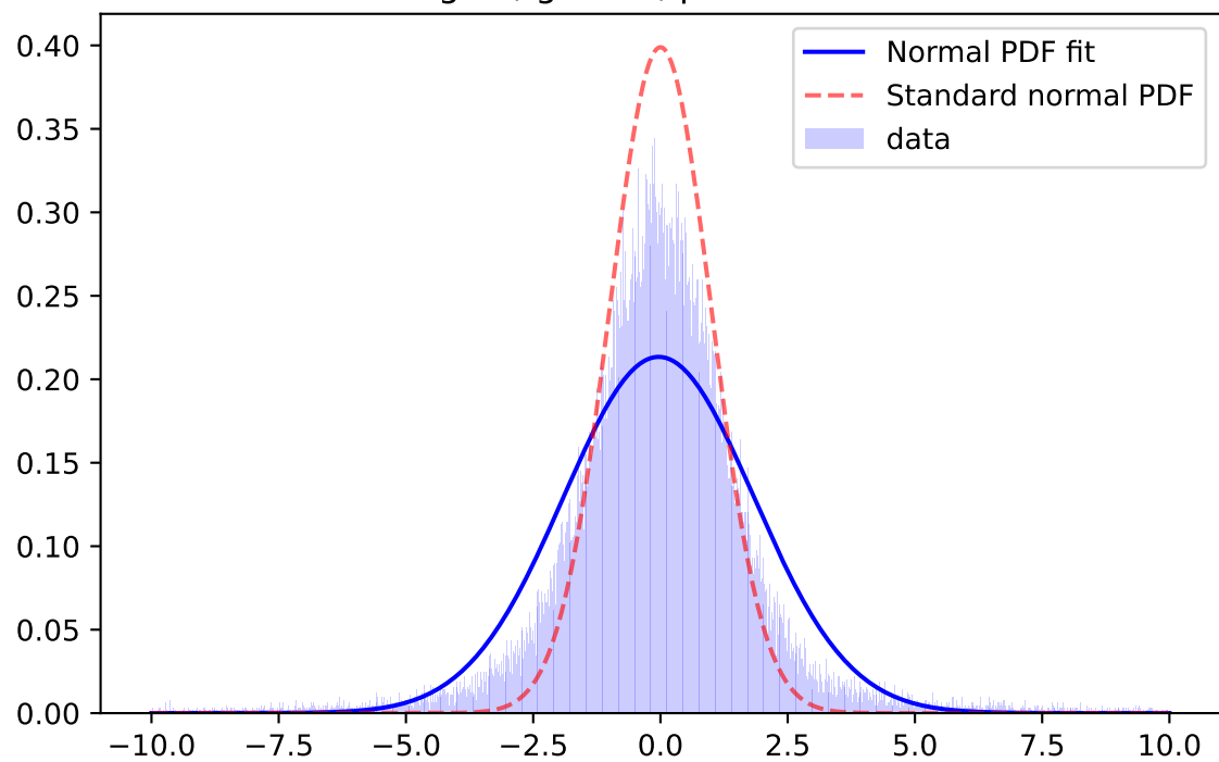
Whiten Signal, i-band, \mu=-0.1416 \sigma=2.0493
