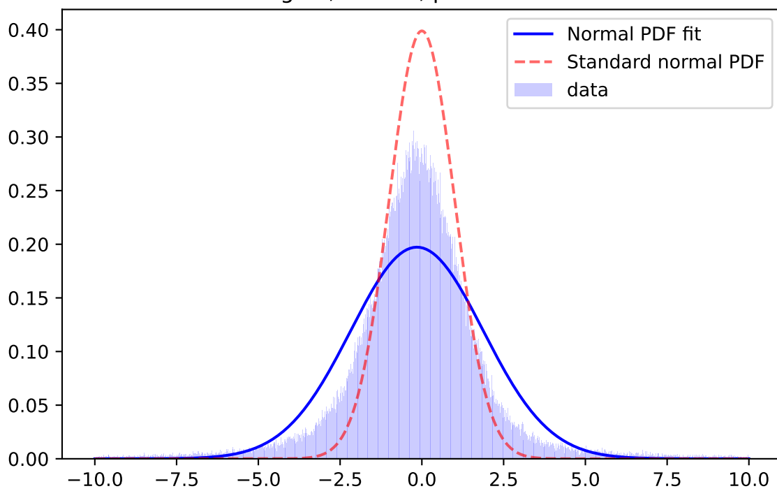
Whiten Signal, z-band, \mu=-0.1501 \sigma=2.0221
