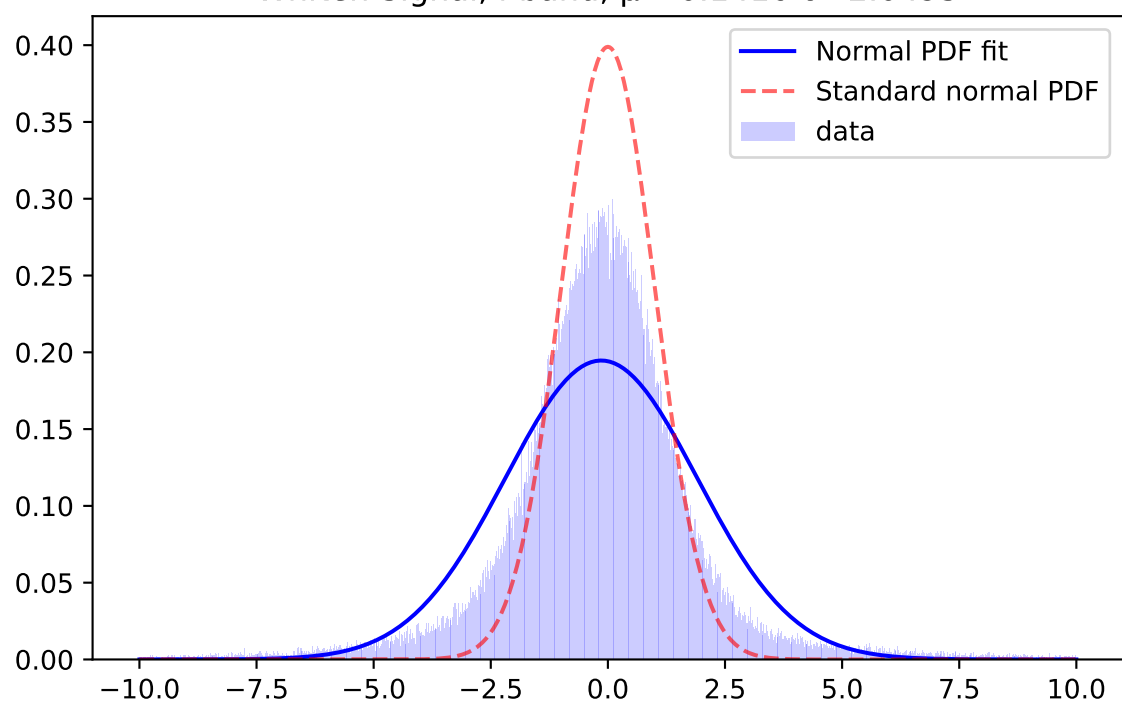
Whiten Signal, y-band, \mu=0.0187 \sigma=1.8619
