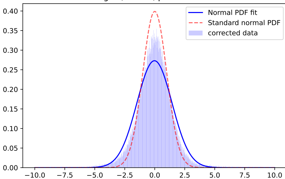
Whiten Signal, z-band, \mu=-0.1345 \sigma=1.4988
