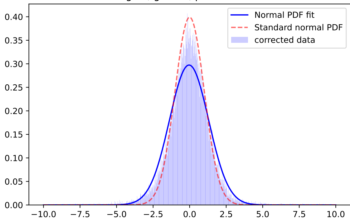
Whiten Signal, i-band, \mu=-0.1329 \sigma=1.5462
