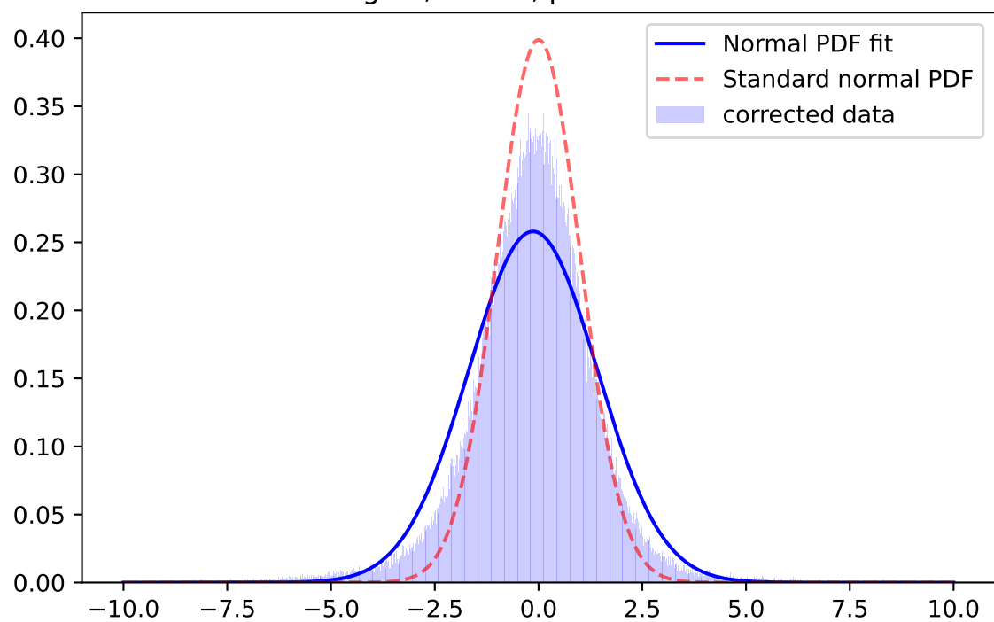
Whiten Signal, y-band, \mu=0.0082 \sigma=1.5138
