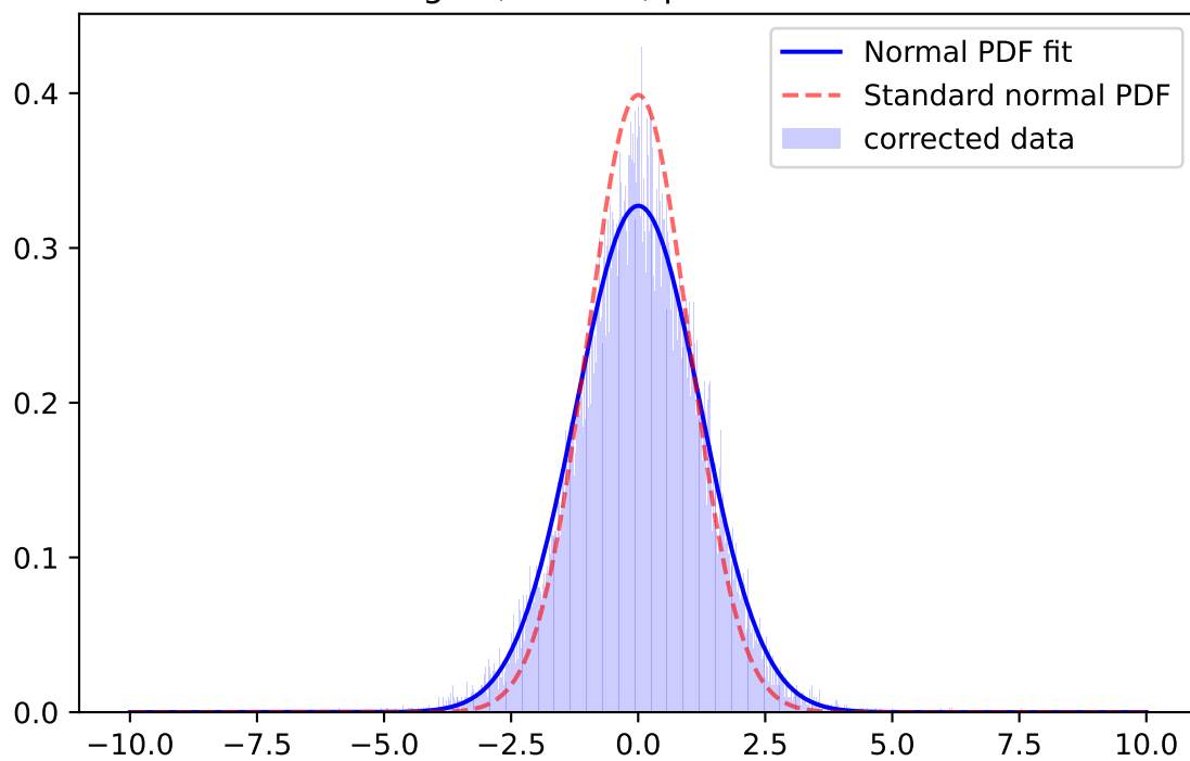
Whiten Signal, r-band, \mu=-0.0237 \sigma=1.4612
