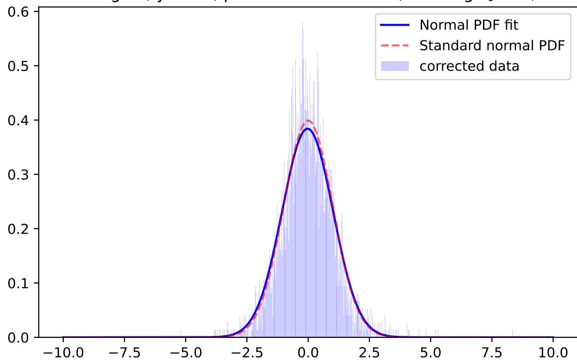
Whiten Signal, y-band, \mu=-0.0238 \sigma=1.0389 ; for mag=[18.0; 18.5]
