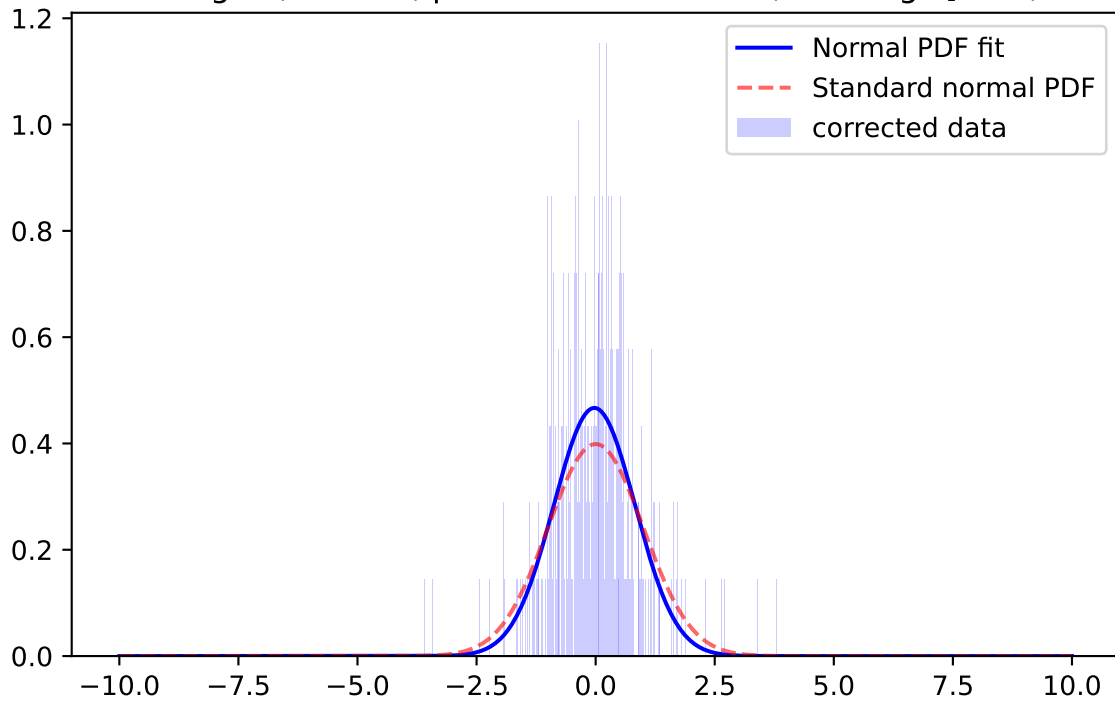
Whiten Signal, r-band, \mu=-0.0283 \sigma=0.9135 ; for mag=[18.0; 18.5]
