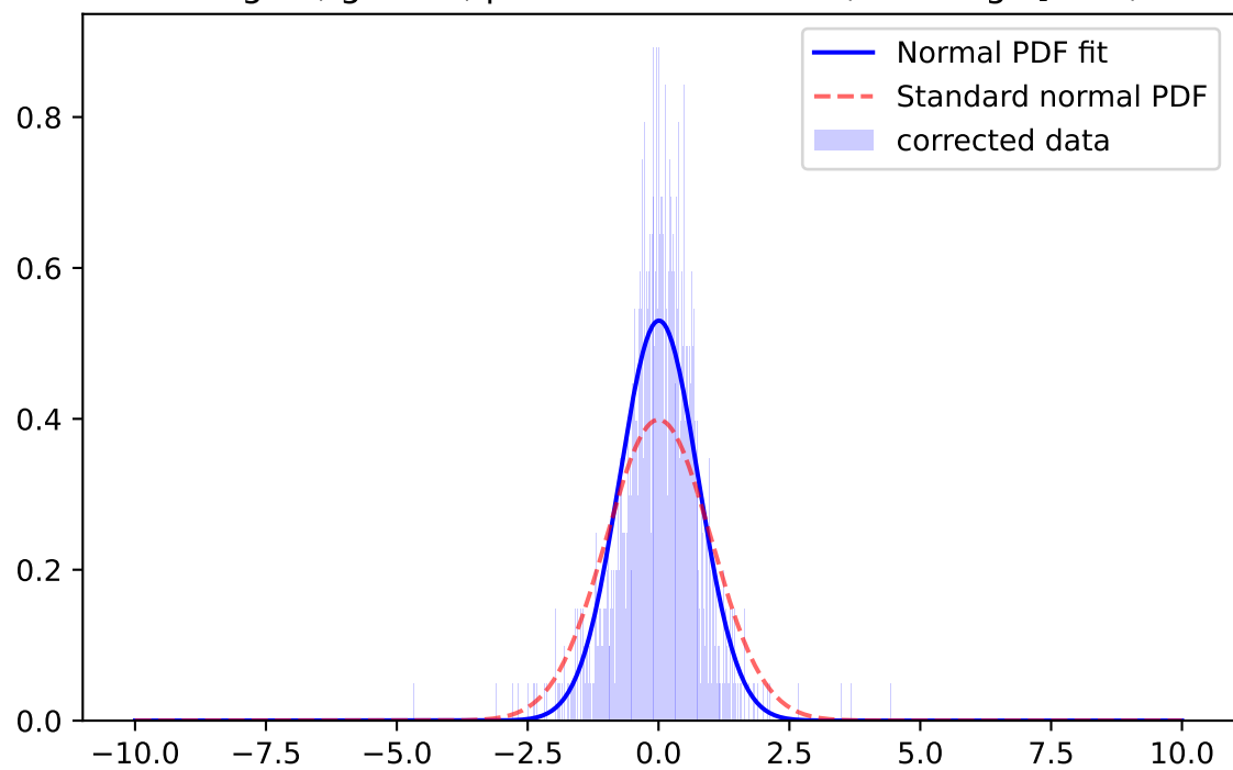
Whiten Signal, i-band, \mu=-0.0243 \sigma=1.1422 ; for mag=[18.0; 18.5]
