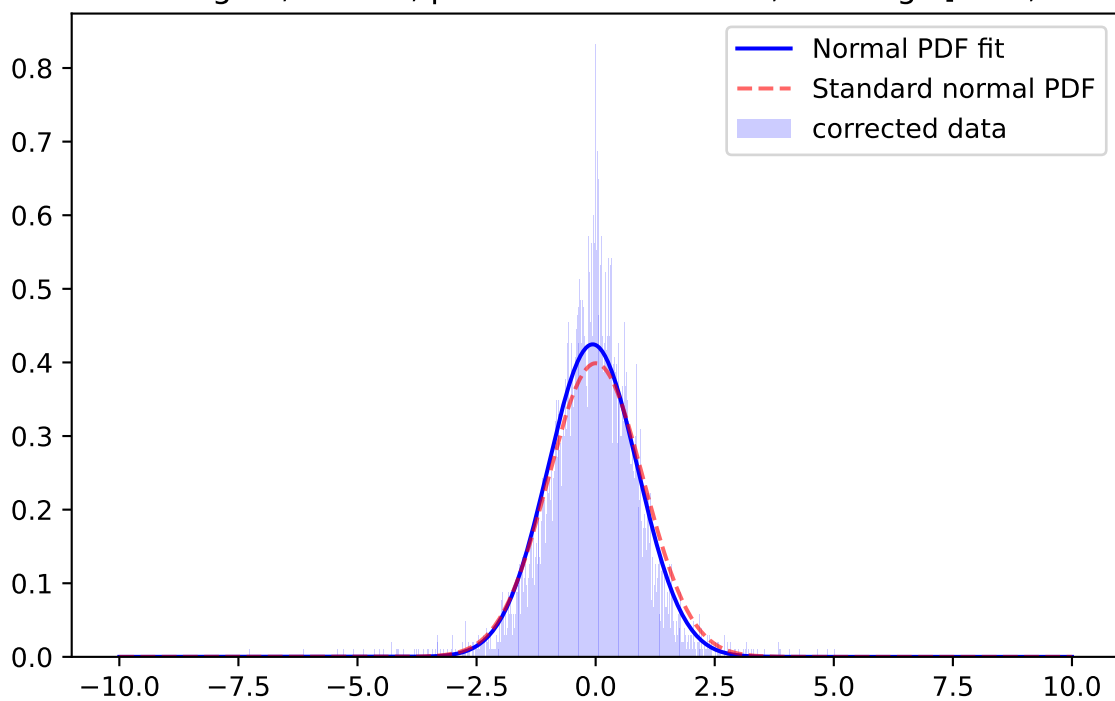
Whiten Signal, z-band, \mu=-0.0619 \sigma=0.9395 ; for mag=[18.0; 18.5]
