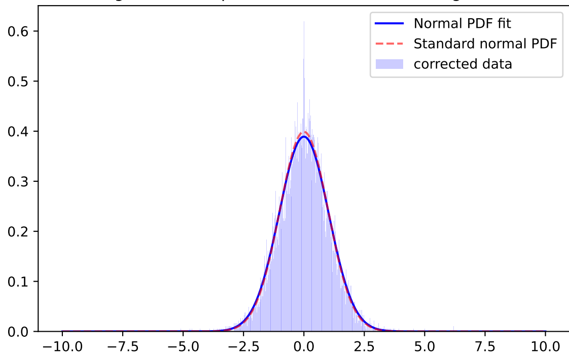
Whiten Signal, y-band, \mu=0.0295 \sigma=1.0576 ; for mag=[21.0; 21.5]
