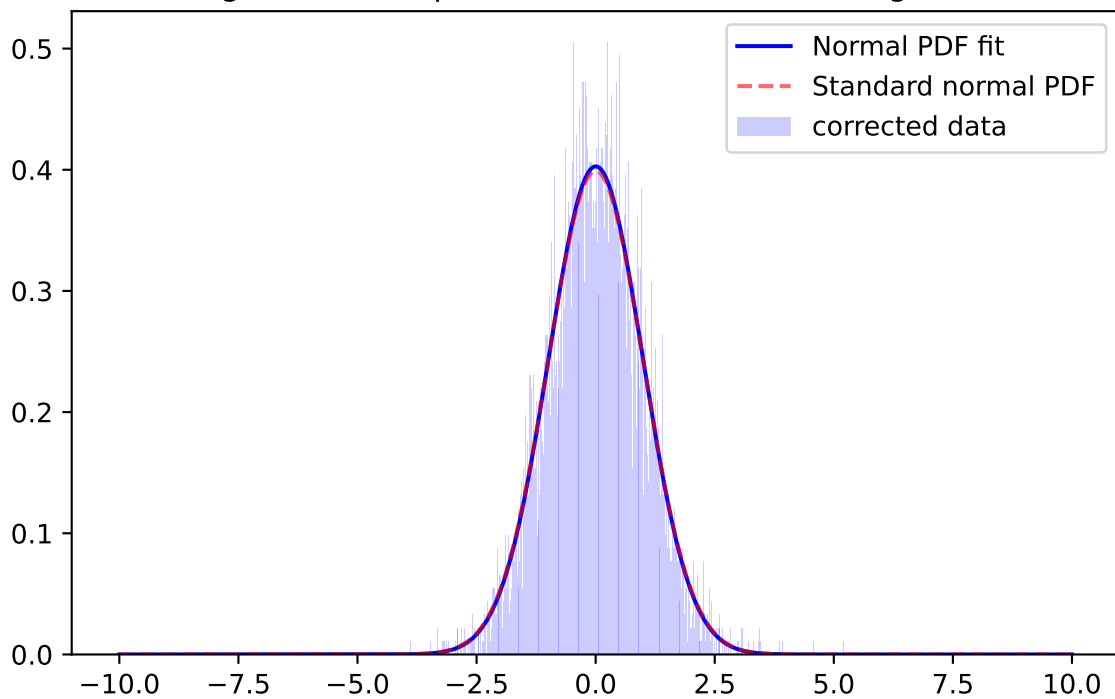
Whiten Signal, z-band, \mu=-0.0081 \sigma=0.9824 ; for mag=[21.0; 21.5]
