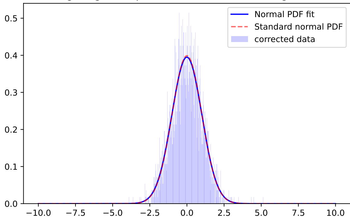
Whiten Signal, i-band, \mu=0.0003 \sigma=1.0252 ; for mag=[21.0; 21.5]
