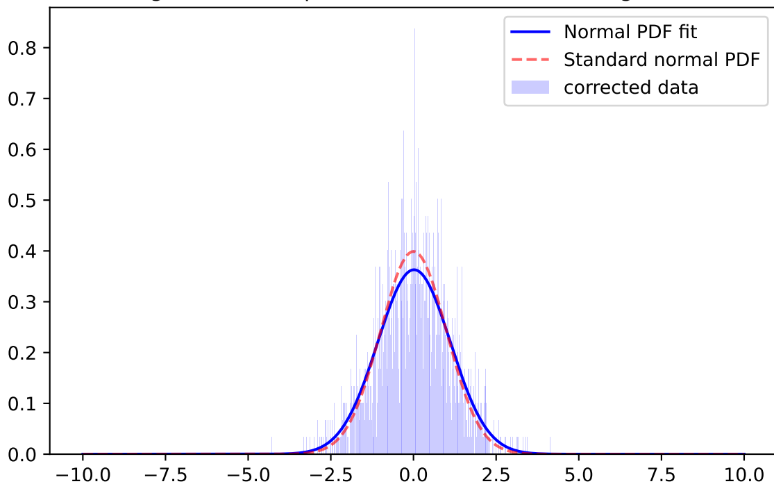
Whiten Signal, r-band, \mu=0.0014 \sigma=0.9903 ; for mag=[21.0; 21.5]
