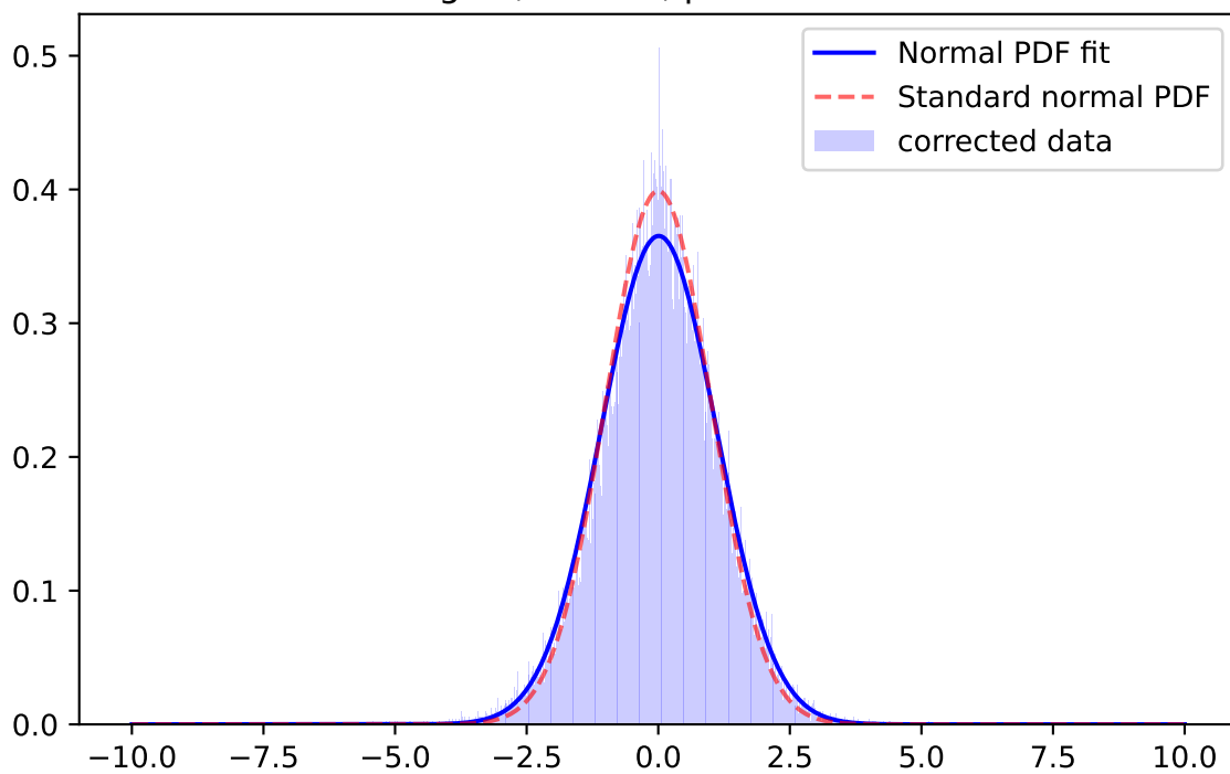
Whiten Signal, r-band, \mu=0.0019 \sigma=0.9946
