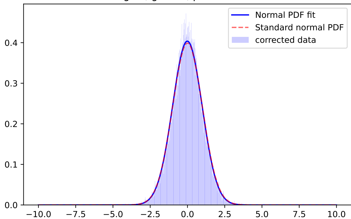
Whiten Signal, i-band, \mu=-0.0066 \sigma=1.0369
