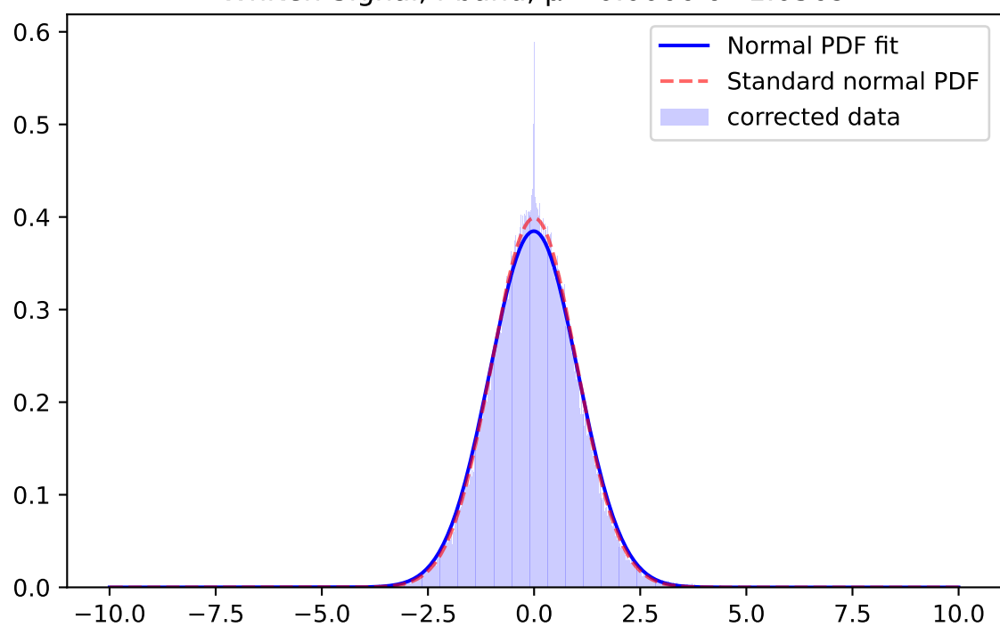
Whiten Signal, y-band, \mu=-0.0014 \sigma=1.0354
