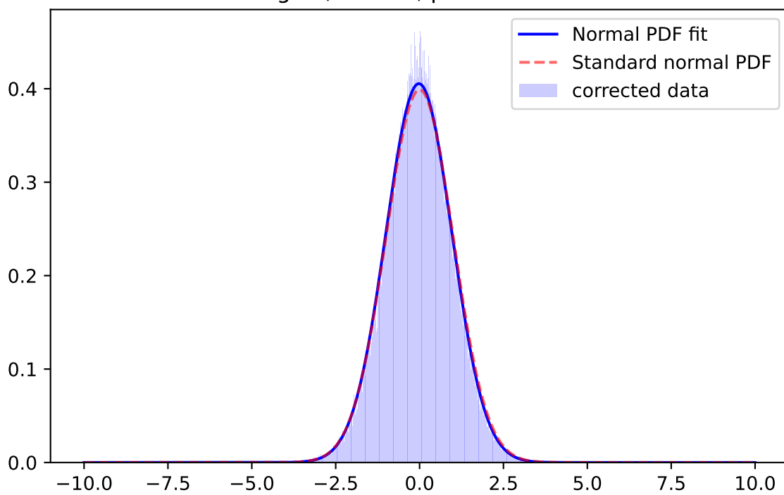
Whiten Signal, z-band, \mu=-0.0207 \sigma=0.9839
