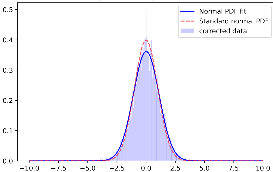
Whiten Signal, r-band, \mu=0.0014 \sigma=1.0101
