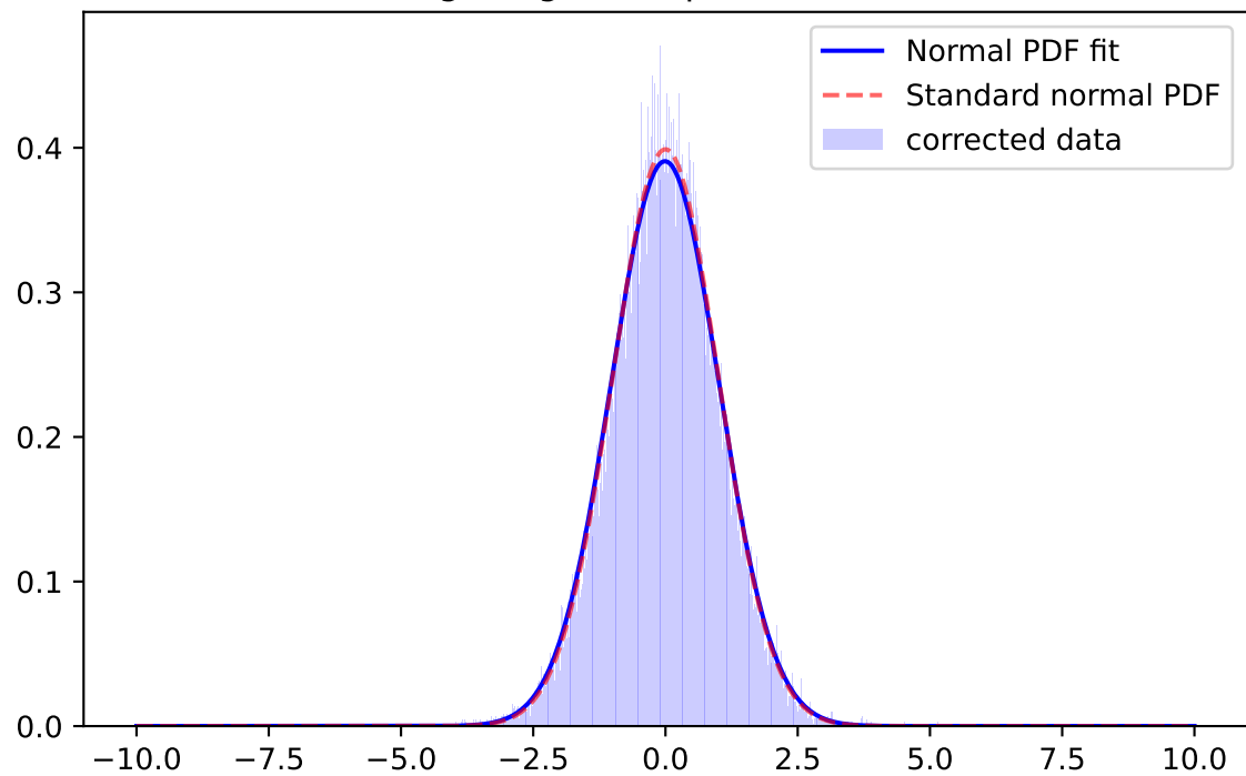
Whiten Signal, i-band, \mu=-0.0072 \sigma=1.0506
