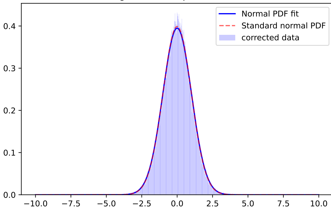
Whiten Signal, z-band, \mu=-0.0220 \sigma=1.0032
