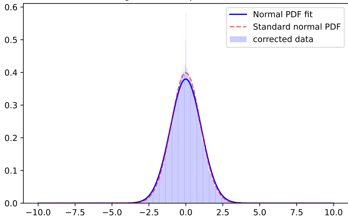
Whiten Signal, y-band, \mu=-0.0018 \sigma=1.0470
