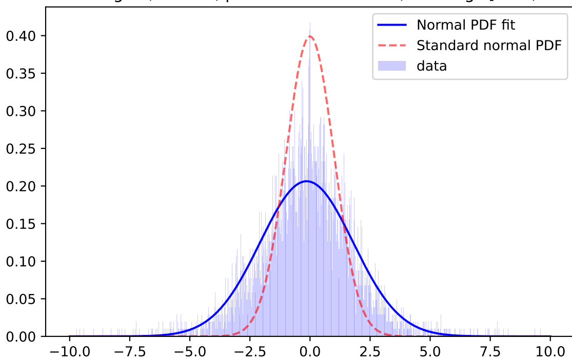
Whiten Signal, z-band, \mu=-0.1410 \sigma=1.9334 ; for mag=[18.0; 18.5]
