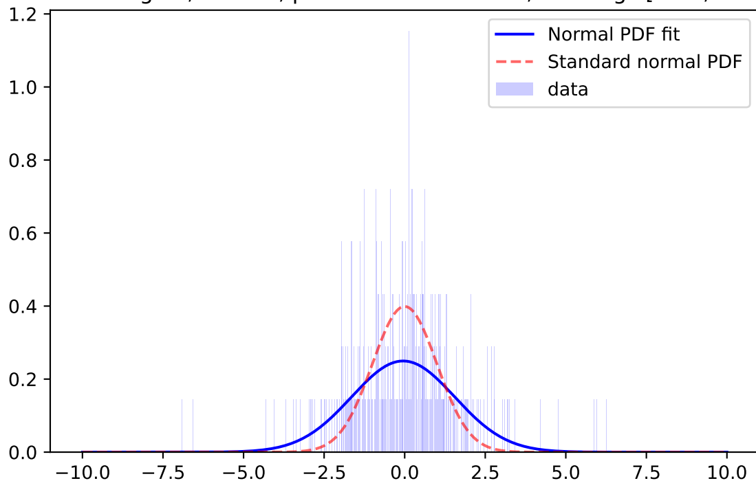
Whiten Signal, r-band, \mu=-0.1869 \sigma=2.8361 ; for mag=[18.0; 18.5]
