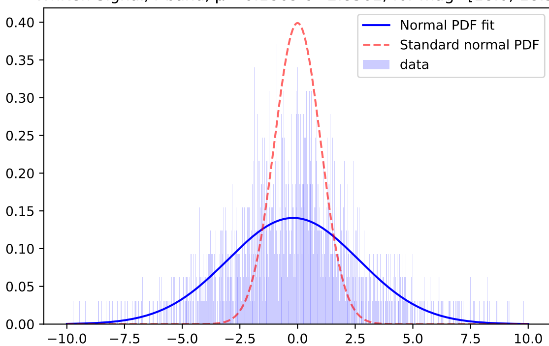
Whiten Signal, z-band, \mu=-0.1410 \sigma=1.9334 ; for mag=[18.0; 18.5]
