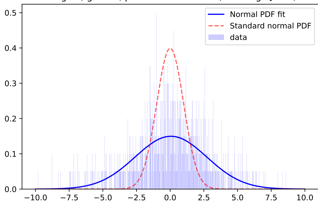
Whiten Signal, i-band, \mu=-0.1600 \sigma=2.7990 ; for mag=[18.0; 18.5]
