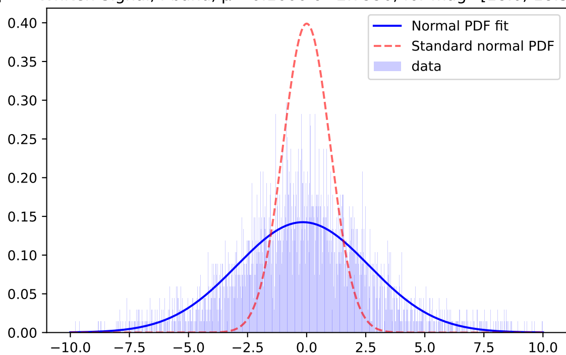
Whiten Signal, y-band, \mu=-0.0397 \sigma=1.4196 ; for mag=[18.0; 18.5]
