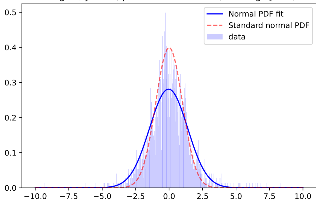
Whiten Signal, y-band, \mu=-0.0397 \sigma=1.4196 ; for mag=[18.0; 18.5]
