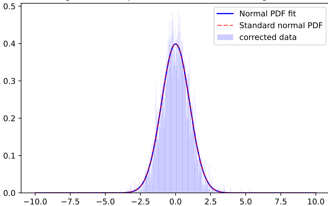
Whiten Signal, z-band, \mu=-0.0083 \sigma=0.9838 ; for mag=[21.0; 21.5]
