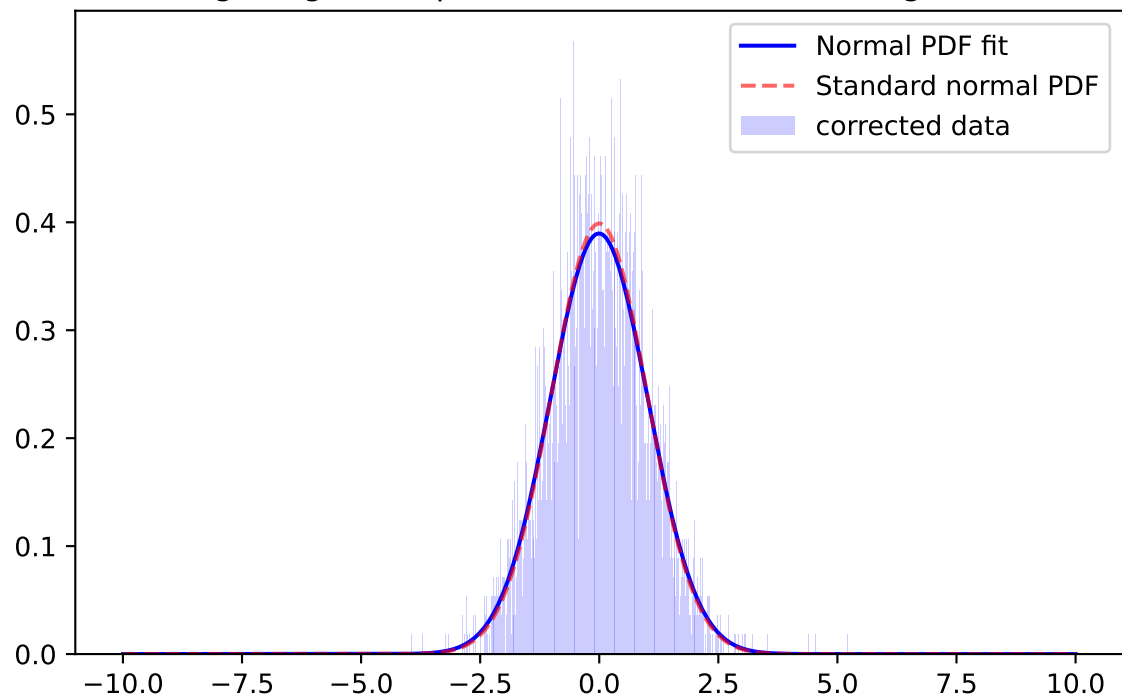
Whiten Signal, i-band, \mu=0.0003 \sigma=1.0261 ; for mag=[21.0; 21.5]
