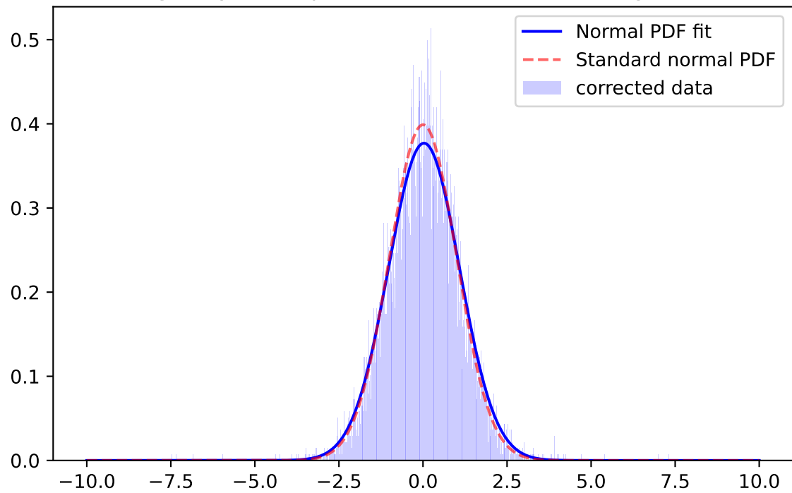
Whiten Signal, y-band, \mu=0.0294 \sigma=1.0581 ; for mag=[21.0; 21.5]
