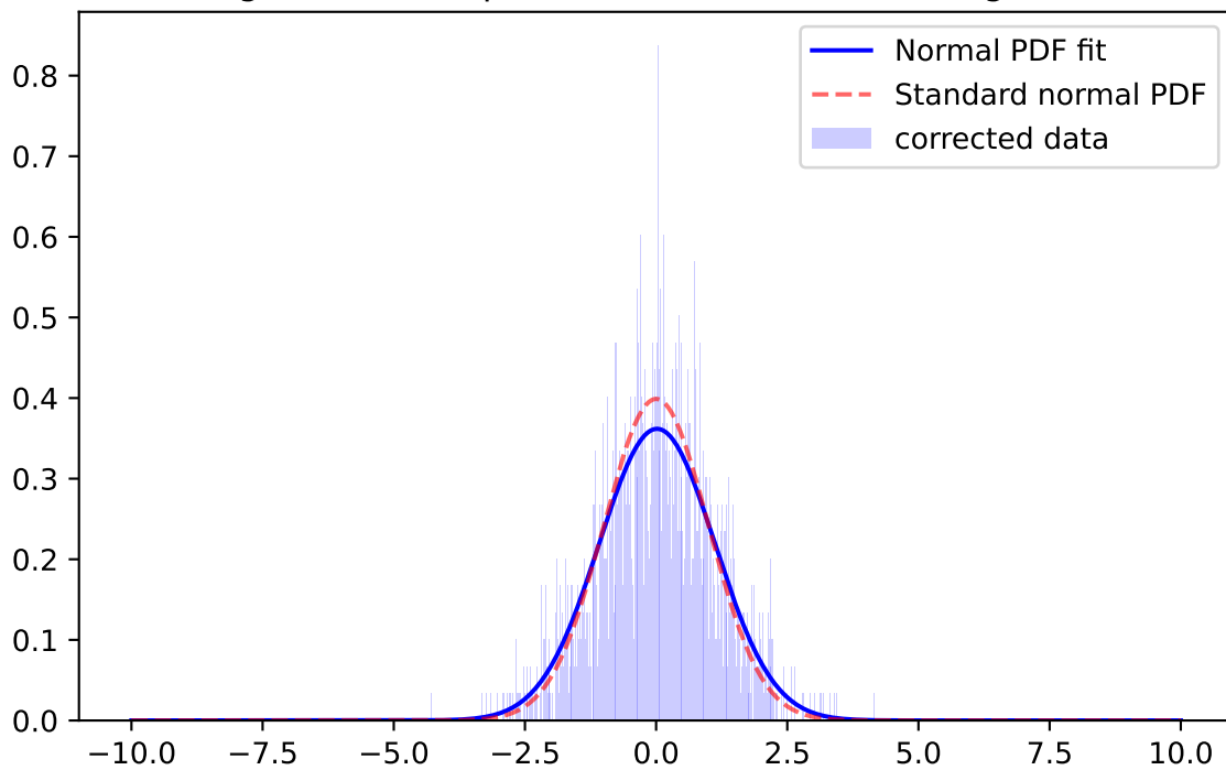
Whiten Signal, r-band, \mu=0.0013 \sigma=0.9999 ; for mag=[21.0; 21.5]
