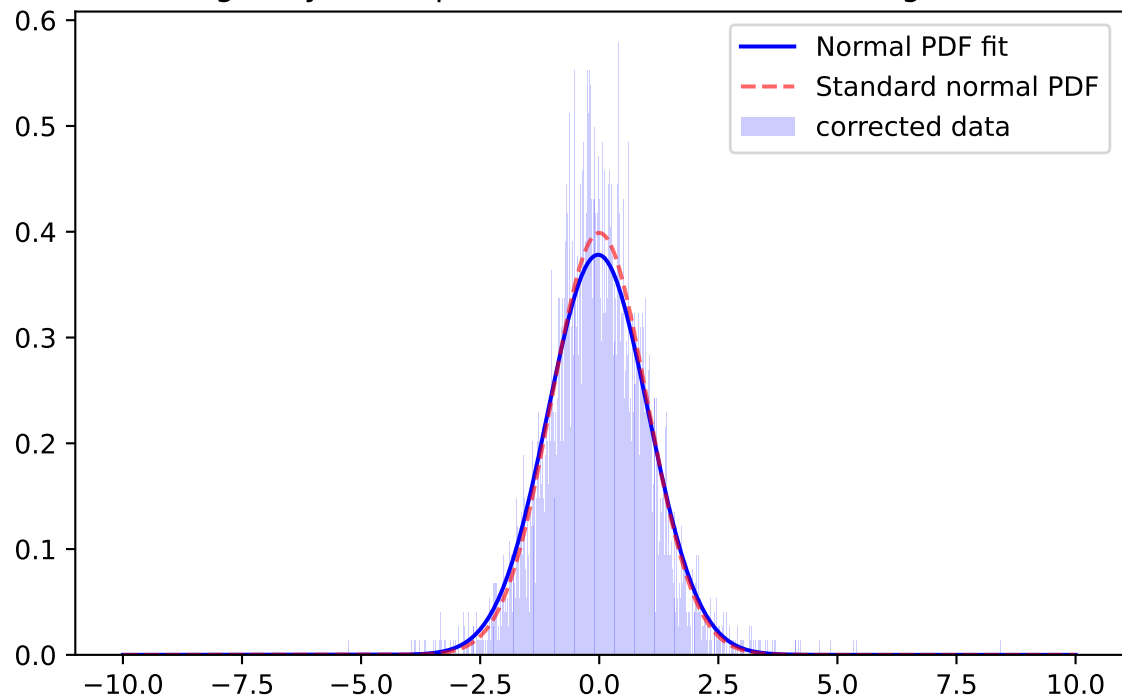
Whiten Signal, y-band, \mu=-0.0245 \sigma=1.0547 ; for mag=[18.0; 18.5]
