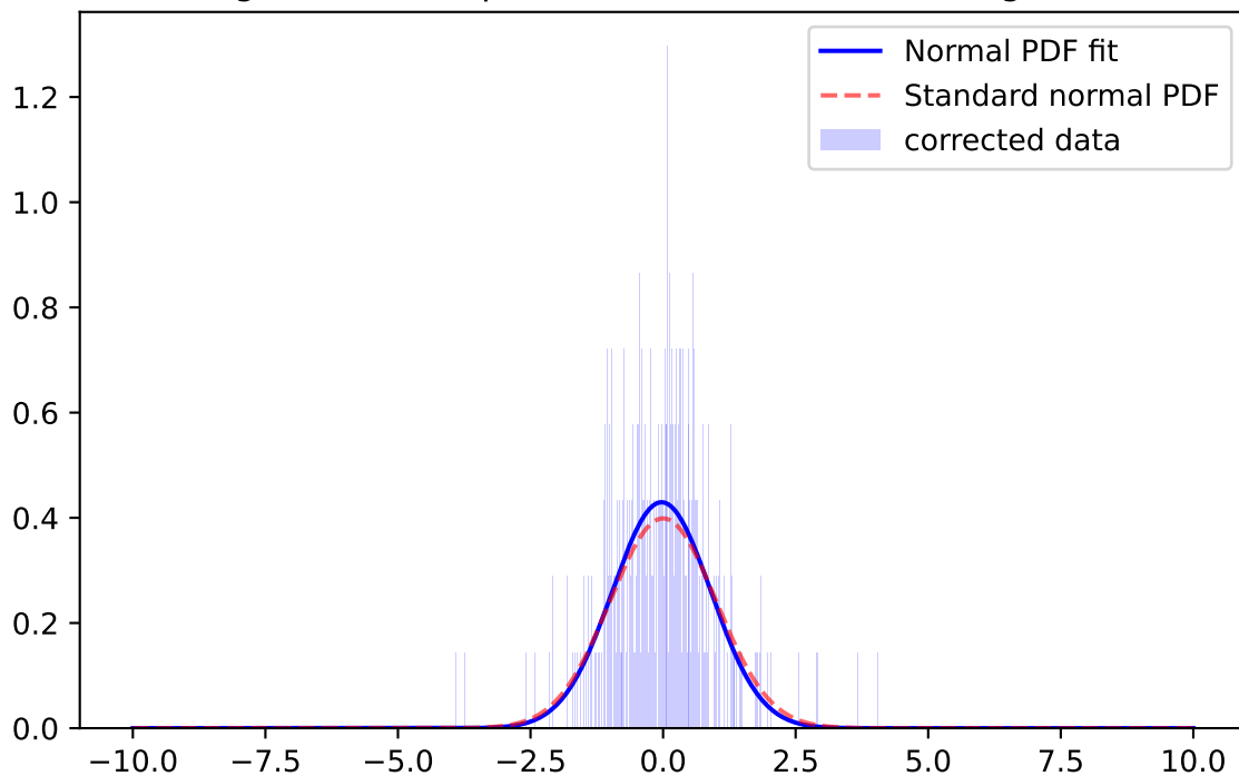
Whiten Signal, r-band, \mu=-0.0301 \sigma=0.9601 ; for mag=[18.0; 18.5]
