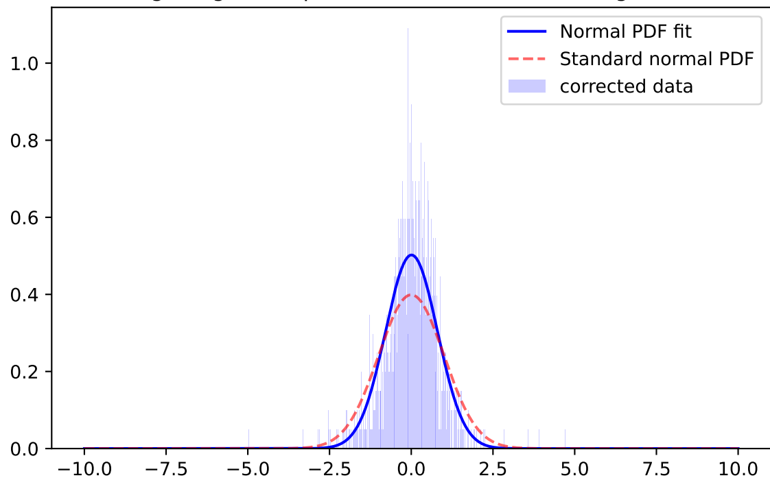
Whiten Signal, i-band, \mu=-0.0243 \sigma=1.1500 ; for mag=[18.0; 18.5]
