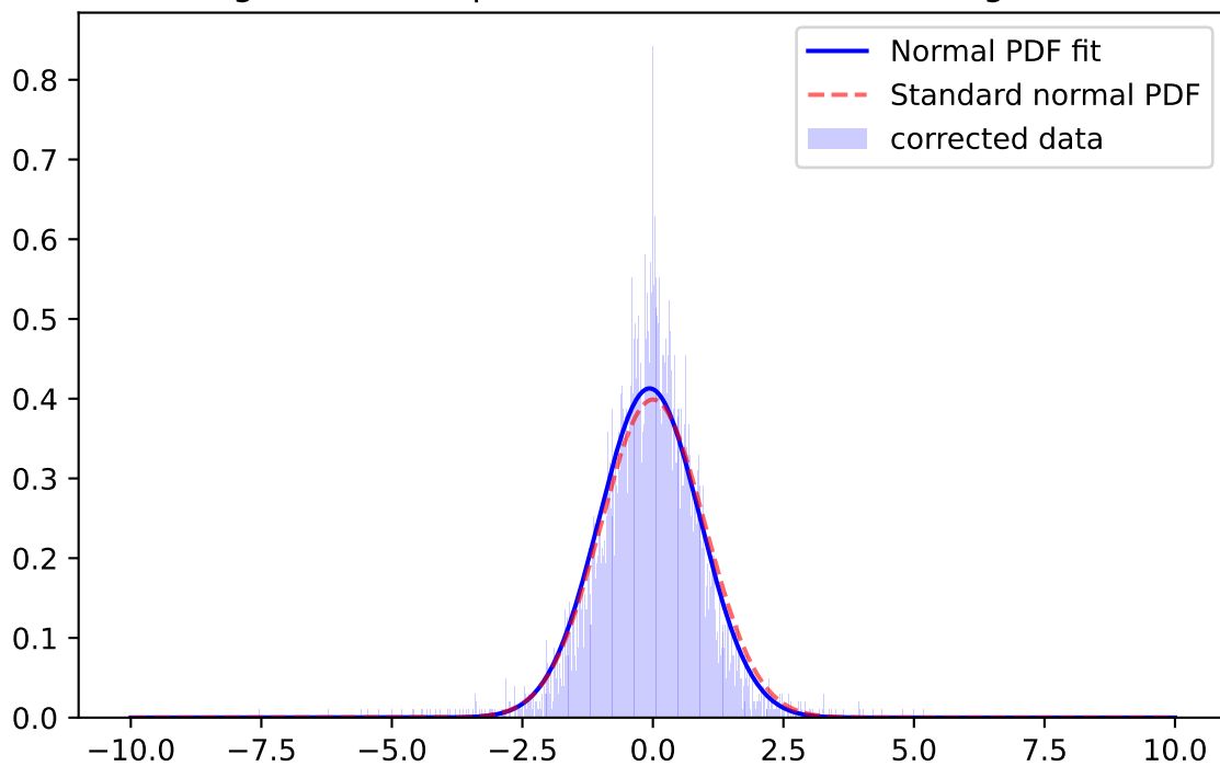
Whiten Signal, z-band, \mu=-0.0640 \sigma=0.9662 ; for mag=[18.0; 18.5]
