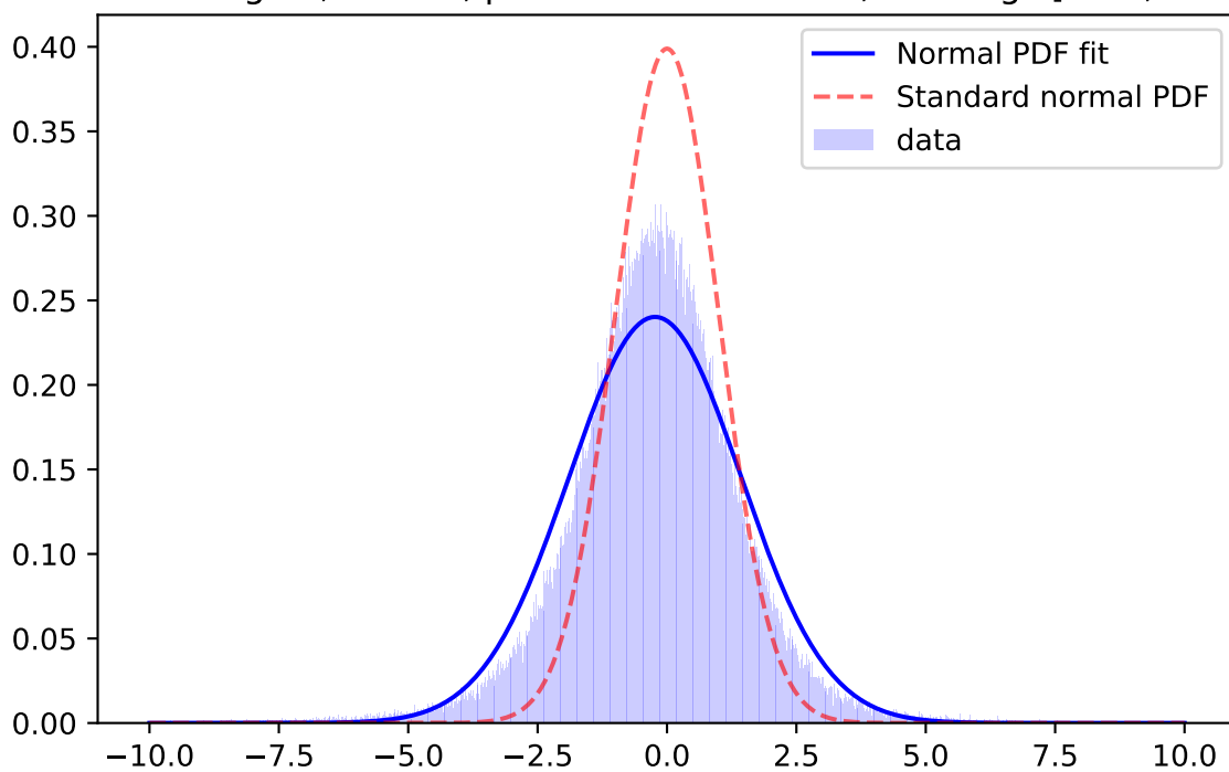
Whiten Signal, z-band, \mu=-0.2312 \sigma=1.6607 ; for mag=[21.0; 21.5]
