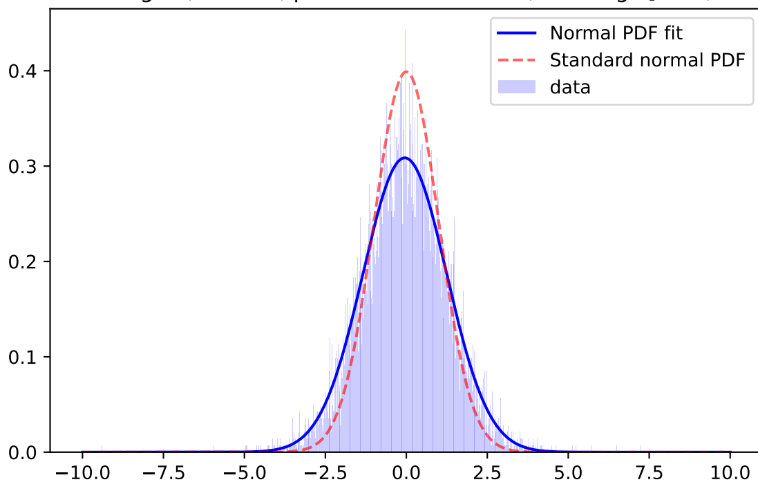
Whiten Signal, r-band, \mu=-0.0086 \sigma=2.2147 ; for mag=[21.0; 21.5]
