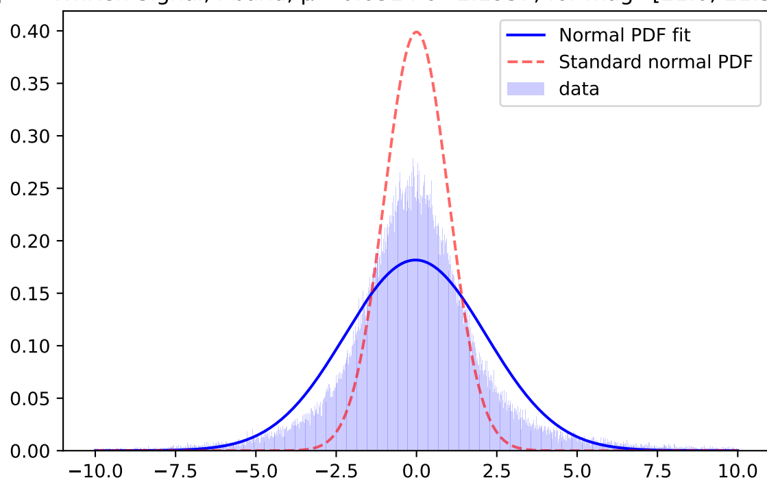
Whiten Signal, y-band, \mu=-0.0220 \sigma=1.5745 ; for mag=[21.0; 21.5]
