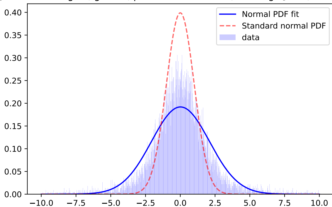
Whiten Signal, i-band, \mu=-0.0314 \sigma=2.1957 ; for mag=[21.0; 21.5]
