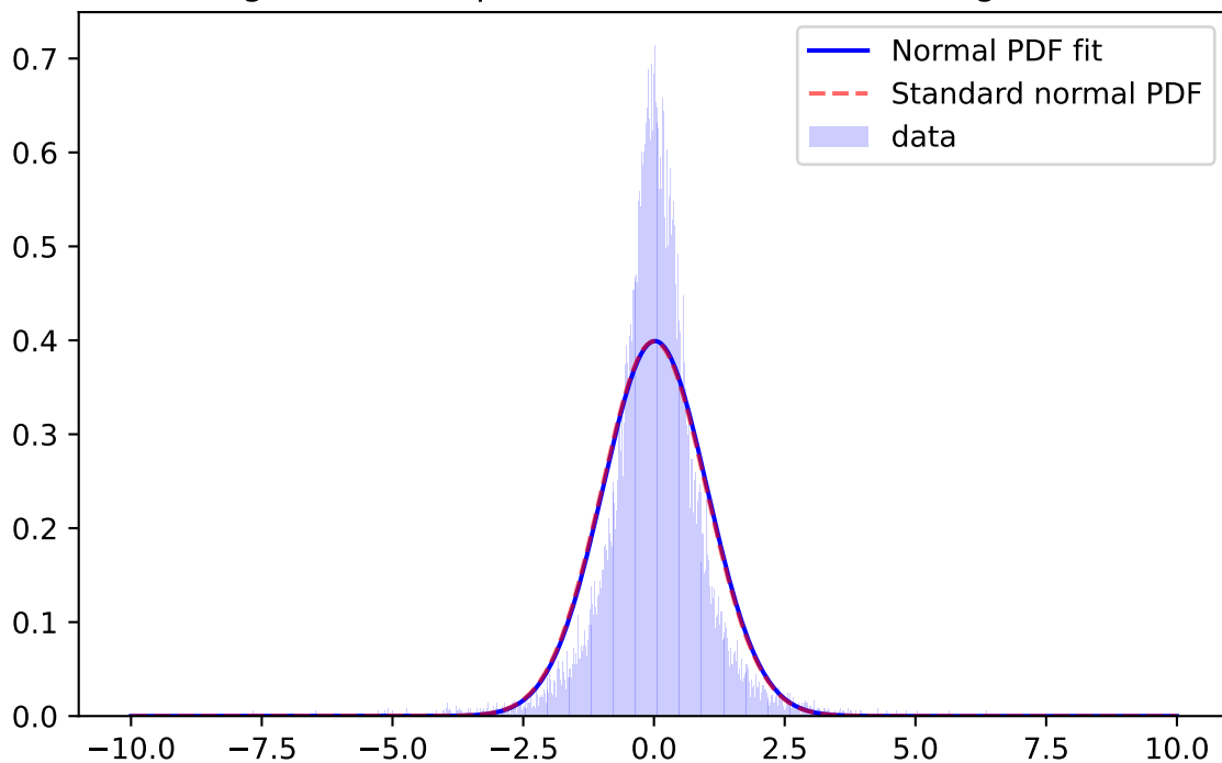
Whiten Signal, z-band, \mu=0.0320 \sigma=1.0975 ; for mag=[18.0; 18.5]
