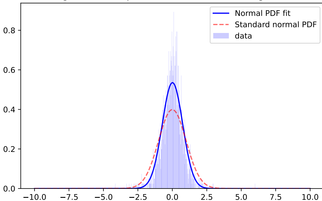
Whiten Signal, r-band, \mu=0.0196 \sigma=0.9992 ; for mag=[18.0; 18.5]
