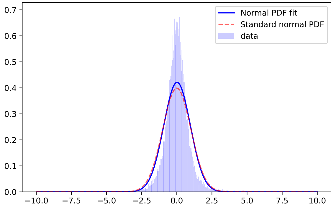
Whiten Signal, y-band, \mu=0.0197 \sigma=0.9471 ; for mag=[18.0; 18.5]
