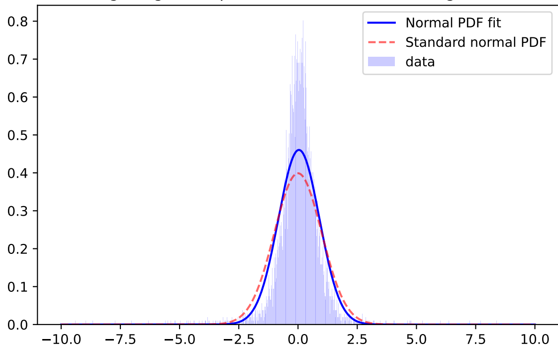
Whiten Signal, i-band, \mu=0.0367 \sigma=1.0259 ; for mag=[18.0; 18.5]
