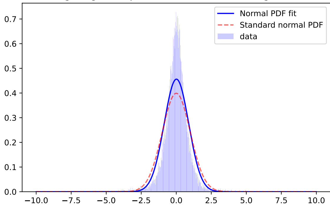
Whiten Signal, i-band, \mu=0.0203 \sigma=1.0561 ; for mag=[21.0; 21.5]
