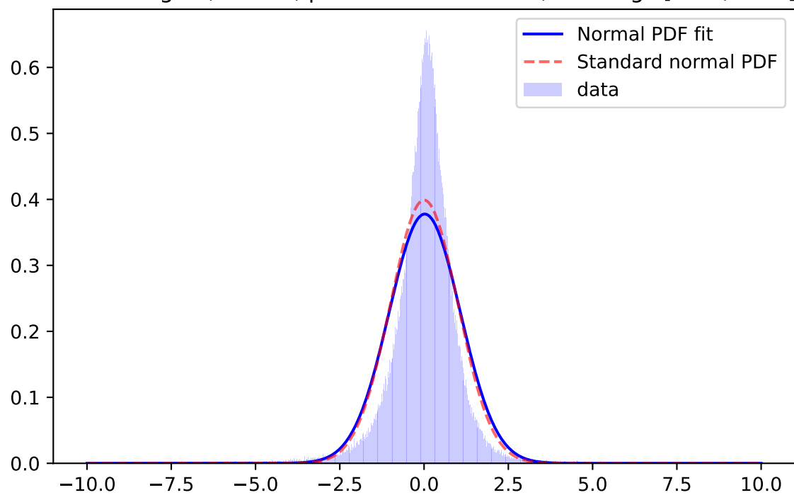
Whiten Signal, y-band, \mu=0.0130 \sigma=1.0449 ; for mag=[21.0; 21.5]
