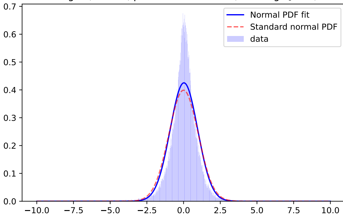
Whiten Signal, z-band, \mu=-0.0161 \sigma=1.0445 ; for mag=[21.0; 21.5]
