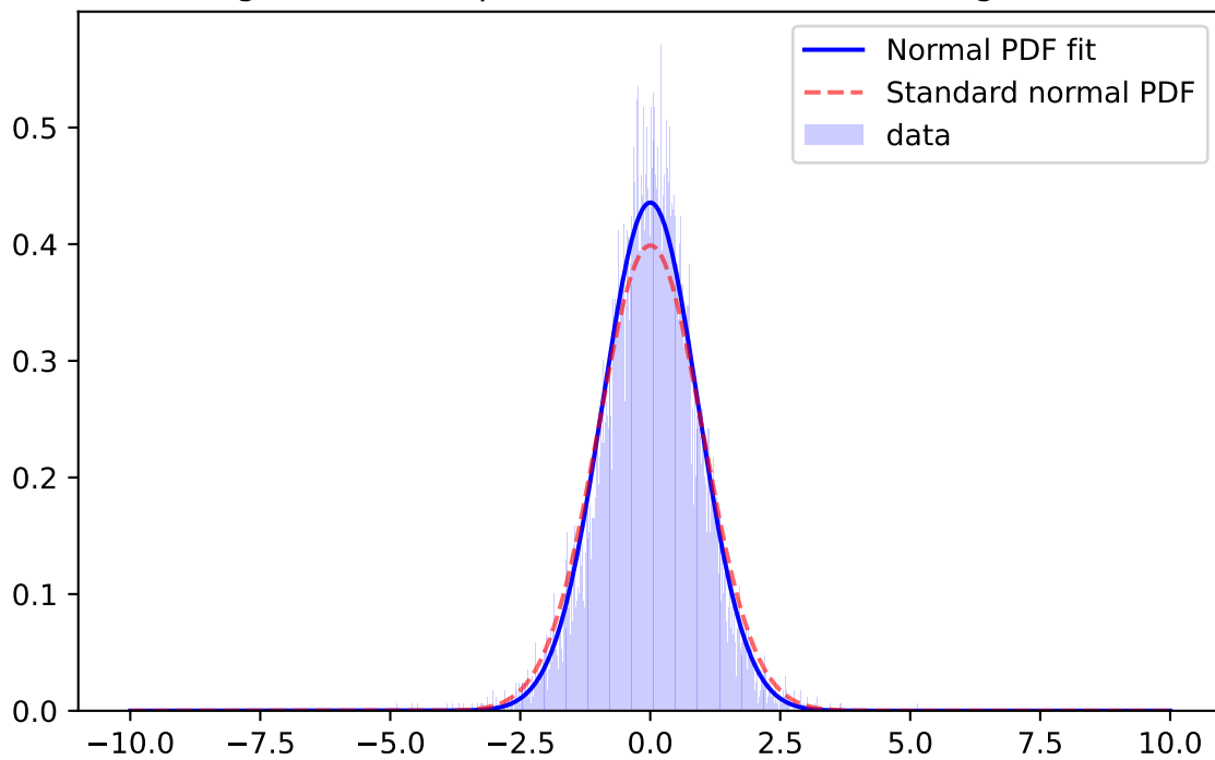
Whiten Signal, r-band, \mu=0.0247 \sigma=0.9380 ; for mag=[21.0; 21.5]
