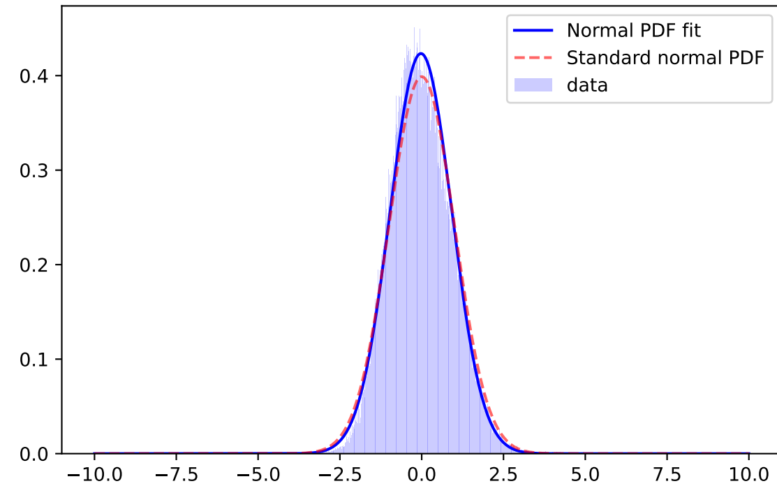
Whiten Signal, z-band, \mu=-0.0232 \sigma=0.9421 ; for mag=[25.0; 25.5]
