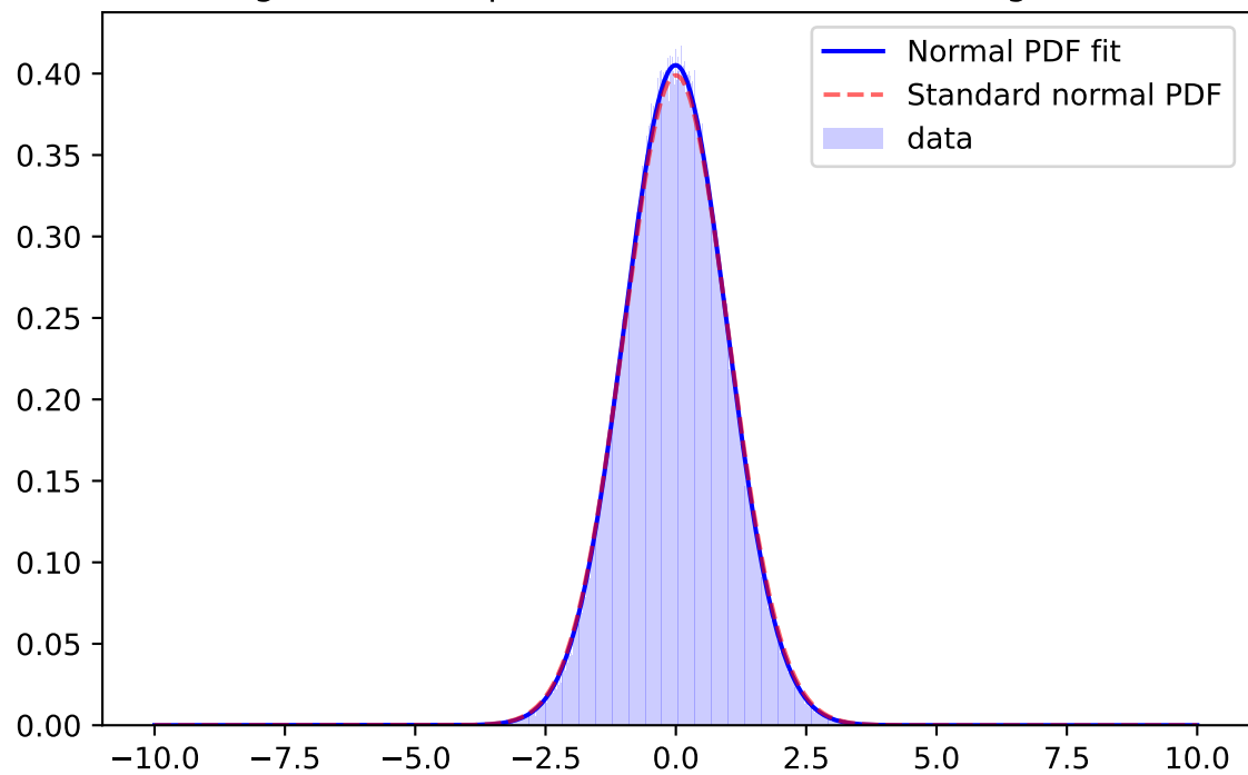
Whiten Signal, y-band, \mu=-0.0444 \sigma=0.9001 ; for mag=[25.0; 25.5]
