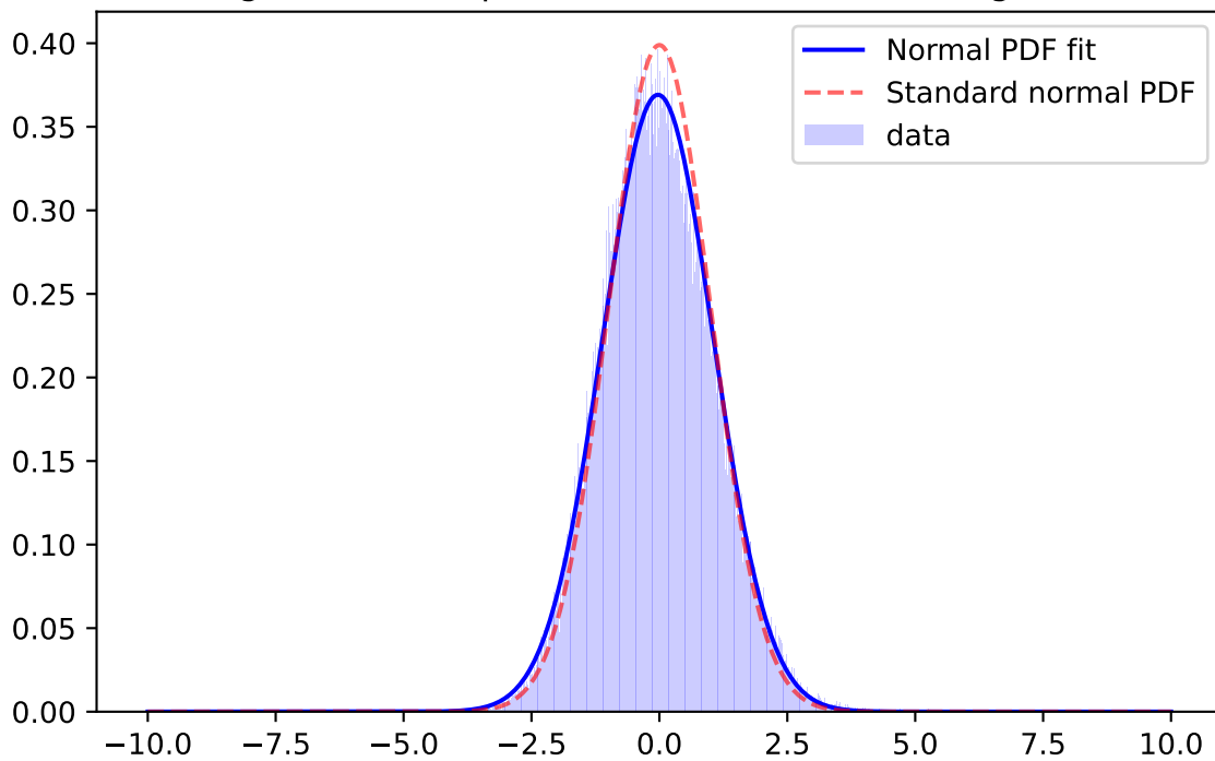
Whiten Signal, r-band, \mu=-0.0067 \sigma=1.0476 ; for mag=[25.0; 25.5]
