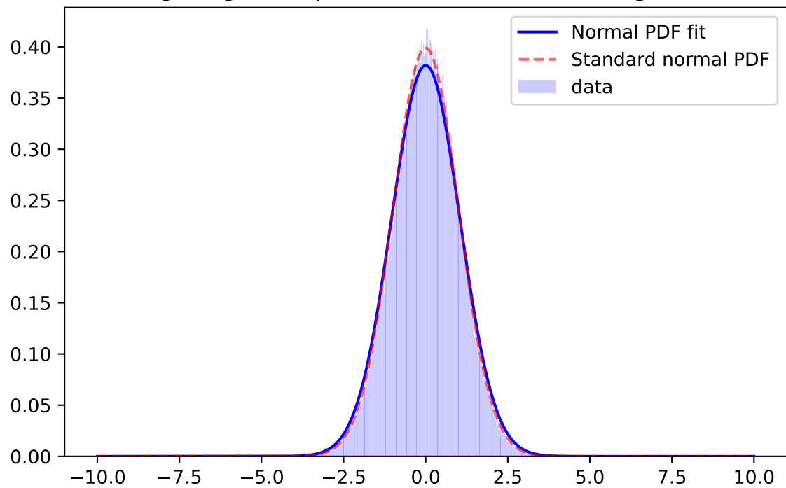
Whiten Signal, i-band, \mu=-0.0048 \sigma=0.9846 ; for mag=[25.0; 25.5]
