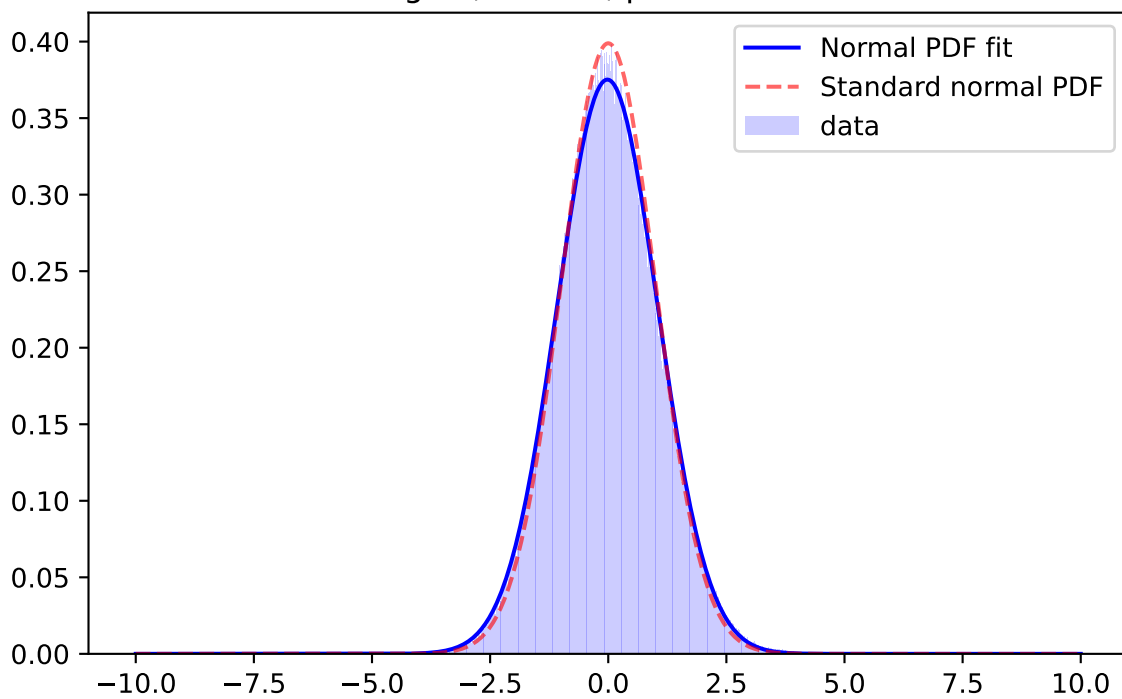
Whiten Signal, r-band, \mu=0.0143 \sigma=1.0423
