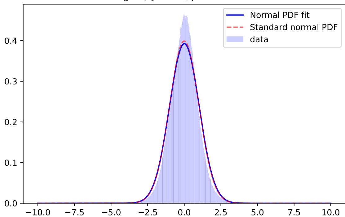
Whiten Signal, y-band, \mu=0.0052 \sigma=1.0163
