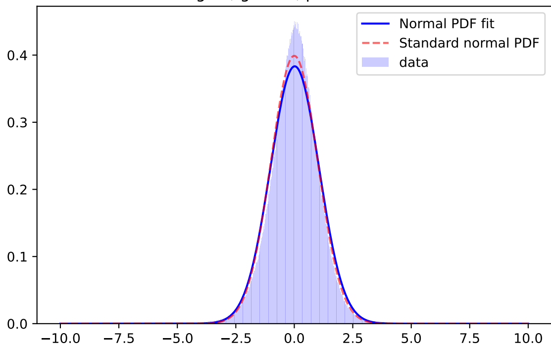
Whiten Signal, i-band, \mu=-0.0010 \sigma=1.0466
