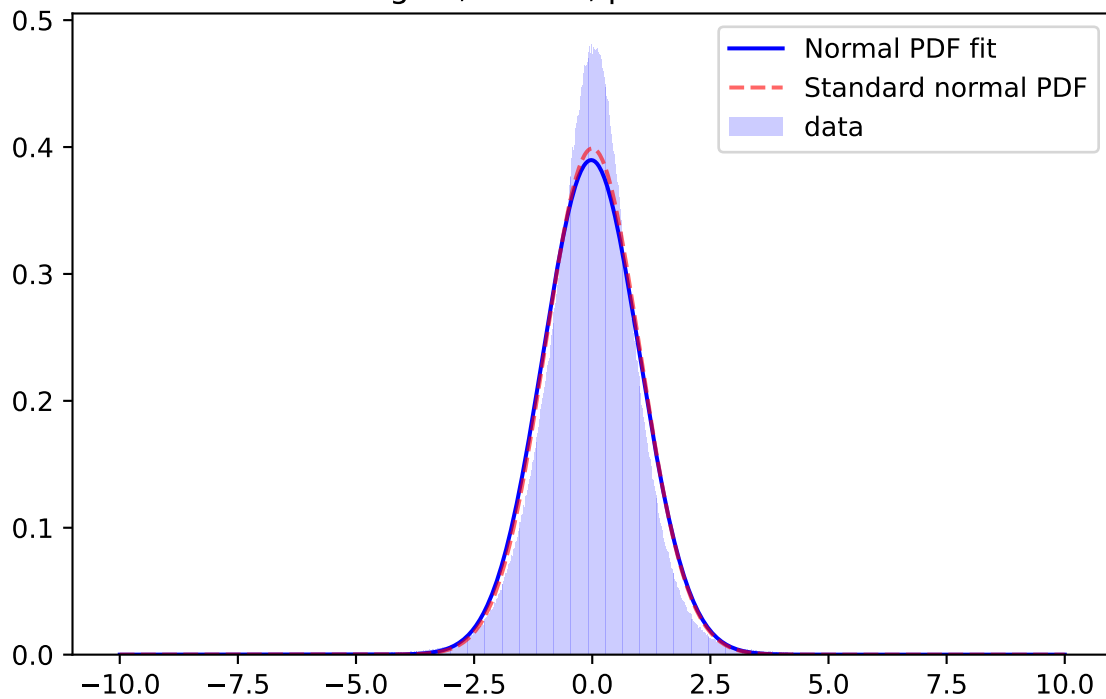
Whiten Signal, z-band, \mu=-0.0216 \sigma=1.0236
