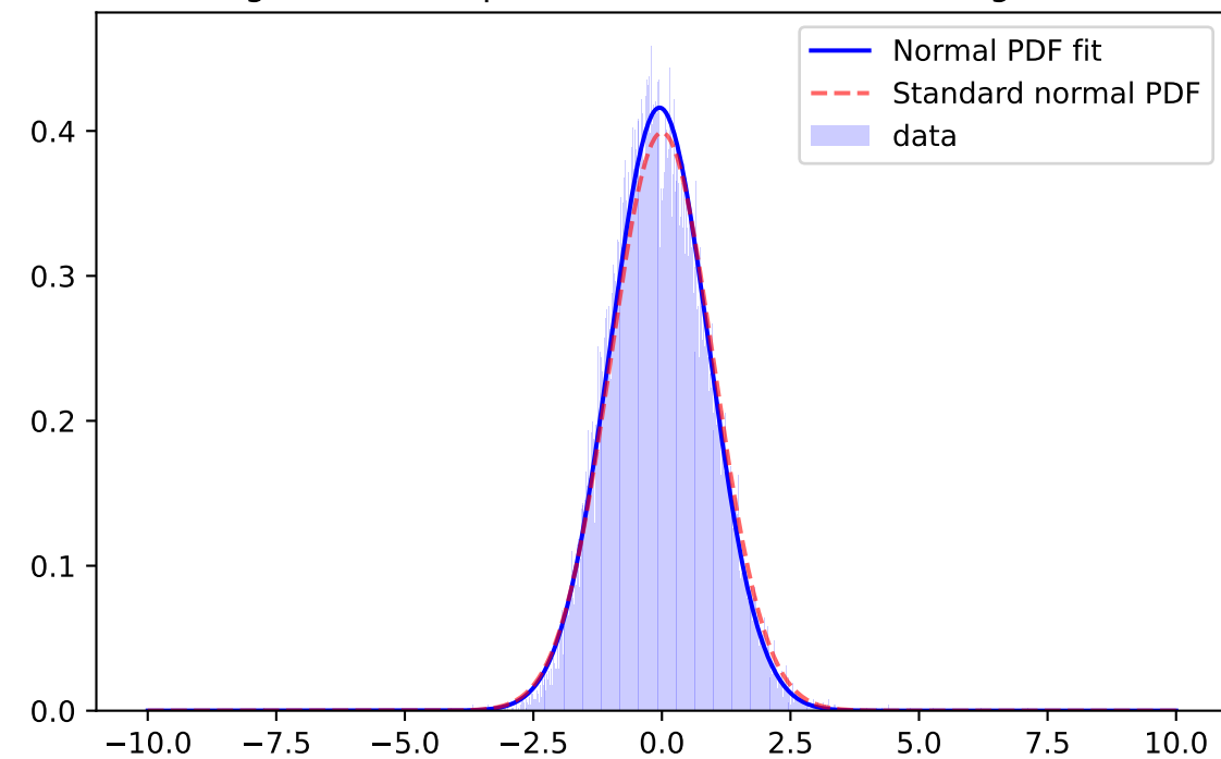
Whiten Signal, z-band, \mu=-0.0454 \sigma=0.9587 ; for mag=[25.0; 25.5]
