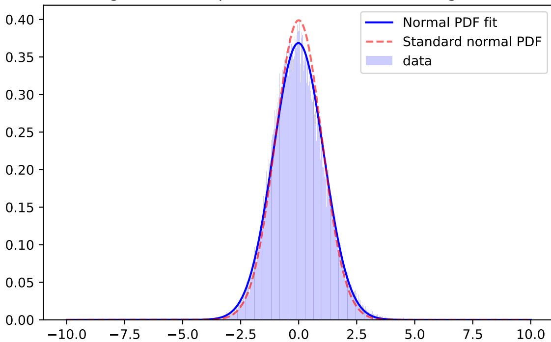
Whiten Signal, r-band, \mu=-0.0012 \sigma=1.0602 ; for mag=[25.0; 25.5]
