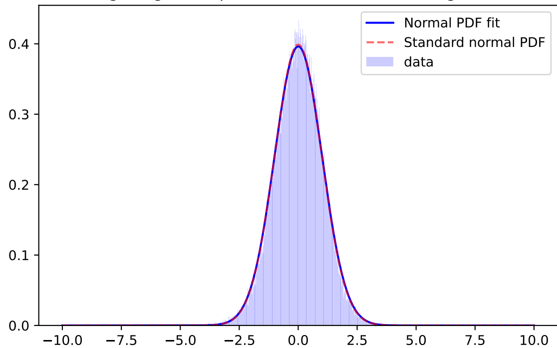
Whiten Signal, i-band, \mu=-0.0133 \sigma=0.9774 ; for mag=[25.0; 25.5]
