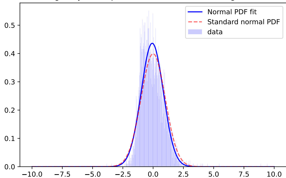
Whiten Signal, y-band, \mu=-0.0722 \sigma=0.9148 ; for mag=[25.0; 25.5]
