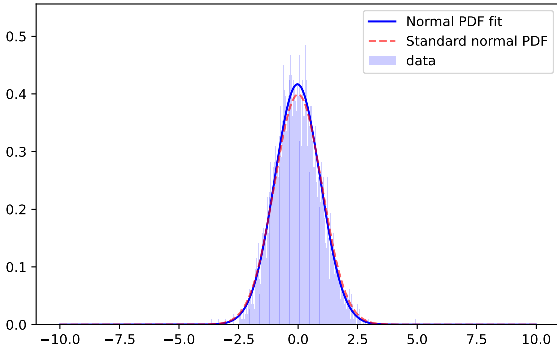
Whiten Signal, z-band, \mu=-0.0252 \sigma=0.9573 ; for mag=[25.0; 25.5]
