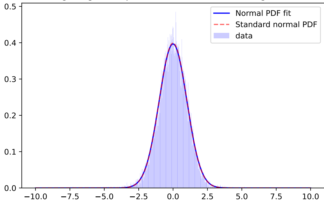
Whiten Signal, i-band, \mu=-0.0154 \sigma=0.9855 ; for mag=[25.0; 25.5]
