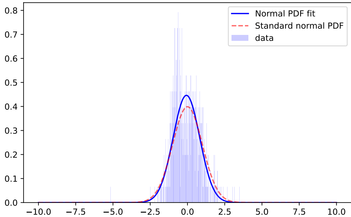
Whiten Signal, y-band, \mu=-0.0701 \sigma=0.8939 ; for mag=[25.0; 25.5]
