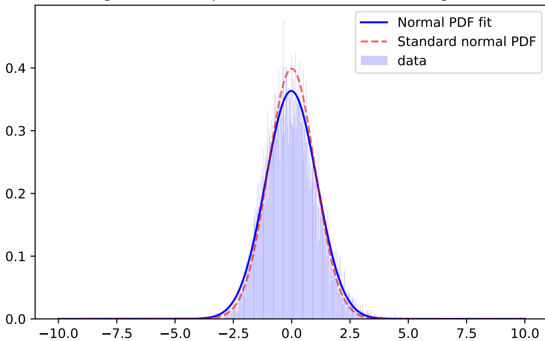
Whiten Signal, r-band, \mu=-0.0027 \sigma=1.0466 ; for mag=[25.0; 25.5]
