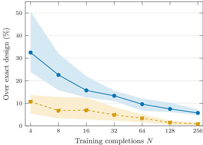
(b) True-risk regret
