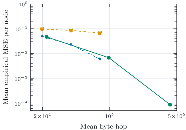
(b) Accuracy versus communication
