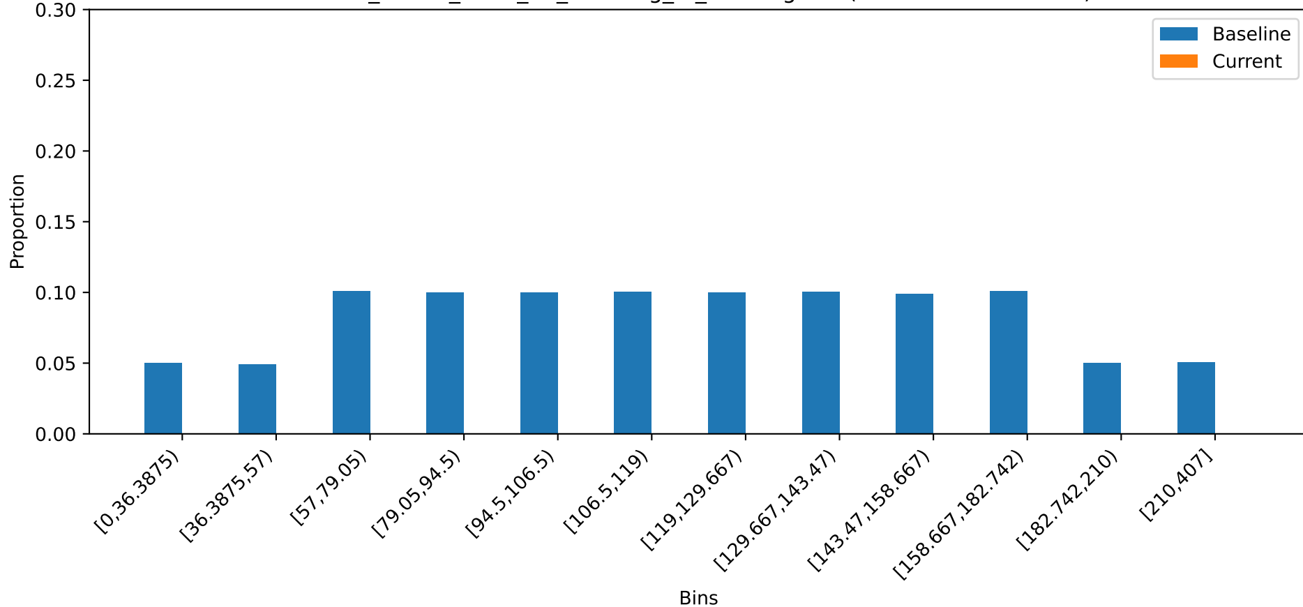
credit_model_2024_06_01 - avg_fe_9 histogram (Baseline vs 2024-09)
