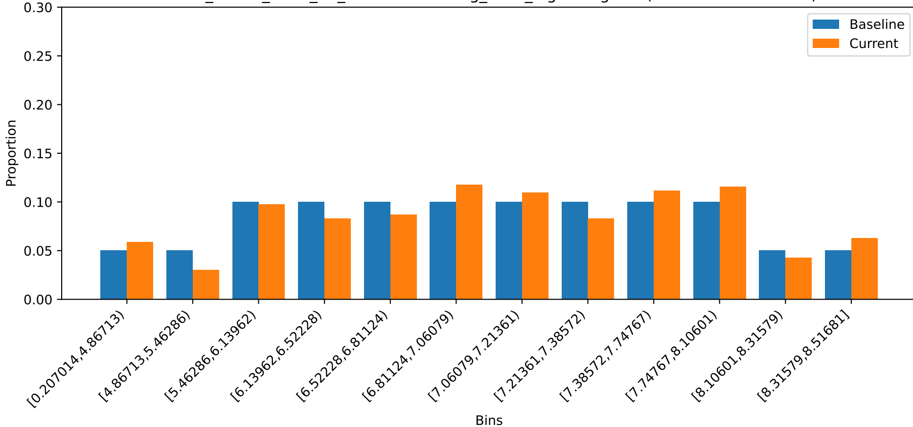
credit_model_2024_06_01 - Outstanding_Debt_log histogram (Baseline vs 2024-09)
