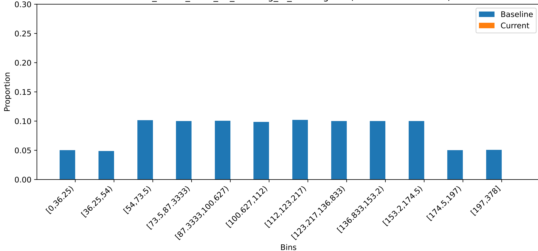
credit_model_2024_06_01 - avg_fe_5 histogram (Baseline vs 2024-09)
