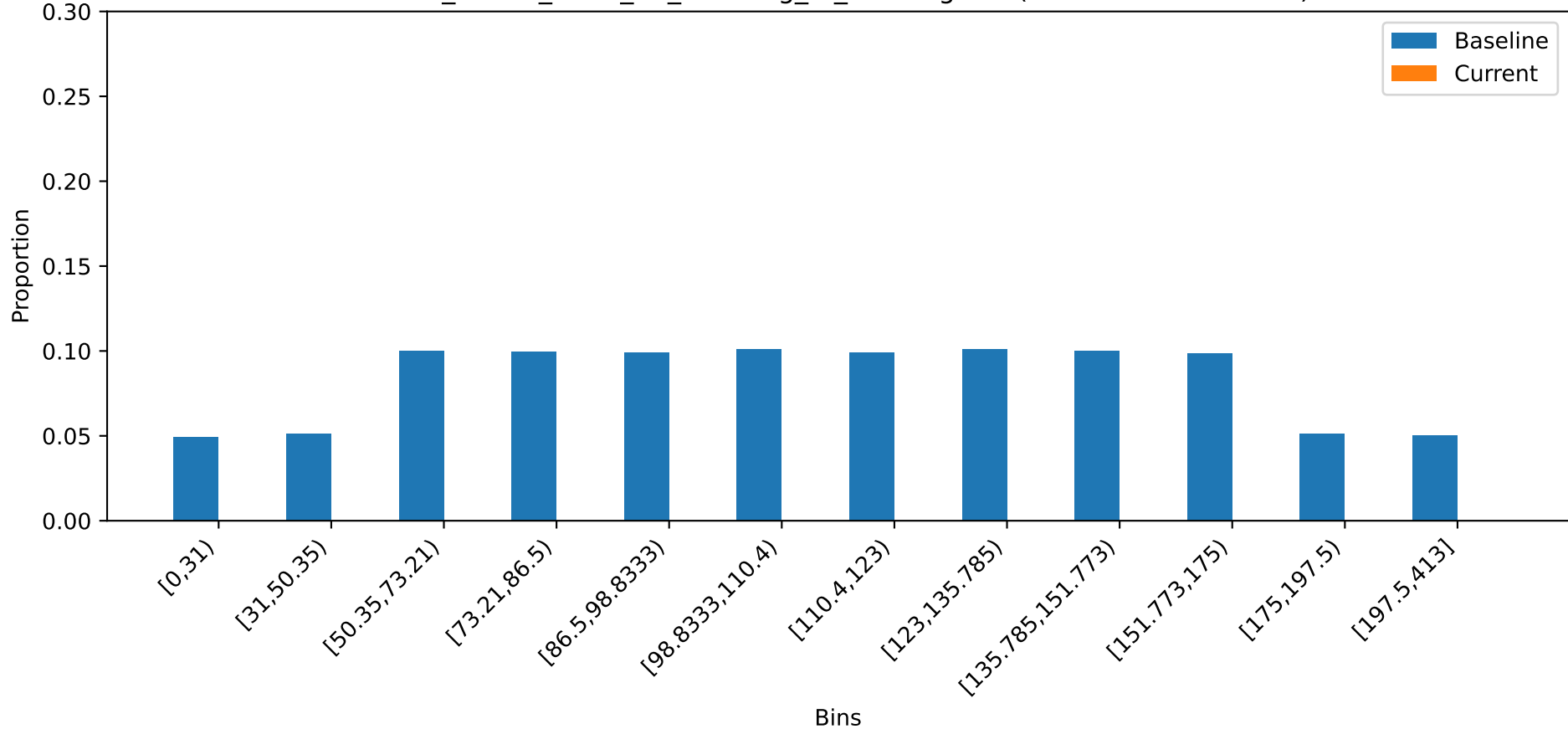
credit_model_2024_06_01 - avg_fe_4 histogram (Baseline vs 2024-09)
