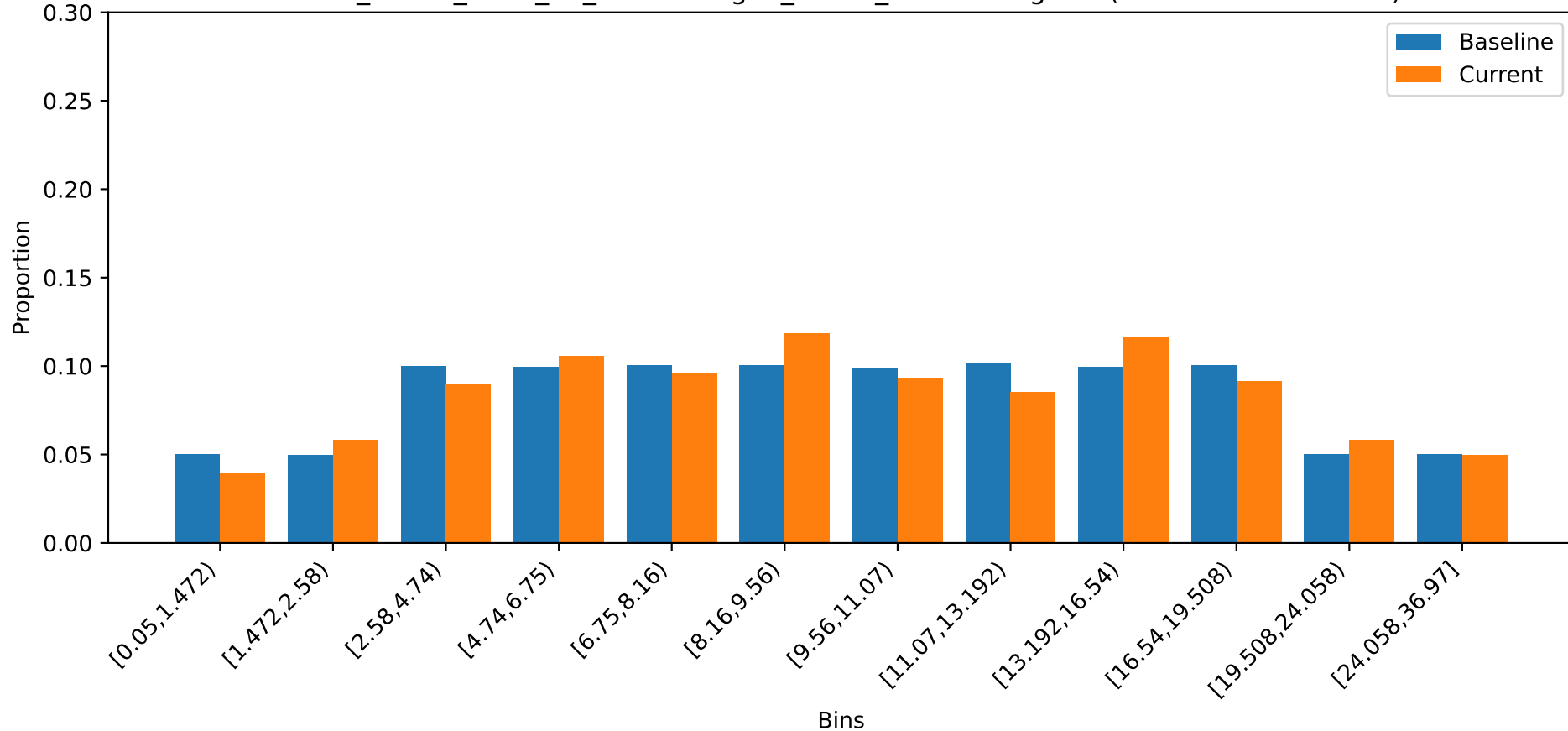
credit_model_2024_06_01 - Changed_Credit_Limit histogram (Baseline vs 2024-09)
