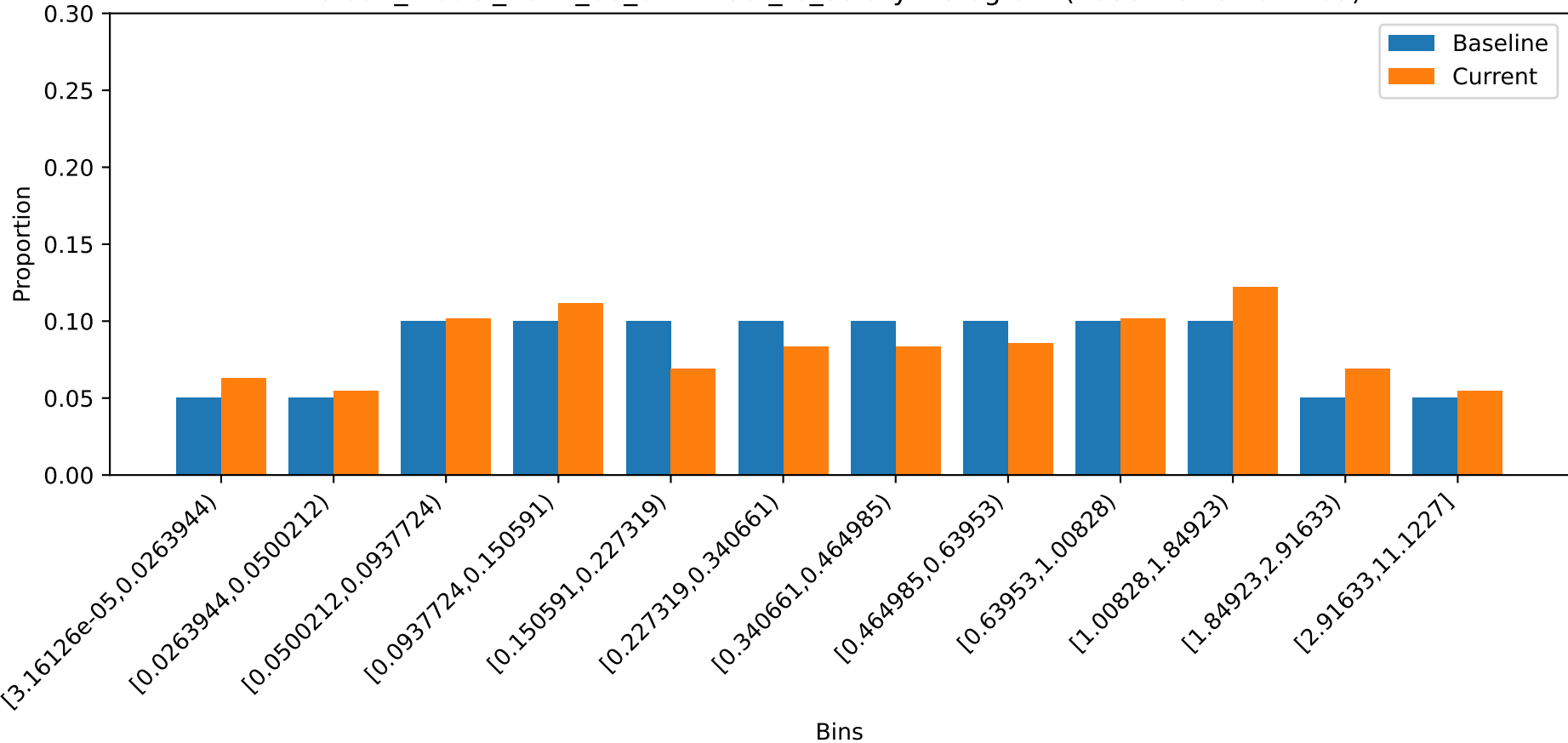
credit_model_2024_06_01 - Debt_to_Salary histogram (Baseline vs 2024-09)
