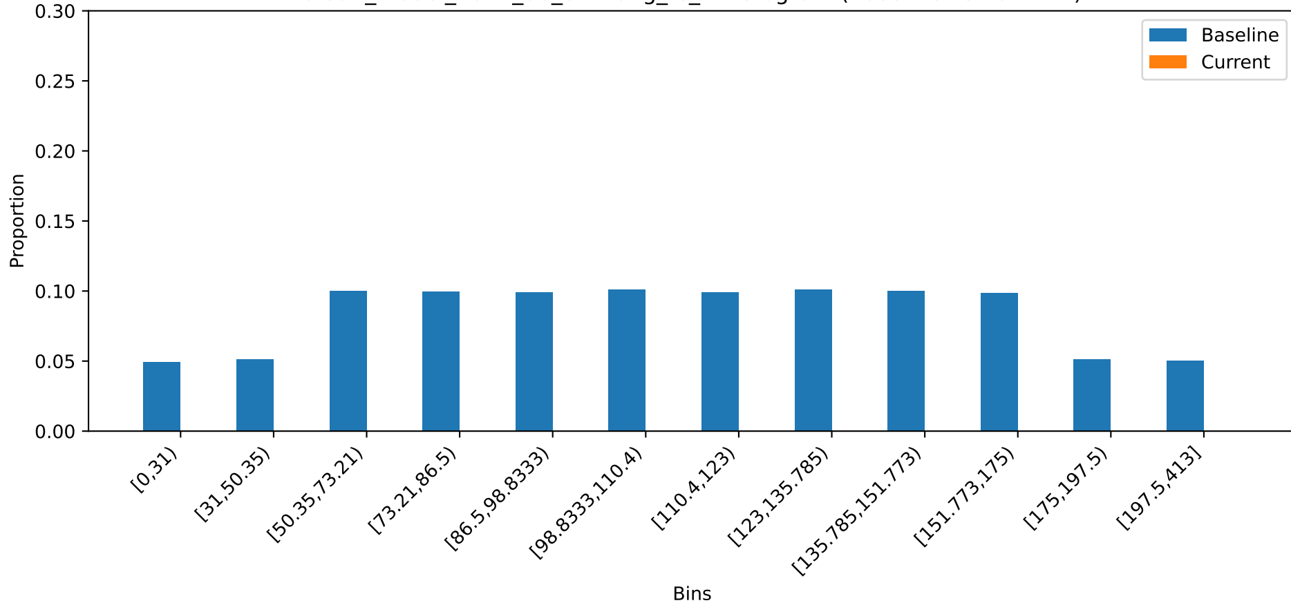
credit_model_2024_06_01 - avg_fe_4 histogram (Baseline vs 2024-12)
