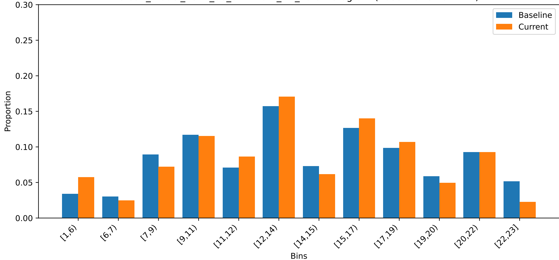
credit_model_2024_06_01 - Num_Fin_Pdts histogram (Baseline vs 2024-12)
