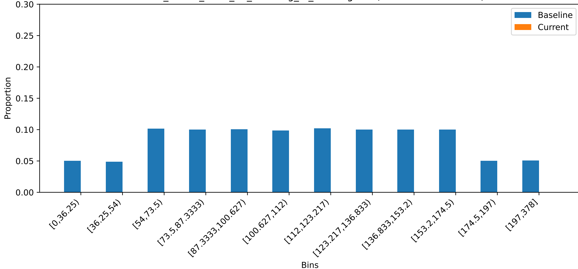
credit_model_2024_06_01 - avg_fe_5 histogram (Baseline vs 2024-12)
