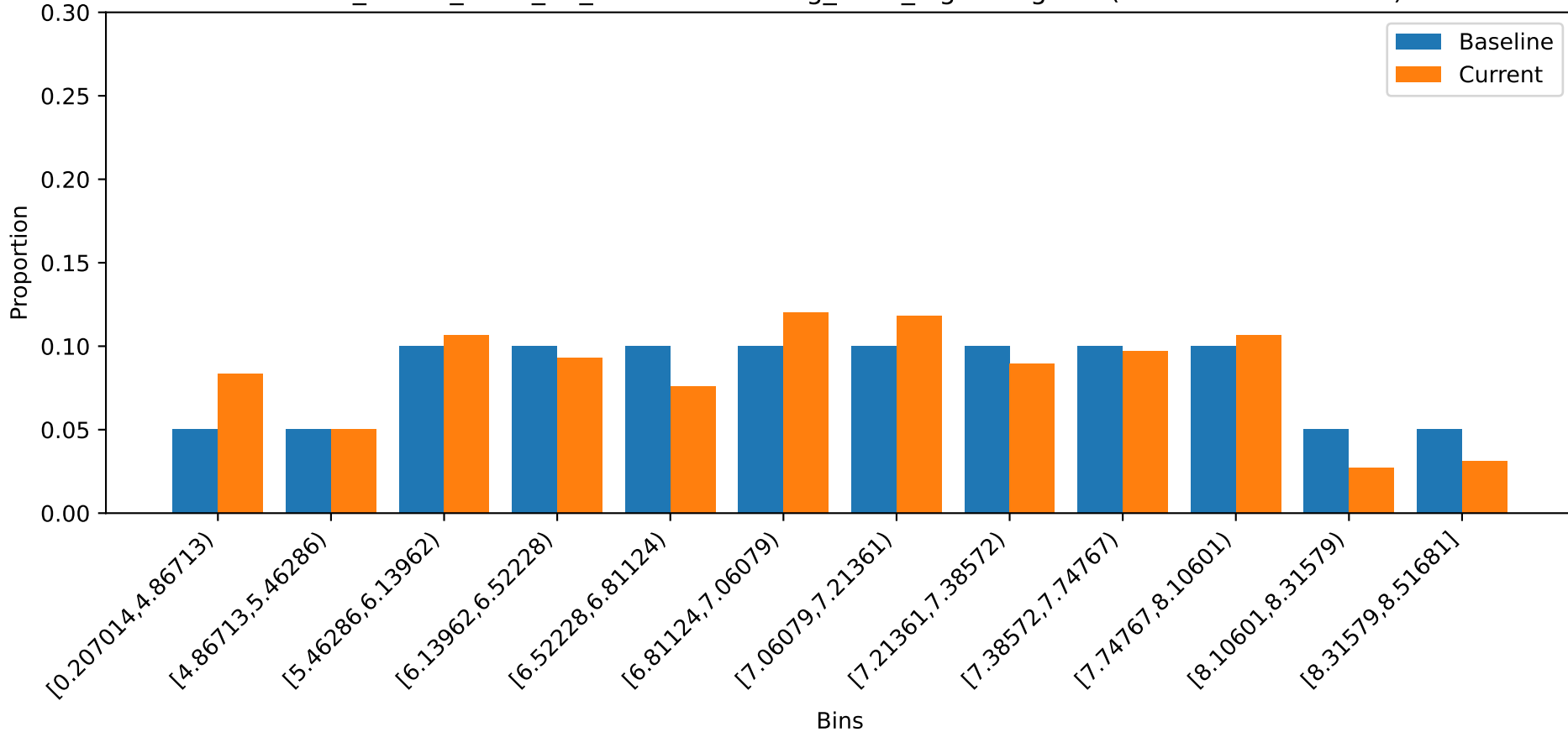
credit_model_2024_06_01 - Outstanding_Debt_log histogram (Baseline vs 2024-12)
