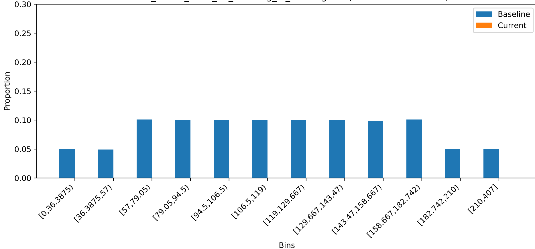
credit_model_2024_06_01 - avg_fe_9 histogram (Baseline vs 2024-12)
