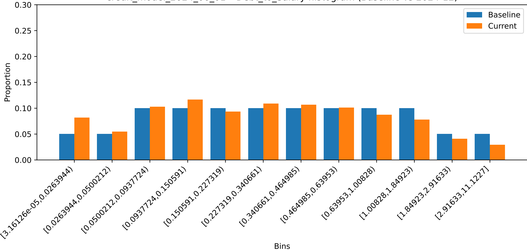
credit_model_2024_06_01 - Debt_to_Salary histogram (Baseline vs 2024-12)
