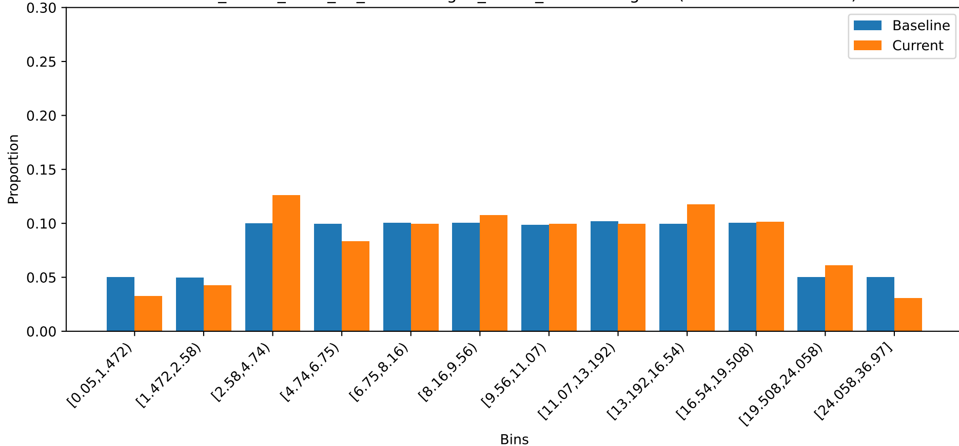
credit_model_2024_06_01 - Changed_Credit_Limit histogram (Baseline vs 2024-12)
