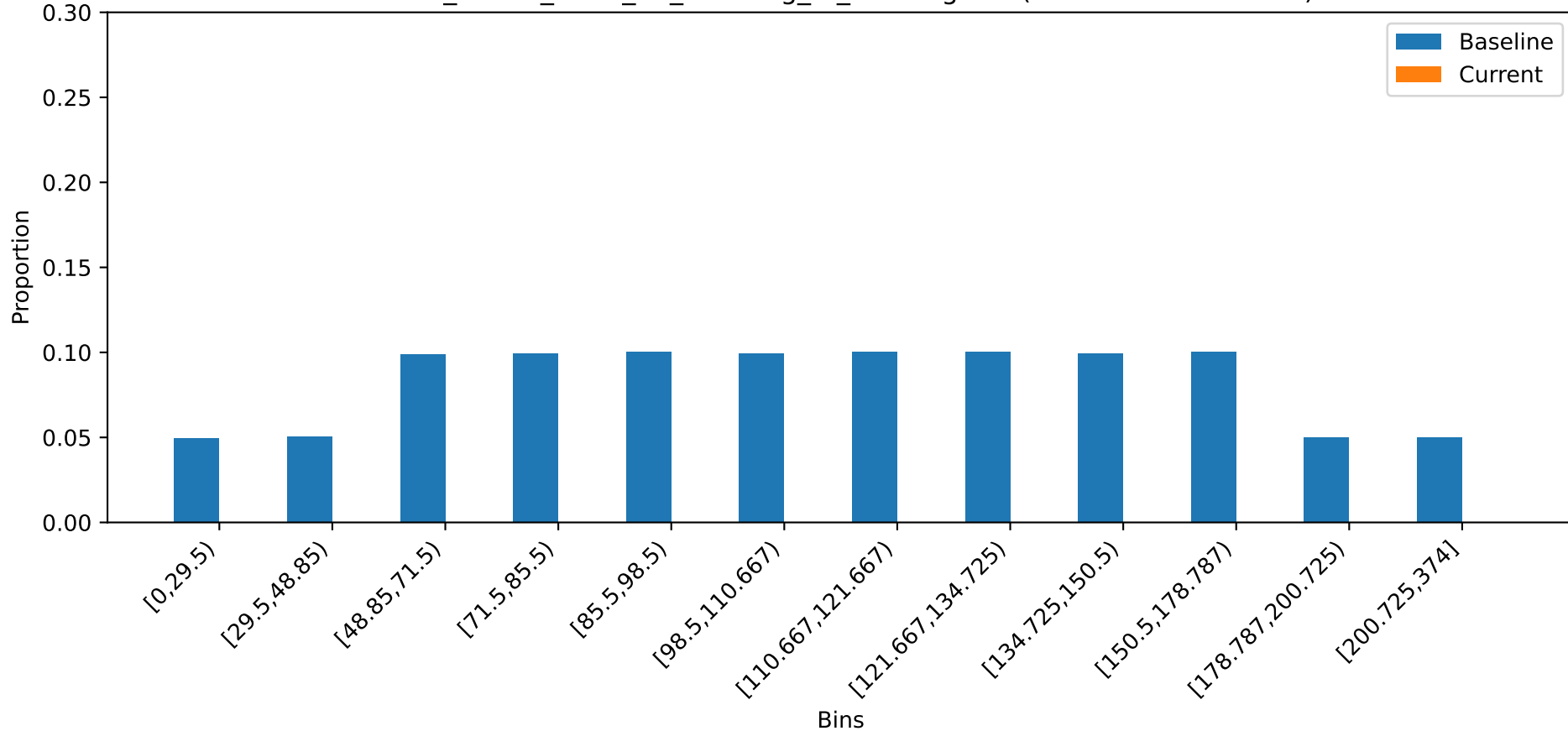
credit_model_2024_06_01 - avg_fe_3 histogram (Baseline vs 2024-12)
