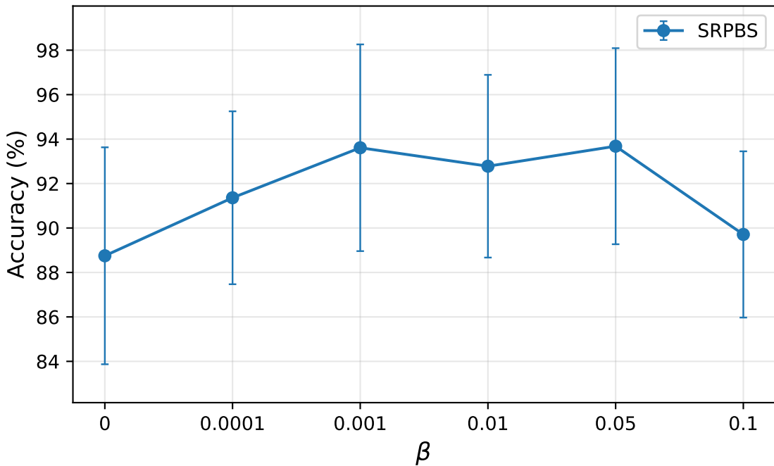
Sensitivity to MI Loss Weight ( \beta ) — SRPBS
