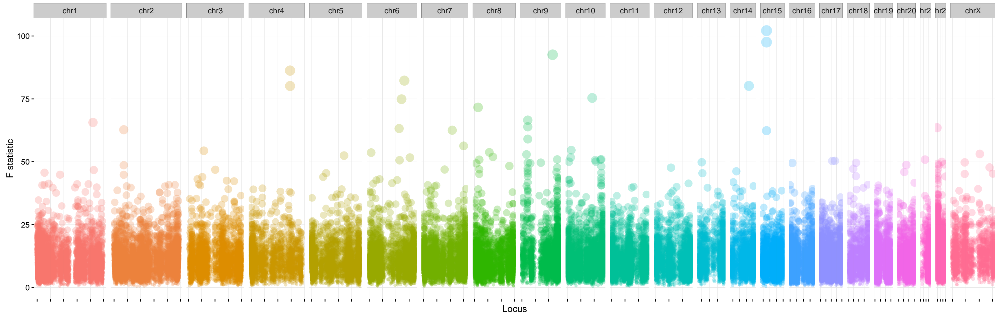
F statistic for each locus, sorted by chromosome
