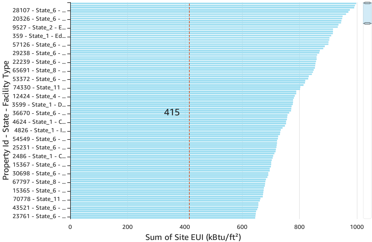
Top 1,000 Buildings by Site EUI
