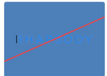
Low-contrast background
